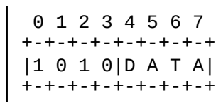
Figure 10.6h: IVAS Bit Rate request
