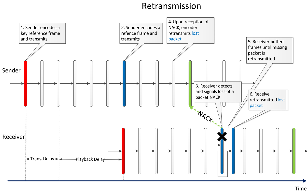
Figure P.4: Video error recovery using NACK feedback message and retransmission.
