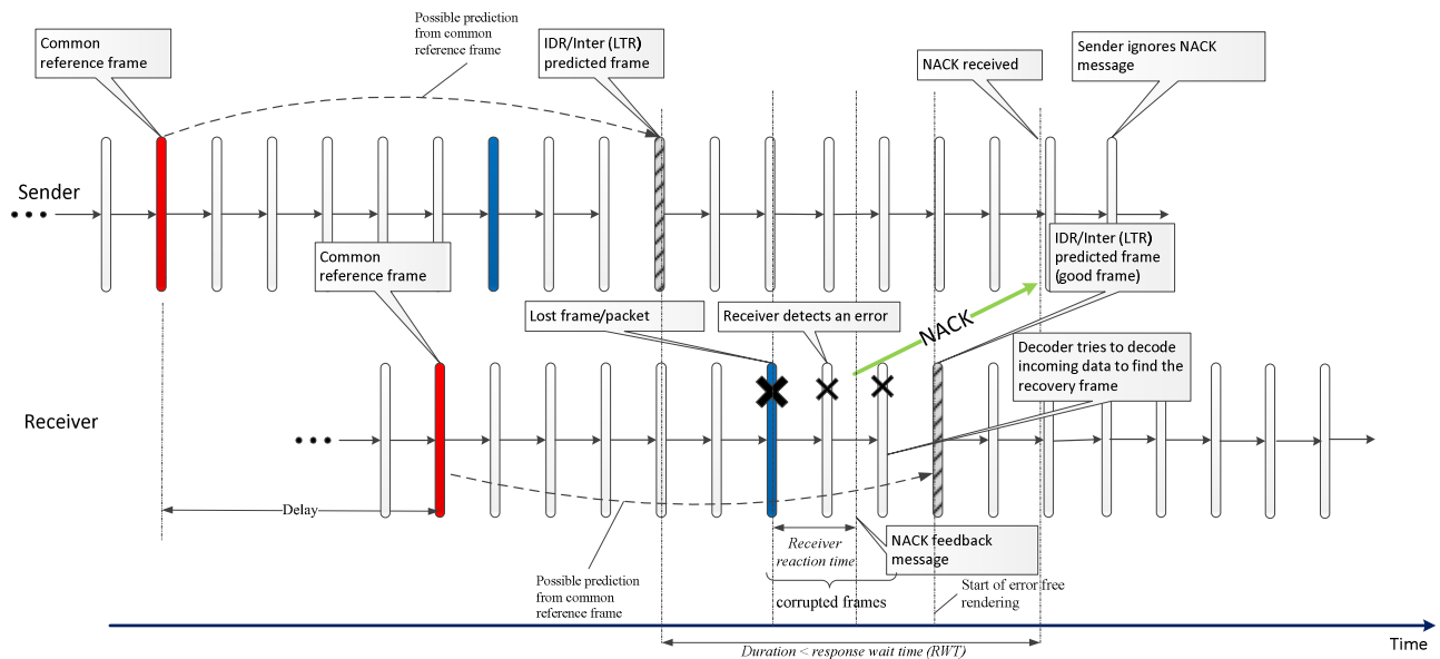
Figure P.3: Example case where sender does not have to respond to incoming NACK/PLI messages.
