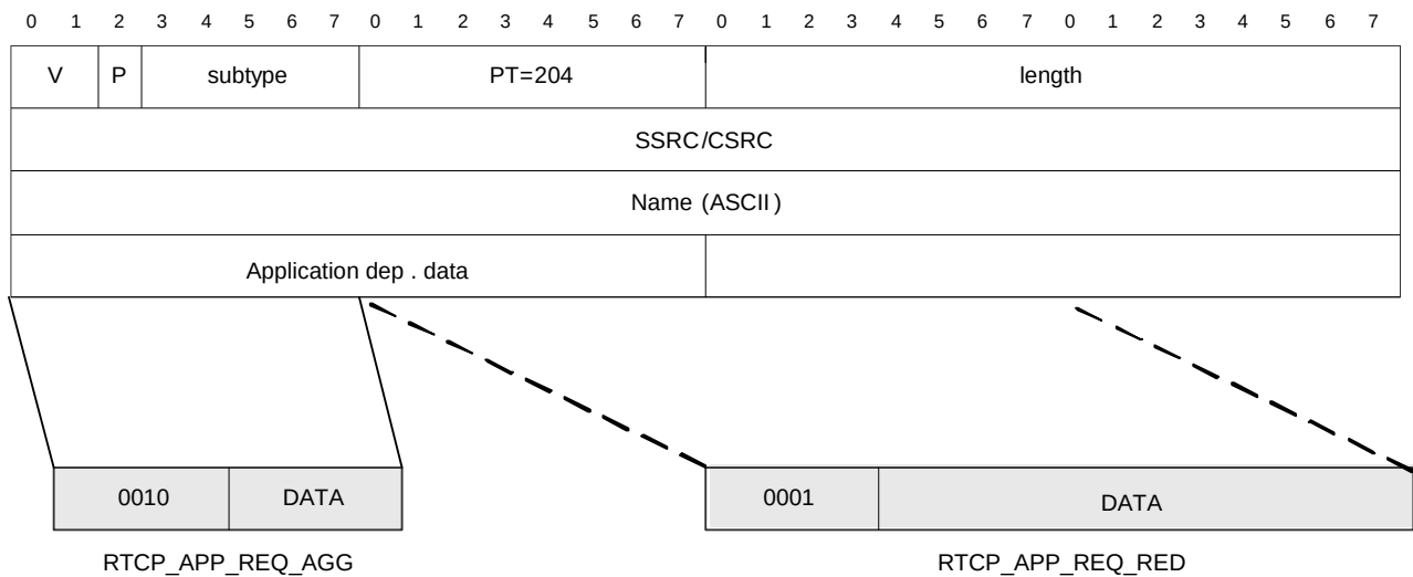
Figure 10.1: RTCP-APP formatting
