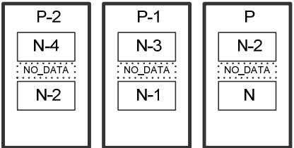
Figure 10.10: Payload packetization with 100 % redundancy and an extra offset of one packet
