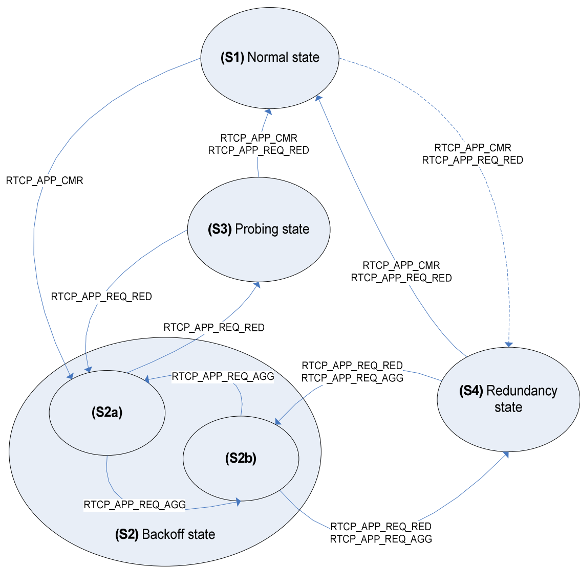
Figure C.2: State diagram for four-state adaptation state machine
