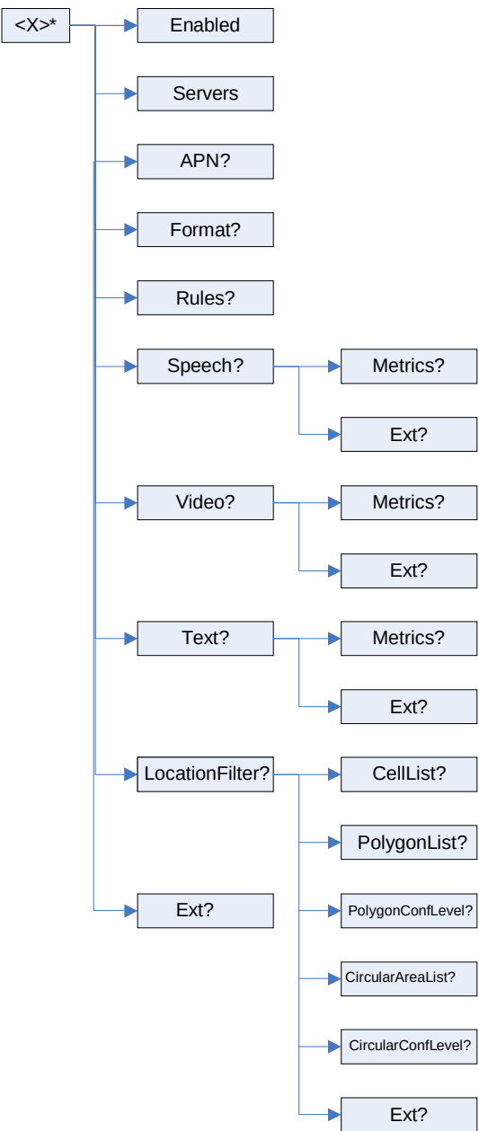
Figure 16.1: MTSI QoE metrics management object tree
