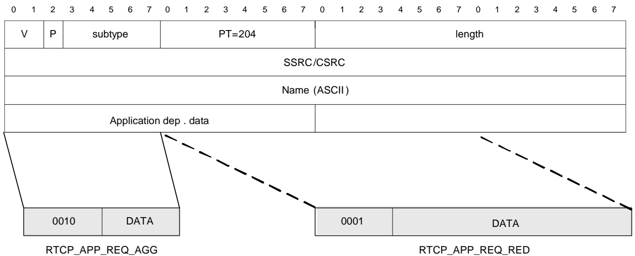
Figure 10.1: RTCP-APP formatting
