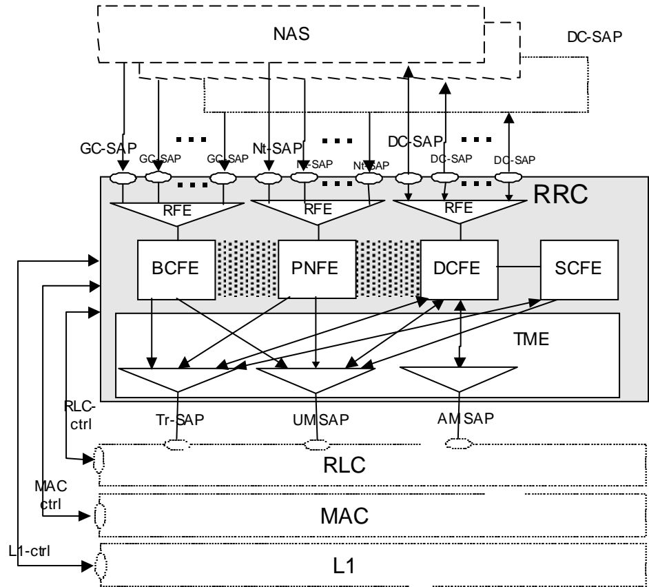
Figure 4.2-3: UTRAN side RRC model (DS-41 System)
