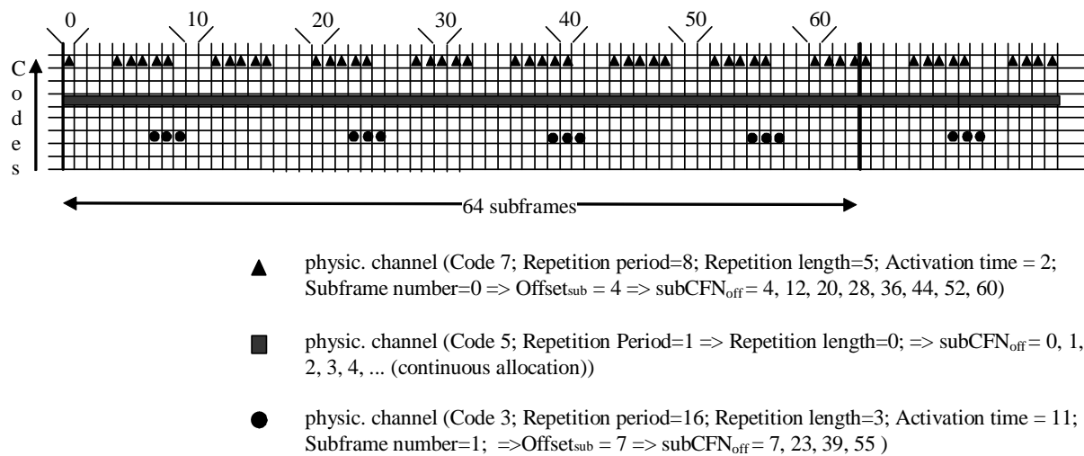
Figure 8.6.16a-1: Examples for subframe allocations in TDD
