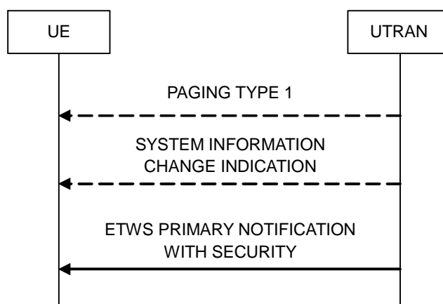
Figure 8.1.17-1: ETWS primary notification with security
