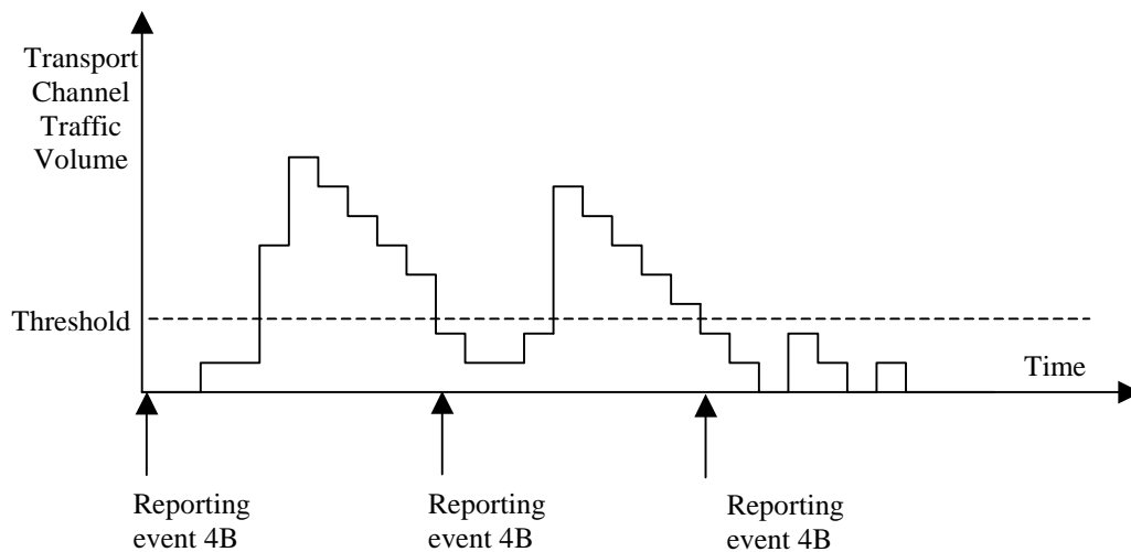
Figure 14.4.2-2: Event triggered report when Transport Channel Traffic Volume becomes smaller than certain threshold
