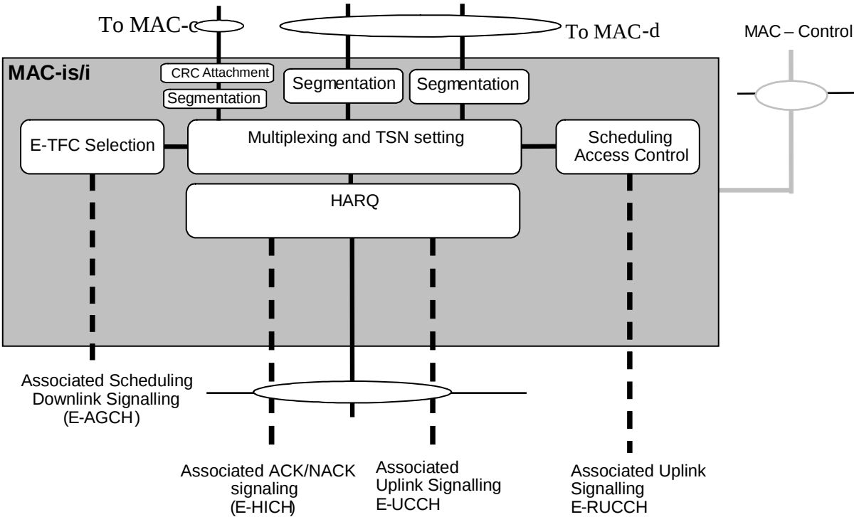
Figure 4.2.3.6-2: UE side MAC architecture / MAC-i/i details (TDD)
