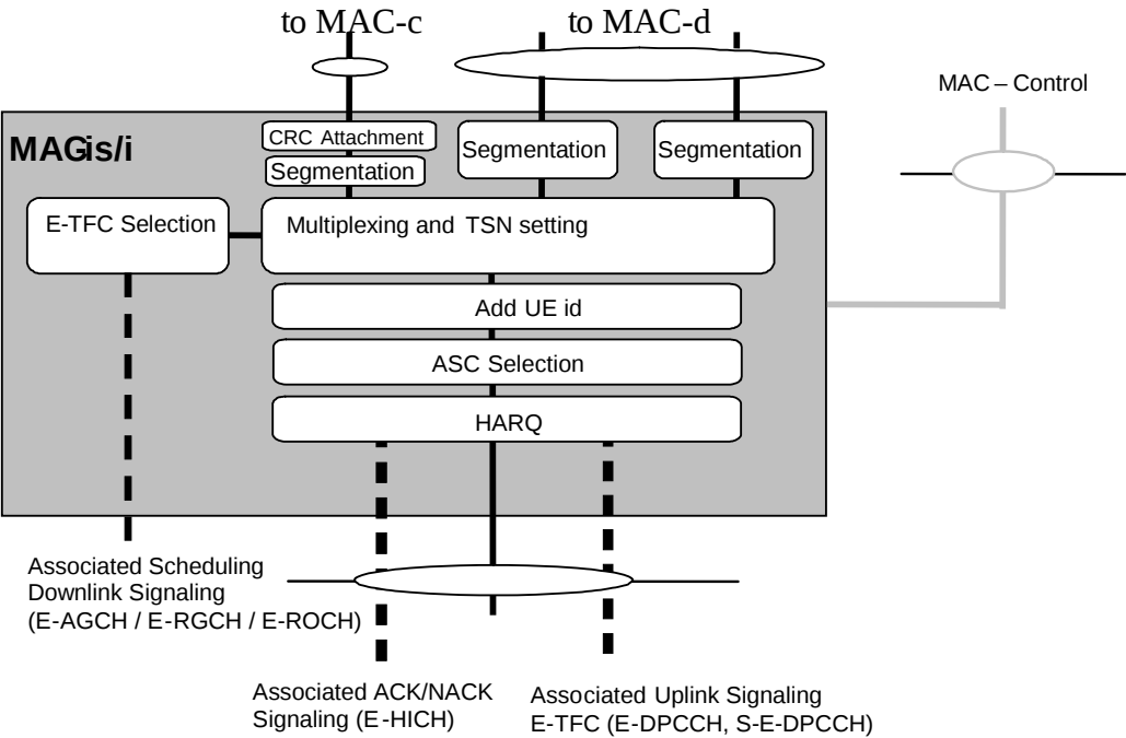
Figure 4.2.3.6-1a: UE side MAC architecture / MAC-i/i details (uplink MIMO is configured, FDD)
