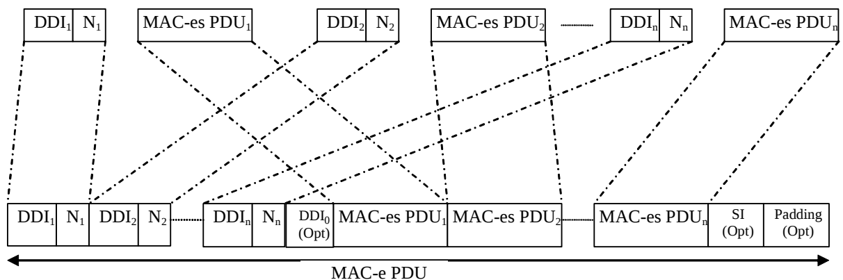
Figure 9.1.5-2a: MAC-e PDU
