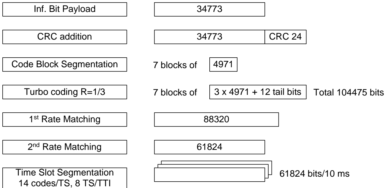
Figure [A.12] Coding for HS-PDSCH fixed reference channel with 16-QAM modulation for the VA120 Channel – Category 8
