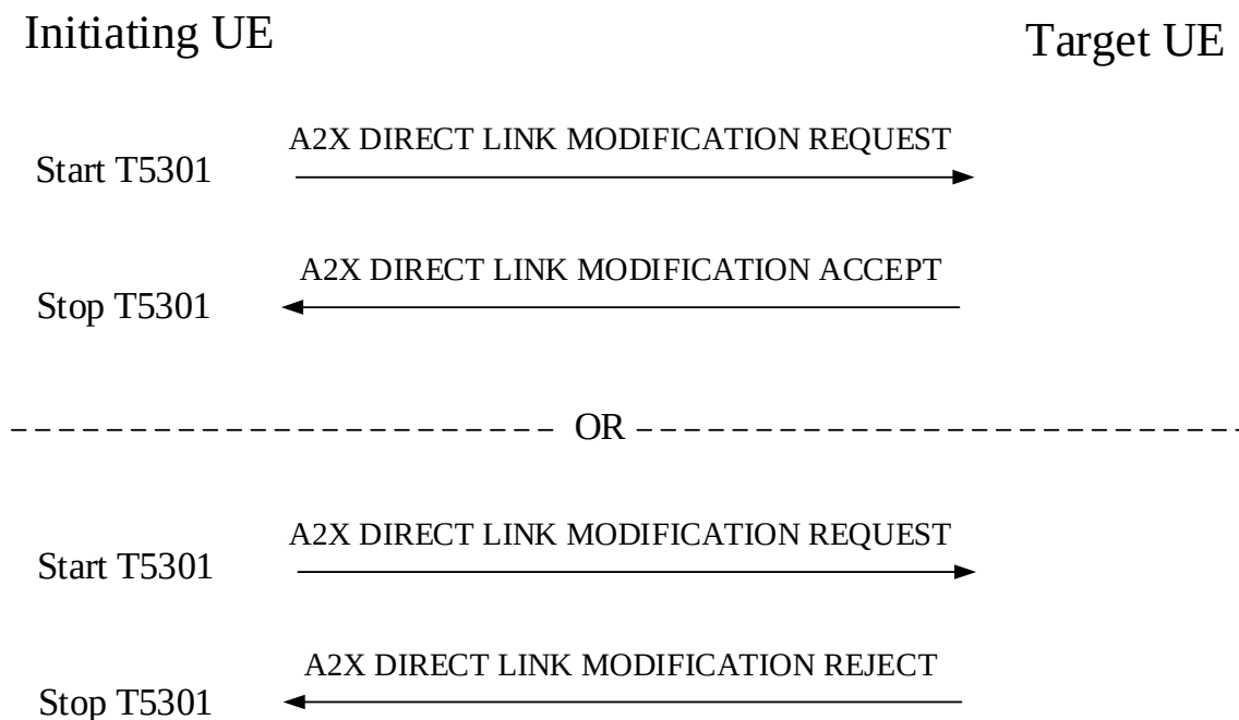
Figure 6.1.2.3.2: A2X PC5 unicast link modification procedure
