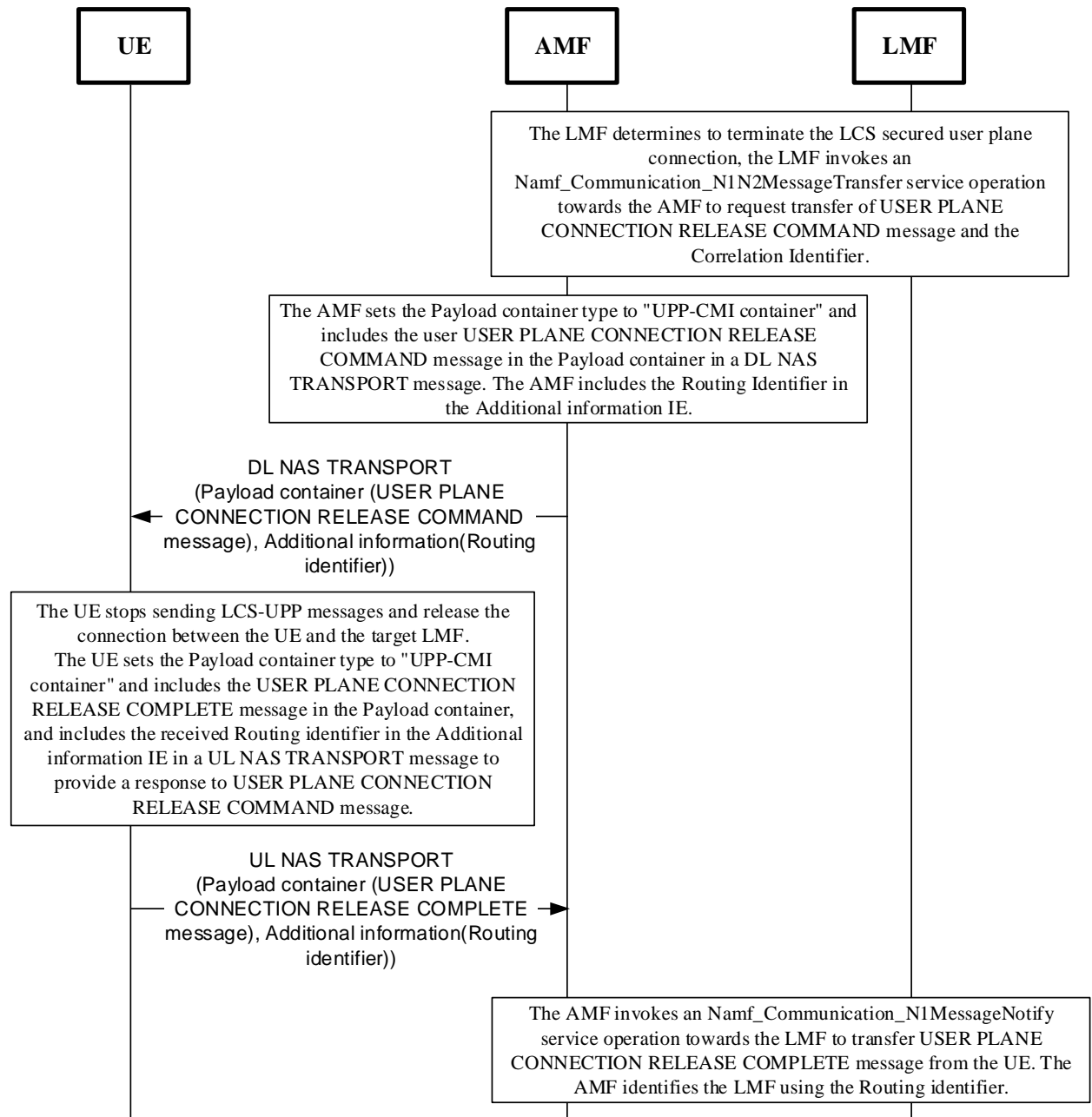
Figure 6.2.1.2.1.1: Signalling transport for network initiated user plane connection release procedure
