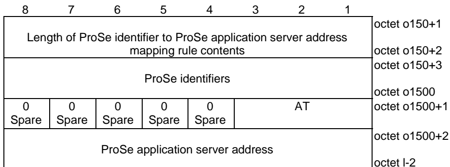
Figure 5.10.2.18: ProSe identifier to ProSe application server address mapping rule
