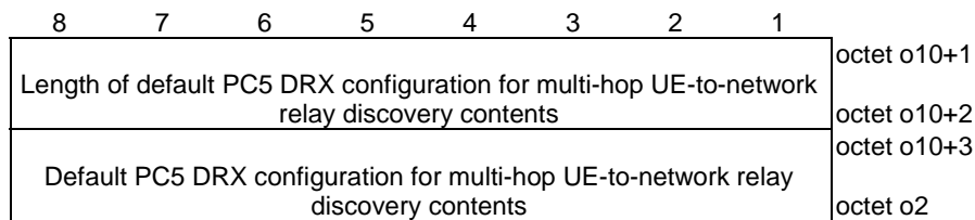
Figure 5.10.2.11a: Default PC5 DRX configuration for multi-hop UE-to-network relay discovery
