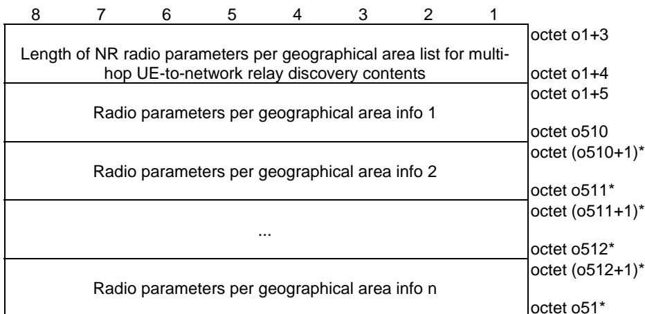
Figure 5.10.2.6: NR radio parameters per geographical area list for multi-hop UE-to-network relay discovery
