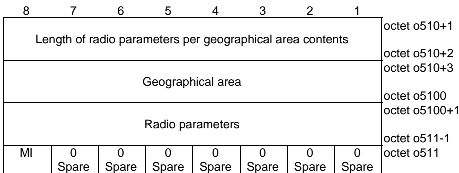
Figure 5.8.2.8: Radio parameters per geographical area info
