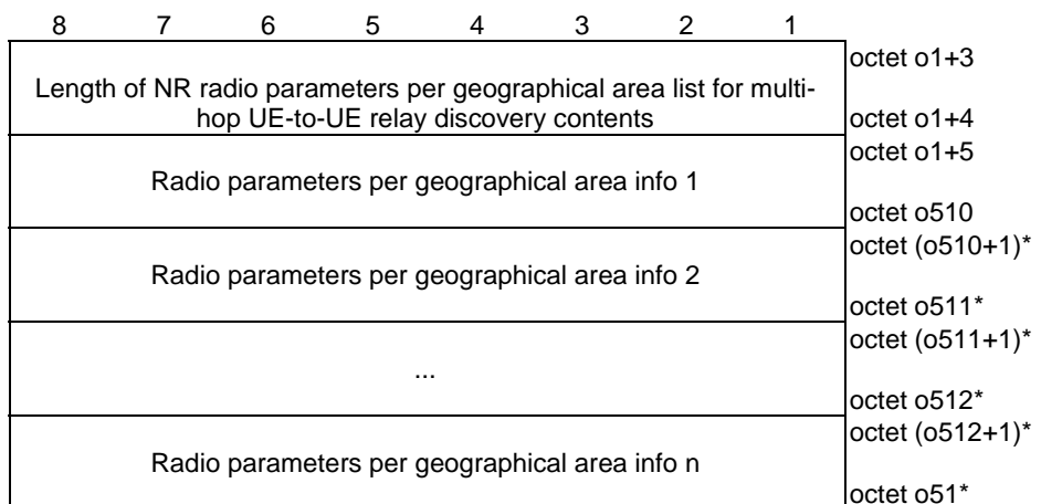
Figure 5.14.2.4: NR radio parameters per geographical area list for multi-hop UE-to-UE relay discovery
