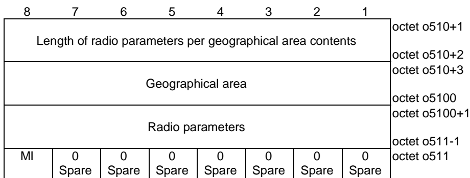
Figure 5.13.2.8: Radio parameters per geographical area info
