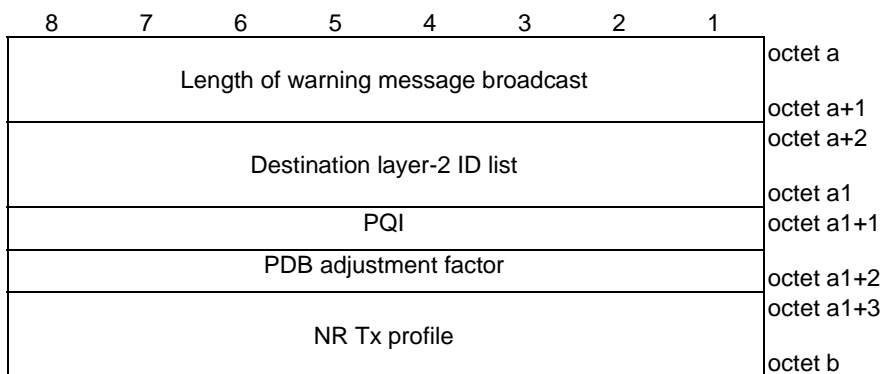
Figure 5.5.2.24: Warning message broadcast
