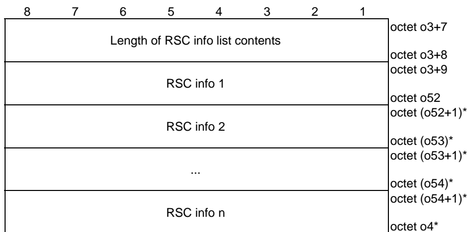
Figure 5.10.2.12: RSC info list
