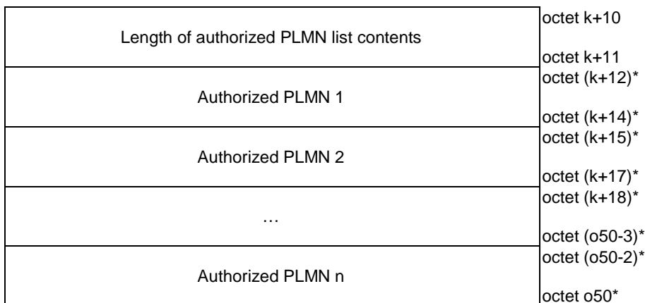
Figure 5.13.2.3: Authorized PLMN list
