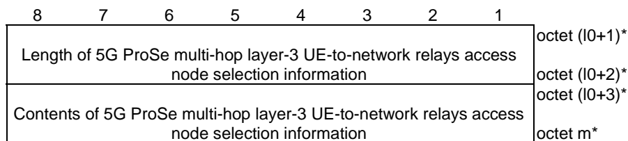
Figure 5.12.2.19: 5G ProSe multi-hop layer-3 UE-to-network relays access node selection information
