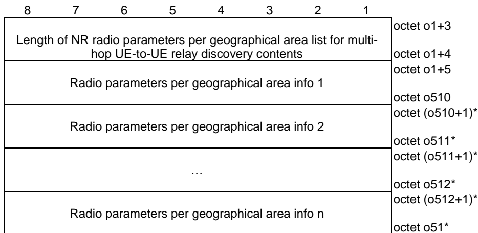
Figure 5.13.2.6: NR radio parameters per geographical area list for multi-hop UE-to-UE relay discovery
