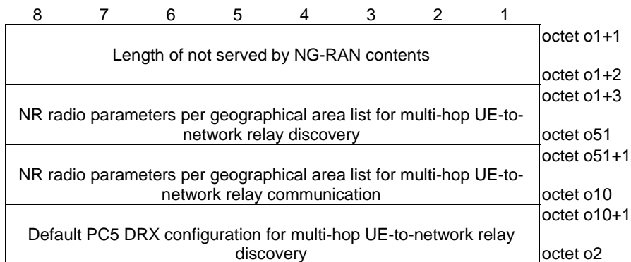
Figure 5.12.2.3: Not served by NG-RAN
