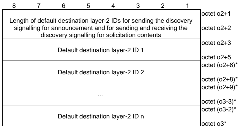
Figure 5.13.2.11b: Default destination layer-2 IDs for sending the discovery signalling for announcement and for sending and receiving the discovery signalling for solicitation
