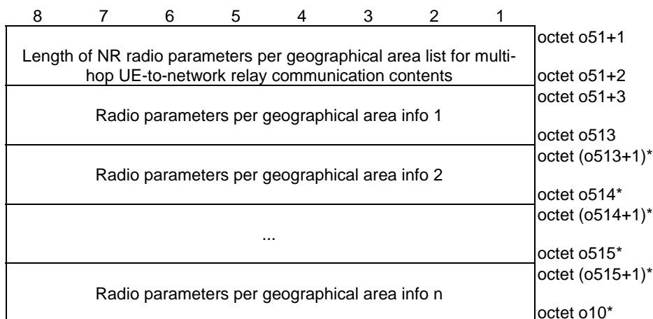
Figure 5.10.2.7: NR radio parameters per geographical area list for multi-hop UE-to-network relay communication
