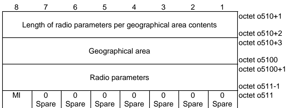
Figure 5.14.2.6: Radio parameters per geographical area info
