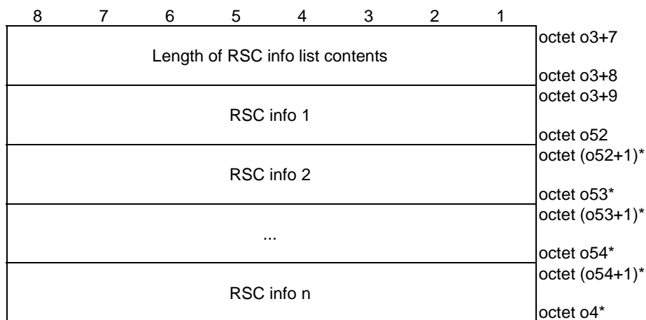
Figure 5.12.2.12: RSC info list
