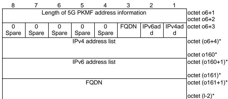
Figure 5.5.2.21: 5G PKMF address information
