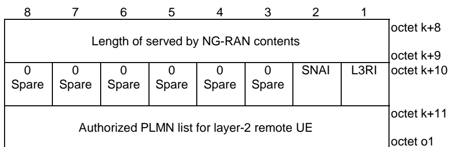
Figure 5.6.2.2: Served by NG-RAN
