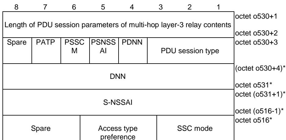
Figure 5.12.2.15: PDU session parameters of multi-hop layer-3 relay
