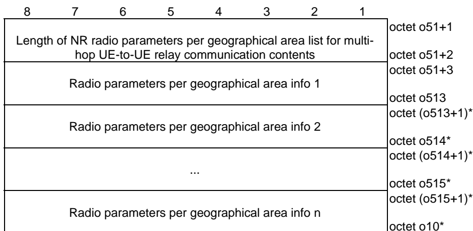
Figure 5.14.2.5: NR radio parameters per geographical area list for multi-hop UE-to-UE relay communication
