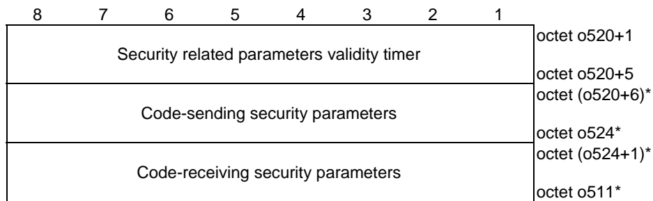
Figure 5.10.2.15: Security related parameters for multi-hop UE-to-network relay discovery
