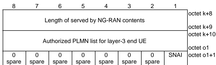
Figure 5.14.2.2: Served by NG-RAN
