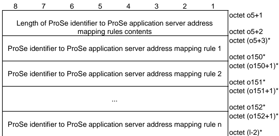
Figure 5.10.2.17: ProSe identifier to ProSe application server address mapping rules
