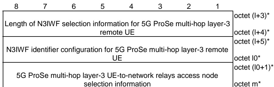
Figure 5.12.2.17: N3IWF selection information for 5G ProSe multi-hop layer-3 remote UE
