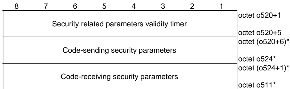
Figure 5.5.2.15: Security related parameters for UE-to-network relay discovery
