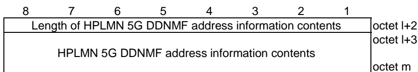
Figure 5.3.2.17: HPLMN 5G DDNMF address information
