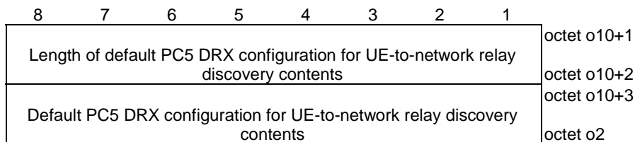
Figure 5.11.2.11: Default PC5 DRX configuration for UE-to-network relay discovery
