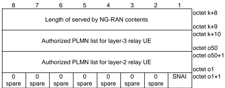
Figure 5.8.2.2: Served by NG-RAN
