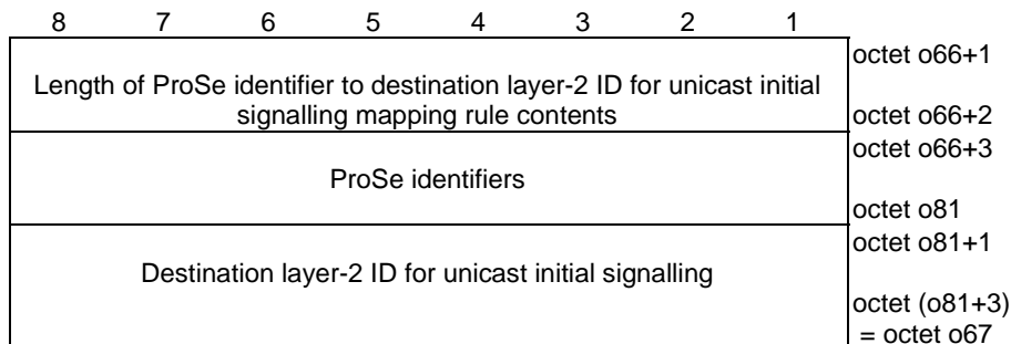
Figure 5.4.2.27: ProSe identifier to destination layer-2 ID for unicast initial signalling mapping rule
