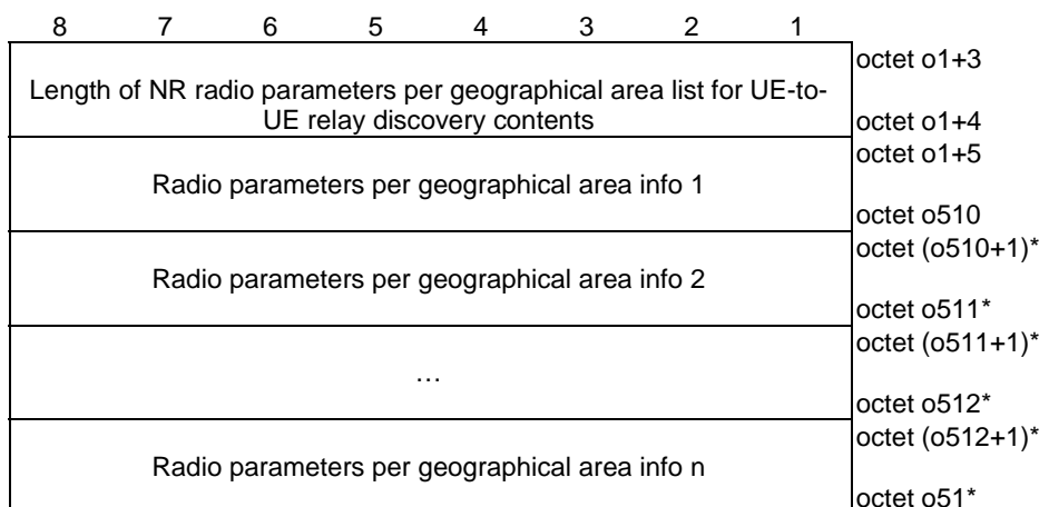
Figure 5.8.2.6: NR radio parameters per geographical area list for UE-to-UE relay discovery
