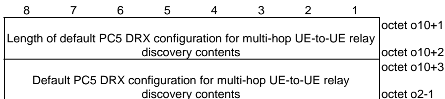
Figure 5.14.2.9a: Default PC5 DRX configuration for multi-hop UE-to-UE relay discovery
