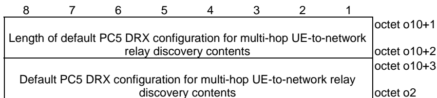
Figure 5.12.2.10: Default PC5 DRX configuration for multi-hop UE-to-network relay discovery
