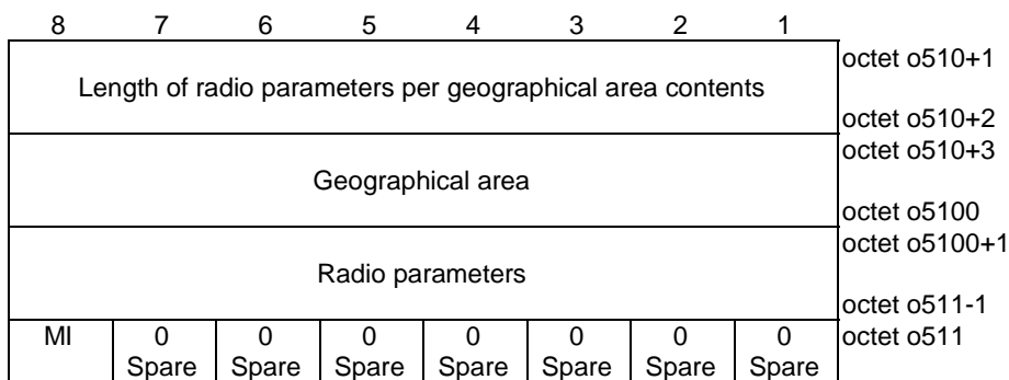
Figure 5.10.2.8: Radio parameters per geographical area info
