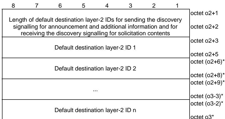
Figure 5.10.2.11b: Default destination layer-2 IDs for sending the discovery signalling for announcement and additional information and for receiving the discovery signalling for solicitation
