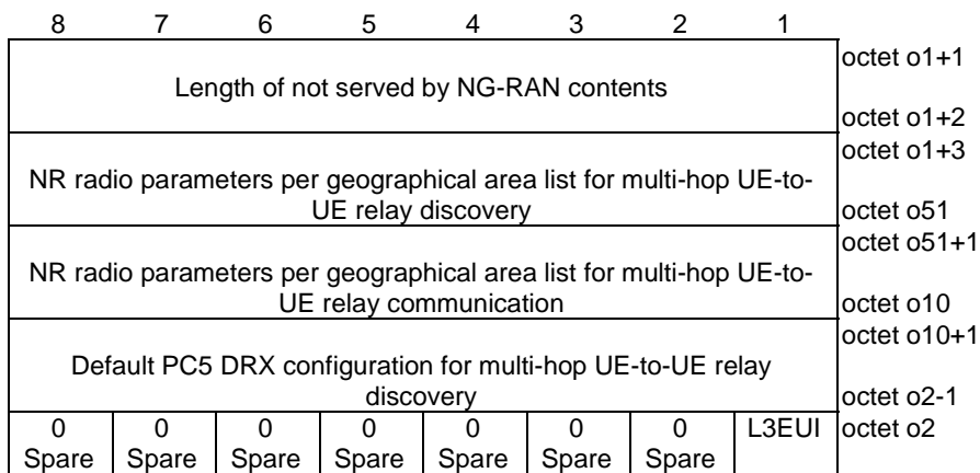
Figure 5.14.2.3: Not served by NG-RAN
