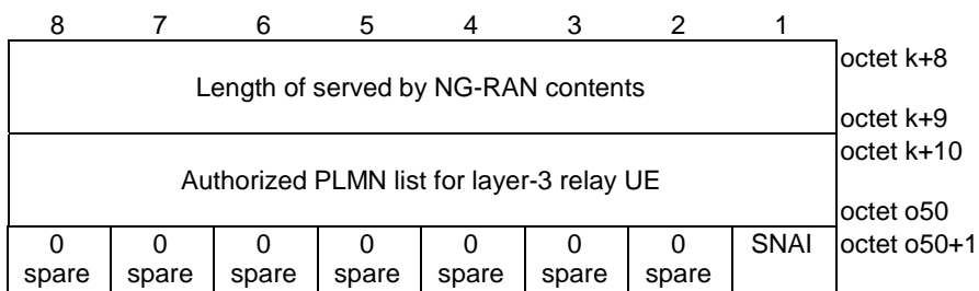
Figure 5.13.2.2: Served by NG-RAN
