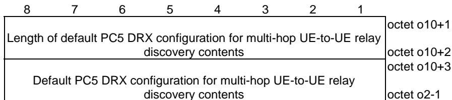
Figure 5.13.2.11a: Default PC5 DRX configuration for multi-hop UE-to-UE relay discovery
