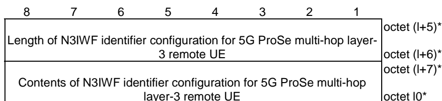
Figure 5.12.2.18: N3IWF identifier configuration for 5G ProSe multi-hop layer-3 remote UE
