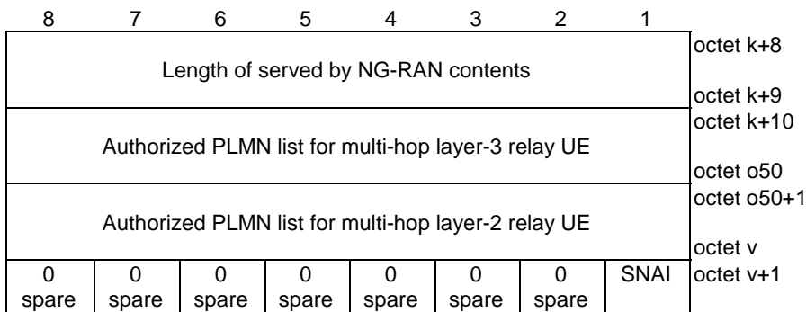
Figure 5.10.2.2: Served by NG-RAN
