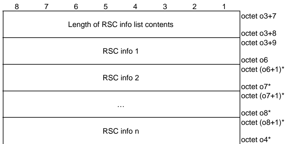
Figure 5.13.2.12: RSC info list
