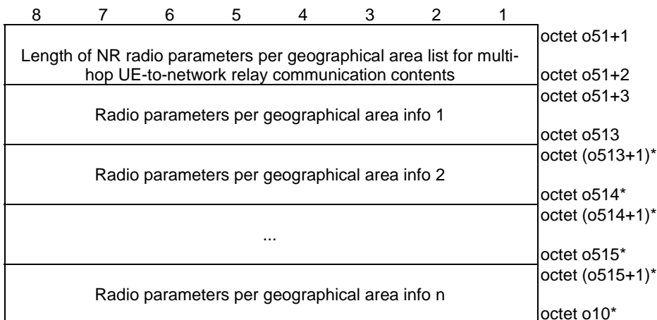
Figure 5.12.2.5: NR radio parameters per geographical area list for multi-hop UE-to-network relay communication
