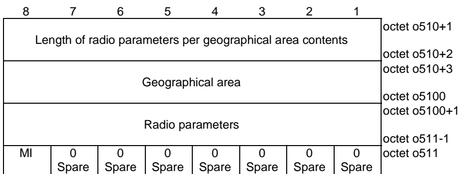
Figure 5.12.2.6: Radio parameters per geographical area info
