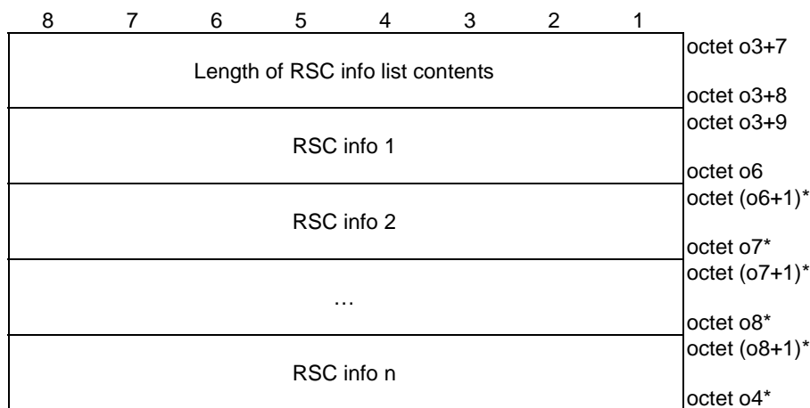
Figure 5.14.2.10: RSC info list
