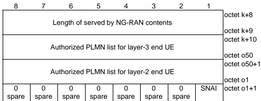
Figure 5.9.2.2: Served by NG-RAN
