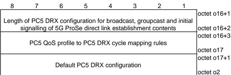
Figure 5.4.2.10a: PC5 DRX configuration for broadcast, groupcast and initial signalling of 5G ProSe direct link establishment
