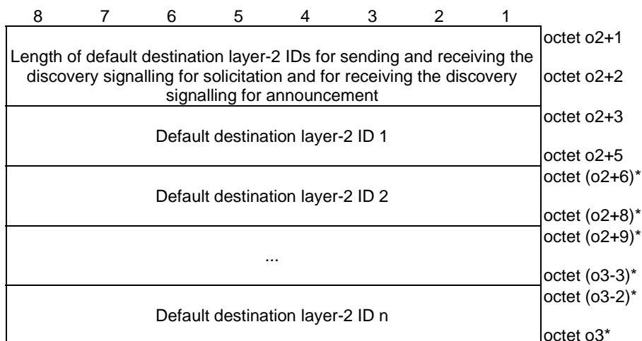
Figure 5.14.2.9b: Default destination layer-2 IDs for sending and receiving the discovery signalling for solicitation and for receiving the discovery signalling for announcement
