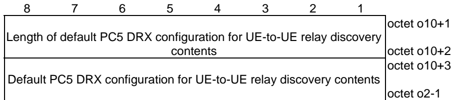
Figure 5.8.2.11a: Default PC5 DRX configuration for UE-to-UE relay discovery
