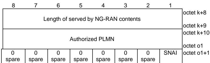
Figure 5.4.2.2: Served by NG-RAN
