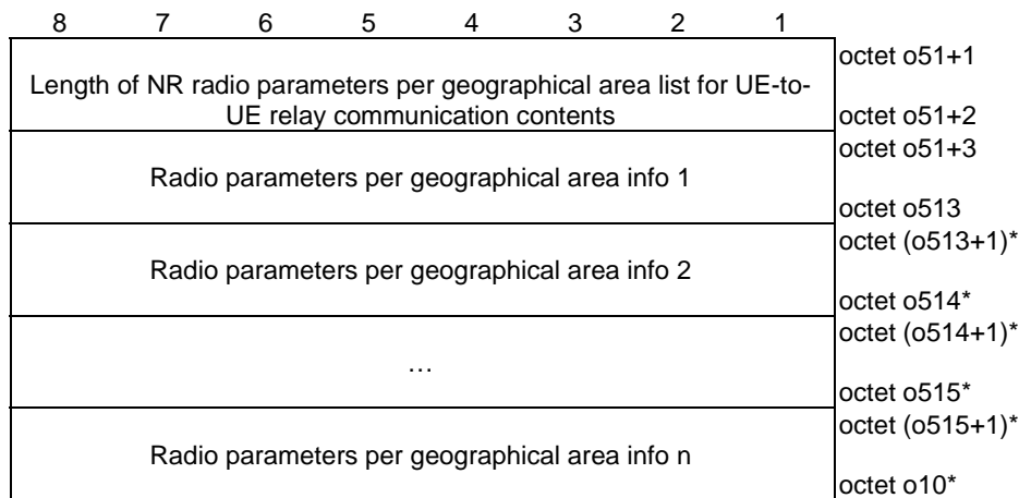
Figure 5.13.2.7: NR radio parameters per geographical area list for multi-hop UE-to-UE relay communication
