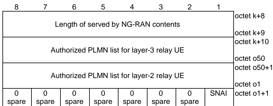
Figure 5.5.2.2: Served by NG-RAN
