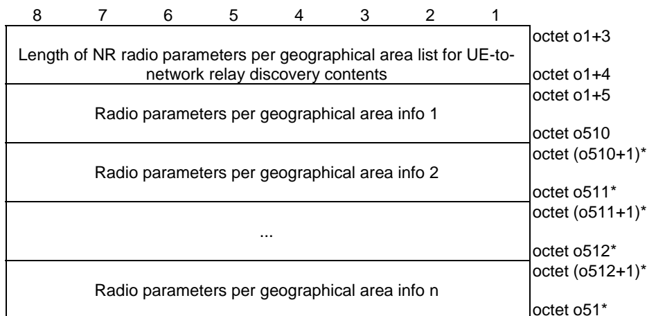
Figure 5.12.2.4: NR radio parameters per geographical area list for multi-hop UE-to-network relay discovery
