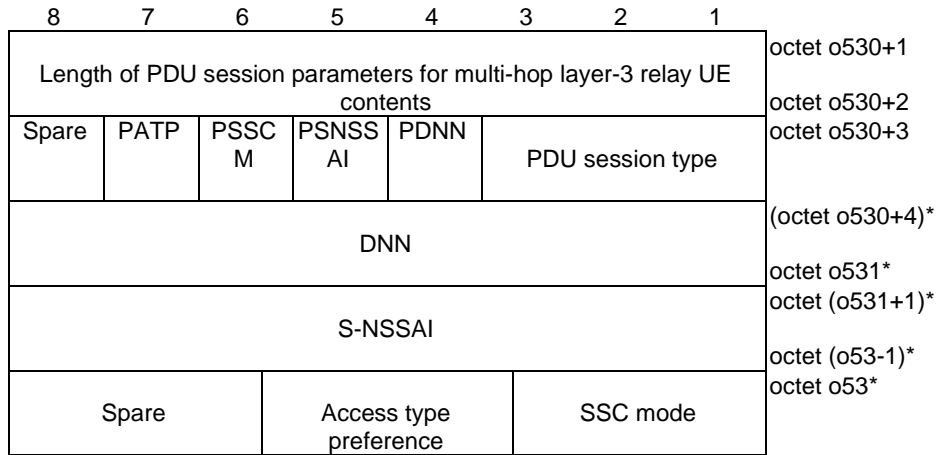
Figure 5.10.2.16: PDU session parameters for multi-hop layer-3 relay UE
