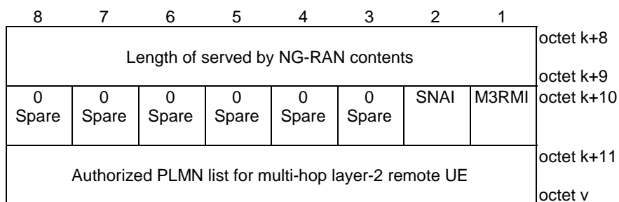
Figure 5.12.2.2: Served by NG-RAN
