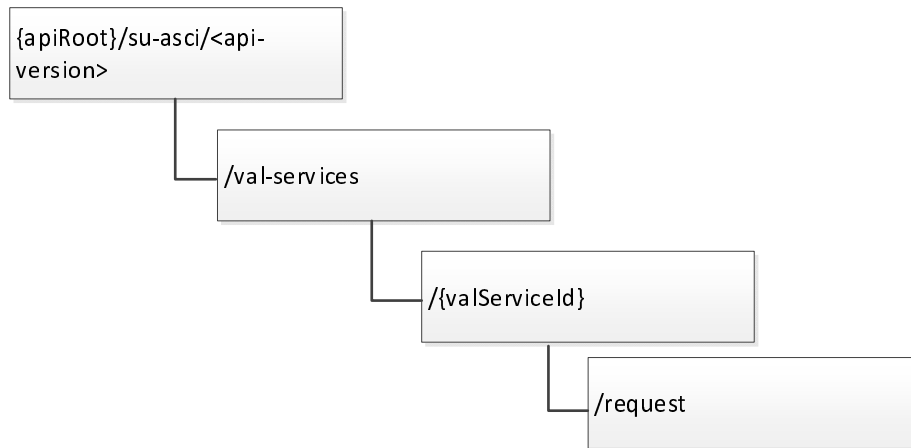
Figure C.4.2.2.1-1: Resource URI structure of the SU_ASCII provided by SCM-C
