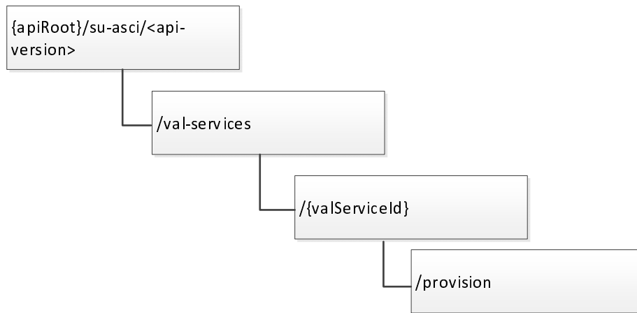
Figure C.4.1.2.1-1: Resource URI structure of the SU_ASCI provided by SCM-S
