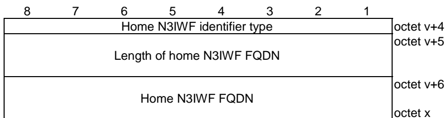
Figure 5.3.3.3.3: Home N3IWF identifier entry (Home N3IWF identifier type = "FQDN")
