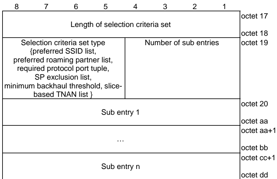
Figure 5.3.2.4b: Selection criteria set
