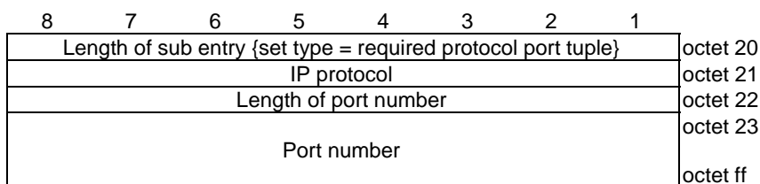
Figure 5.3.2.4e: Selection criteria sub entry {selection criteria set type = required protocol port tuple}
