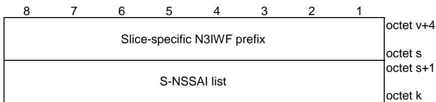
Figure 5.3.3.6.2: slice-specific N3IWF prefix entry
