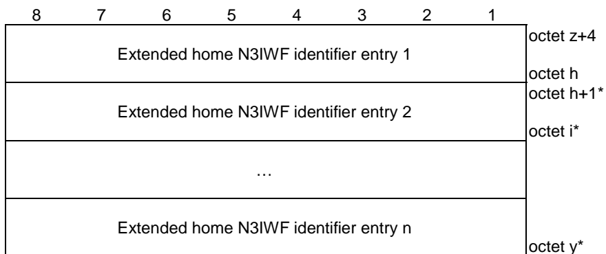
Figure 5.3.3.5.1: Content of extended home N3IWF identifier configuration
