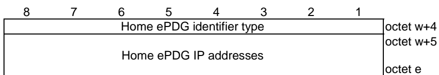
Figure 5.3.3.4.2: Home ePDG identifier entry (Home ePDG identifier type = "IPv4", "IPv6" or "IPv4v6")
