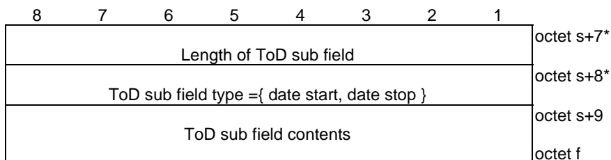
Figure 5.3.2.19: ToD sub field {field type = "date start" or "date stop"}
