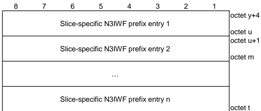
Figure 5.3.3.6.1: Content of slice-specific N3IWF prefix configuration
