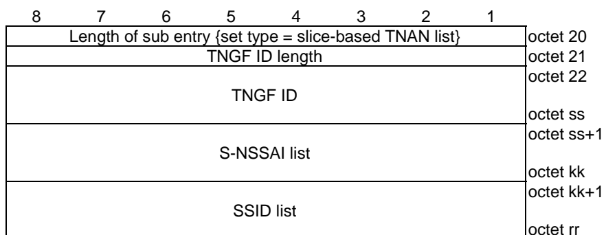
Figure 5.3.2.4h: Selection criteria sub entry {selection criteria set type = slice-based TNAN list}
