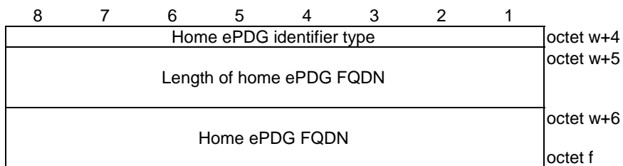
Figure 5.3.3.4.3: Home ePDG identifier entry (Home ePDG identifier type = "FQDN")
