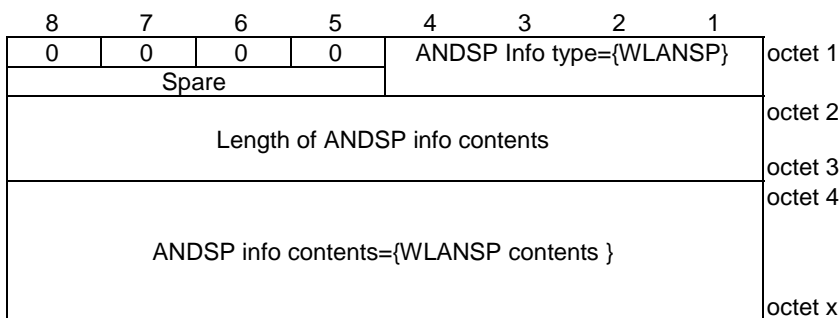
Figure 5.3.2.1: ANDSP Info type = {WLANSP}
