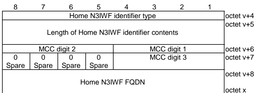
Figure 5.3.3.3.4: Home N3IWF identifier entry (Home N3IWF identifier type = "SNPN FQDN")
