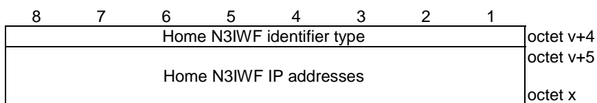
Figure 5.3.3.3.2: Home N3IWF identifier entry (Home N3IWF identifier type = "IPv4", "IPv6" or "IPv4v6")
