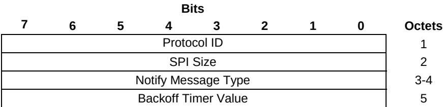
Figure 9.3.1.7-1: N3GPP_BACKOFF_TIMER Notify payload format
