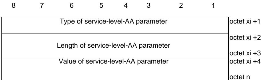
Figure 9.11.2.10.4: Service-level-AA parameter (when the type of service-level-AA parameter field contains an IEI of a type 6 information element as specified in 3GPP TS 24.007 [11])
