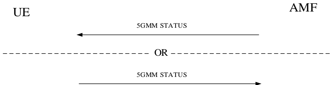
Figure 5.4.6.1: 5GMM status procedure
