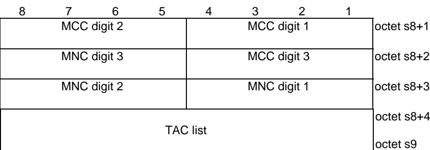
Figure 9.11.3.51.11E: Tracking area information of PLMN
