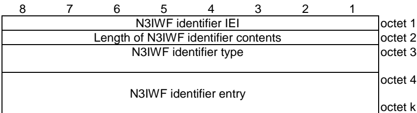
Figure 9.11.3.93.1: N3IWF identifier information element
