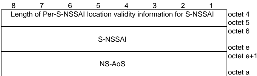
Figure 9.11.3.100.2: Per-S-NSSAI location validity information for S-NSSAI
