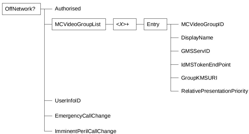
Figure 13.1.3: The MCVideo user profile MO (3 of 3)
