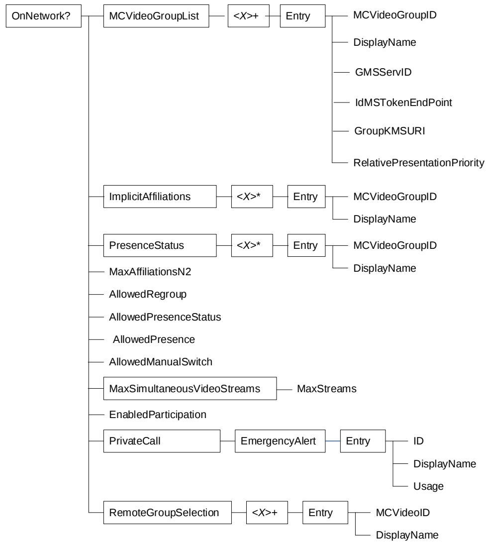
Figure 13.1.2: The MCVideo user profile MO (2 of 3)
