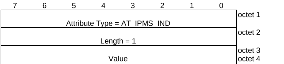
Figure 8.2.1.1: AT_IPMS_IND attribute
