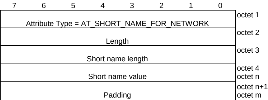
Figure 8.2.5.2-1: AT_SHORT_NAME_FOR_NETWORK attribute
