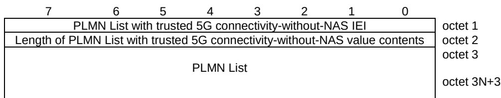
Figure H.2.4.5-1: PLMN List with trusted 5G connectivity-without-NAS information element
