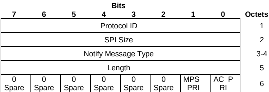
Figure 8.2.9.22-1: HPA_INFO Notify payload format
