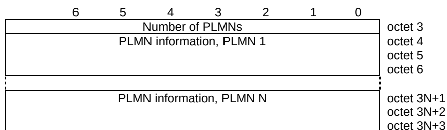
Figure H.2.4.2-1a: PLMN List
