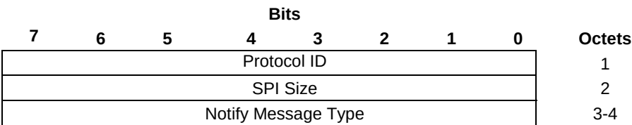
Figure 8.2.9.6-1: REACTIVATION_REQUESTED_CAUSE Notify payload format
