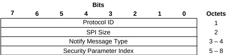
Figure 8.2.9.12-1: MODIFIED_BEARER Notify payload format
