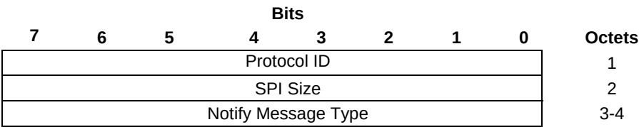
Figure 8.2.9.7-1: EMERGENCY_SUPPORT Notify Payload format
