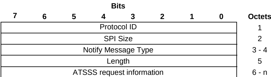
Figure 8.2.9.20-1: ATSSS_REQUEST Notify payload format
