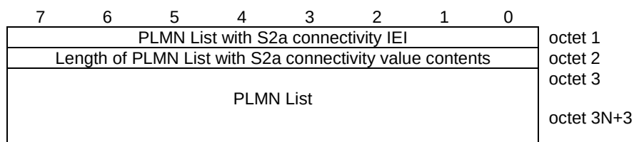
Figure H.2.4.3-1: PLMN List with S2a connectivity information element
