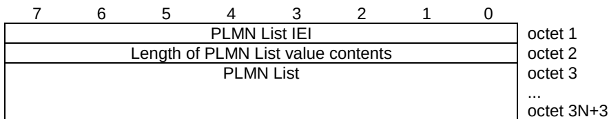
Figure H.2.4.2-1: PLMN List information element
