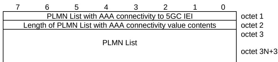
Figure H.2.4.6-1: PLMN List with AAA connectivity to 5GC information element
