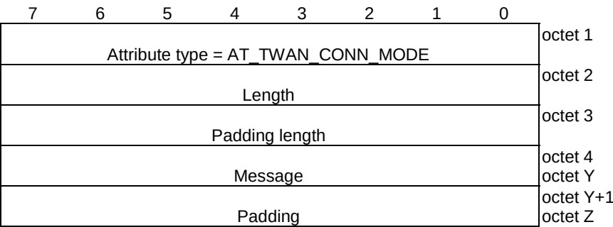
Figure 8.2.7.1-1: AT_TWAN_CONN_MODE attribute
