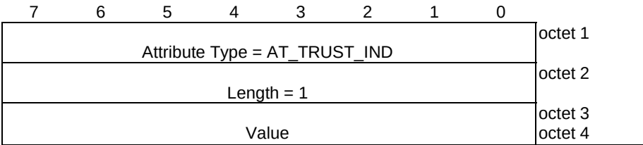
Figure 8.2.3.1-1: AT_TRUST_IND attribute
