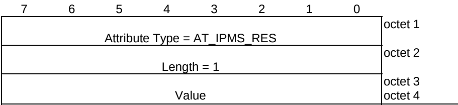
Figure 8.2.1.2: AT_IPMS_RES attribute.
