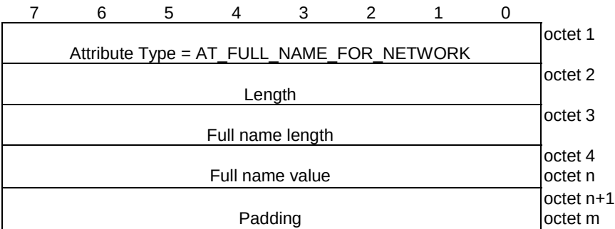
Figure 8.2.5.1-1: AT_FULL_NAME_FOR_NETWORK attribute
