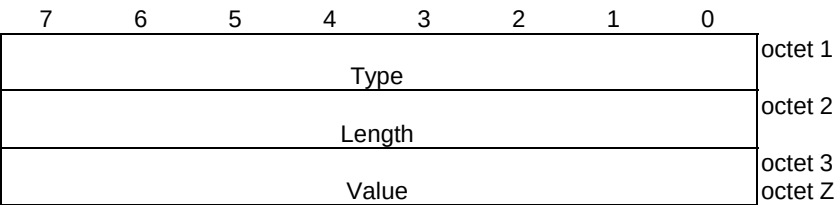
Figure 8.1.4.2-1: Item
