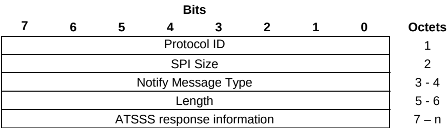
Figure 8.2.9.21-1: ATSSS_RESPONSE Notify payload format
