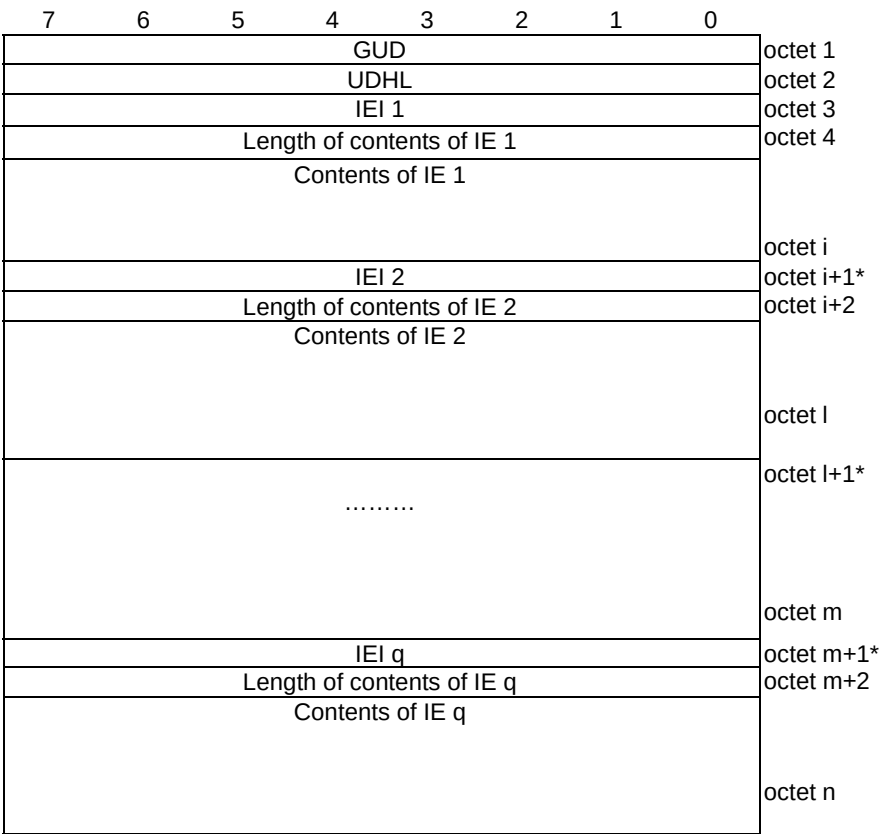
Figure H.2.1-1 – Structure of IEEE Std 802.11 Generic Container
