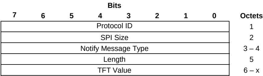
Figure 8.2.9.11-1: TFT Notify payload format
