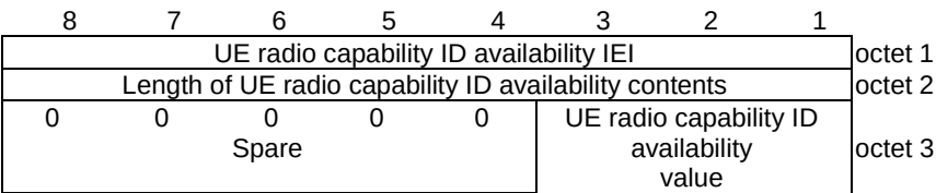
Figure 9.9.3.58.1: UE radio capability ID availability information element
