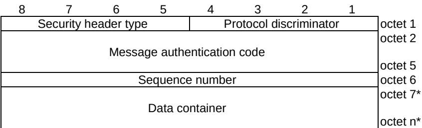
Figure 9.1.3: General message organization for EMM TRANSPORT
