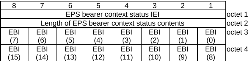
Figure 9.9.2.1.1: EPS bearer context status information element
