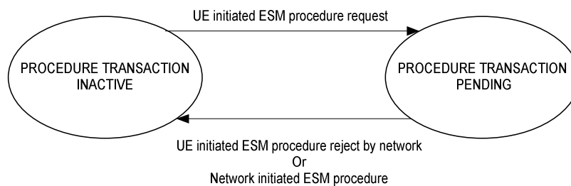
Figure 6.1.3.2.4.1: The procedure transaction states in the UE (overview)
