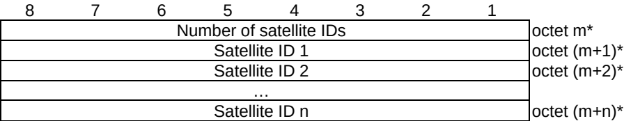
Figure 9.9.3.73.2: S&F monitoring list
