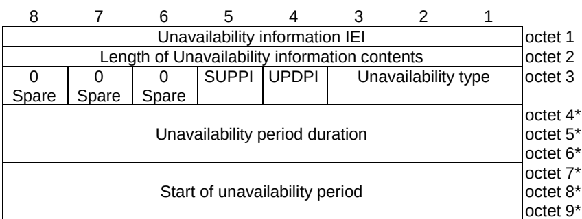
Figure 9.9.3.69.1: Unavailability information information element
