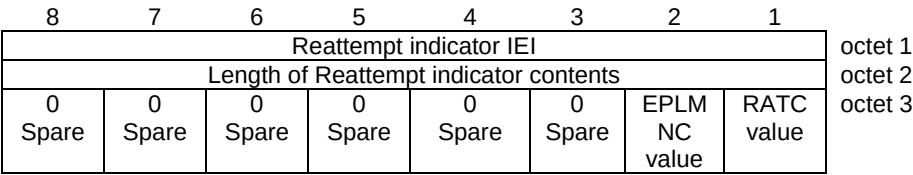
Figure 9.9.4.13A: Re-attempt indicator information element
