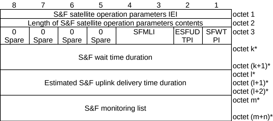
Figure 9.9.3.73.1: S&F satellite operation parameters information element
