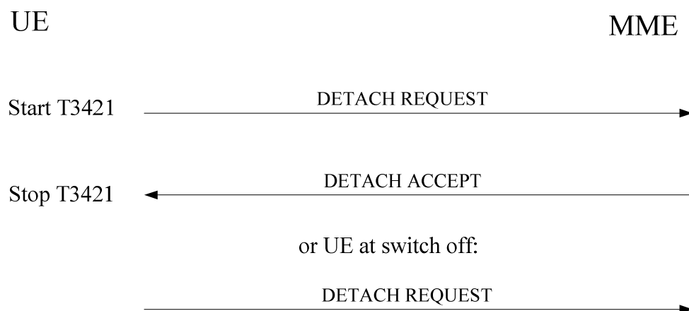
Figure 5.5.2.1.1: UE initiated detach procedure
