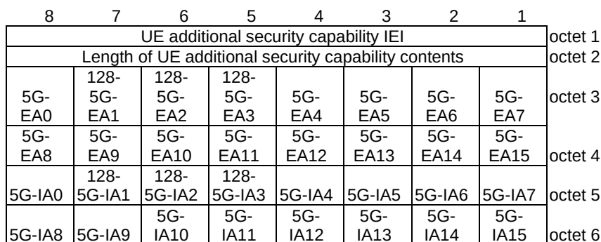
Figure 9.9.3.53.1: UE additional security capability information element
