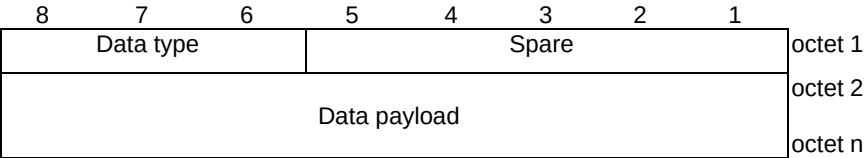
Figure 9.9.3.74.3: Data container IE for Data type "SMS"
