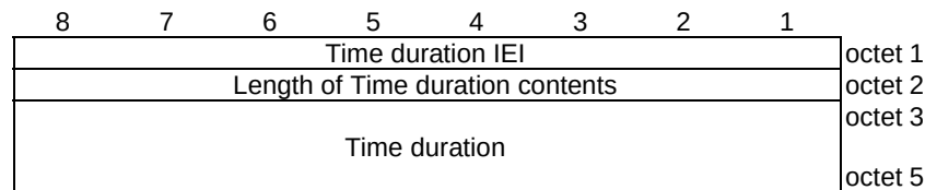
Figure 9.9.3.68.1: Time duration information element
