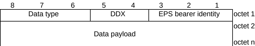
Figure 9.9.3.74.1: Data container IE for Data type "Control plane user data"
