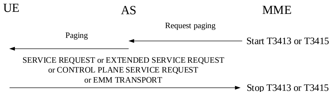
Figure 5.6.2.2.1.1: Paging procedure using S-TMSI
