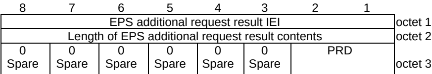
Figure 9.9.3.67.1: EPS additional request result information element
