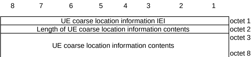
Figure 9.9.3.72.1: UE coarse location information information element
