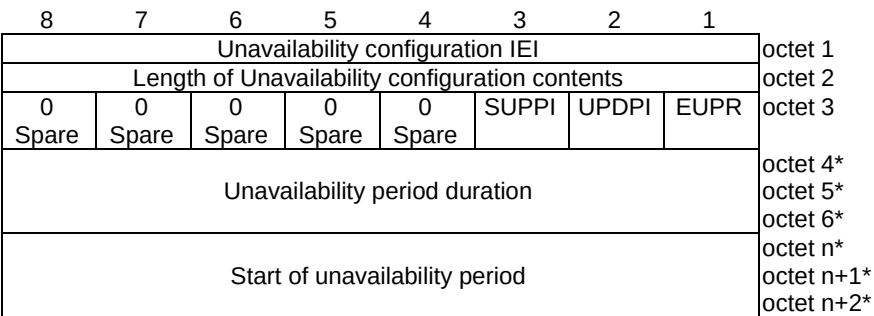
Figure 9.9.3.70.1: Unavailability configuration information element
