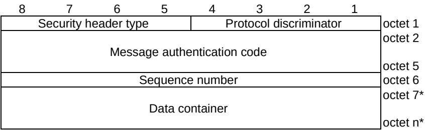
Figure 9.1.3: General message organization for EMM TRANSPORT
