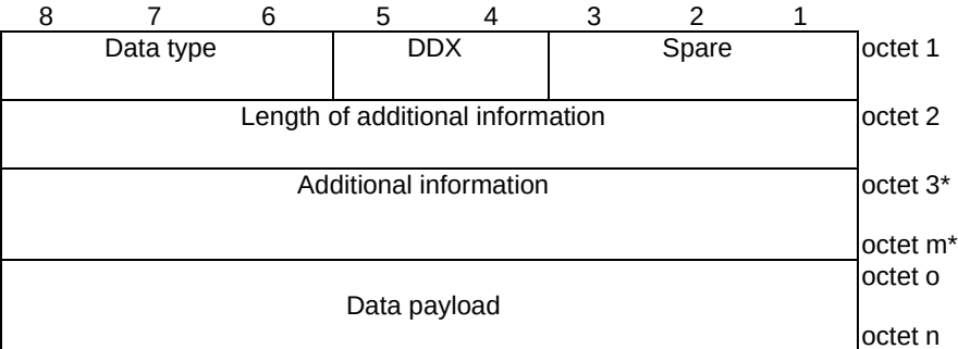
Figure 9.9.3.74.2: Data container IE for Data type "Location services message container"
