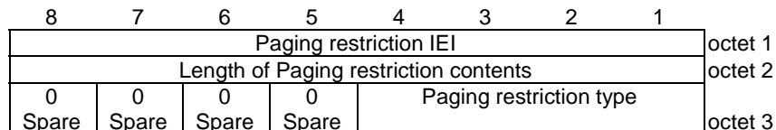
Figure 9.9.3.66.1: Paging restriction information element for Paging restriction type = "All paging is restricted" and for Paging restriction type = "All paging is restricted except voice"
