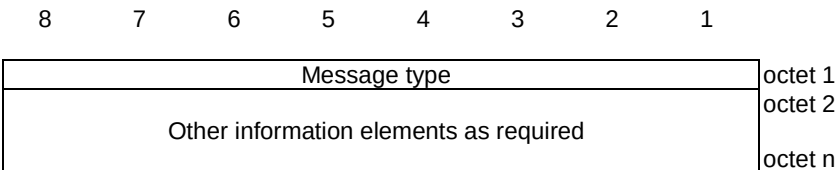
Figure 15.2.1-2: General message organization example
