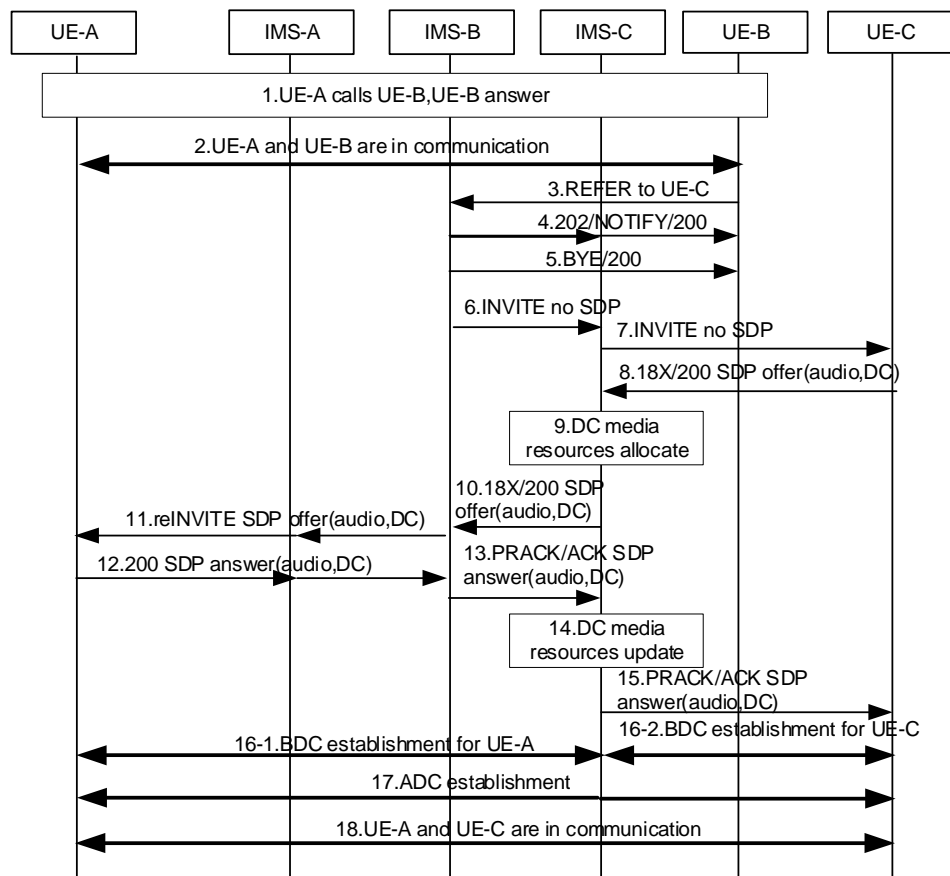
Figure A.1.3.3.1-1: Blind Transfer when IMS serving the transfer target provides data channel service
