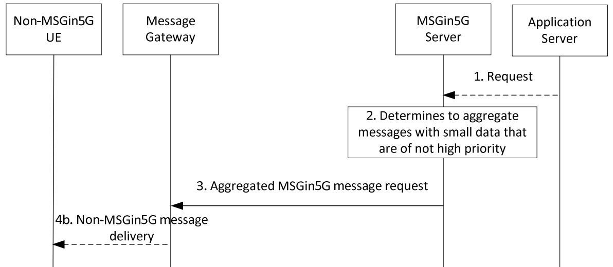
Figure 8.4.3-2: MSGin5G Server aggregates messages towards target Non-MSGin5G UE
