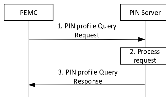
Figure 8.5.5.2-1: Query PIN profile procedure
