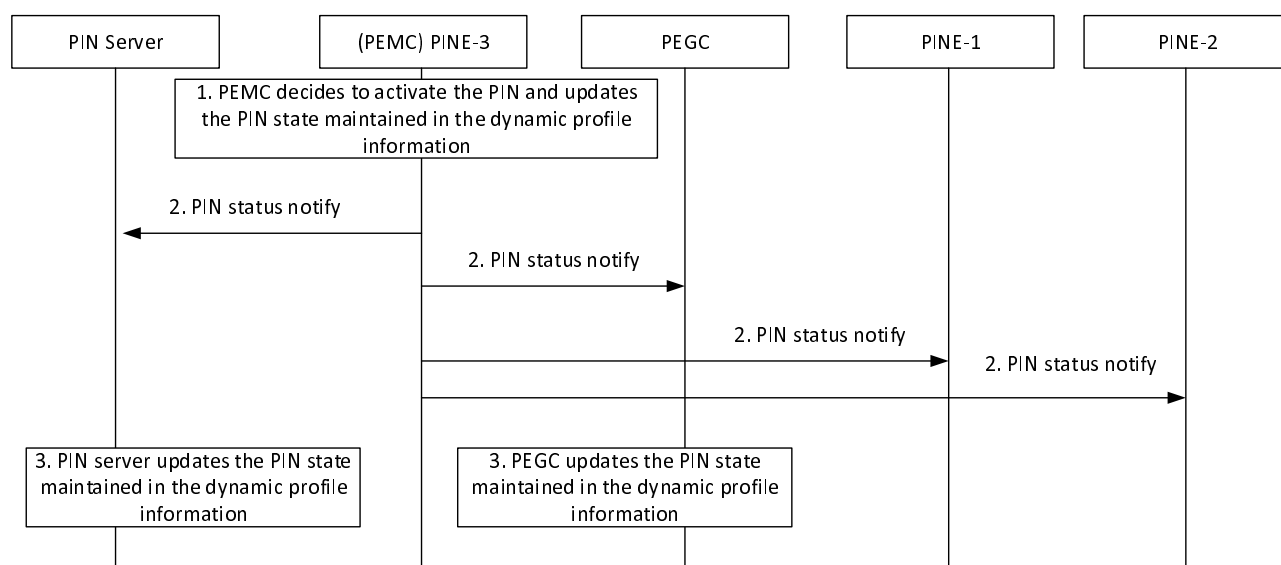
Figure 8.5.13.2.1-1: Activation of PIN by PEMC
