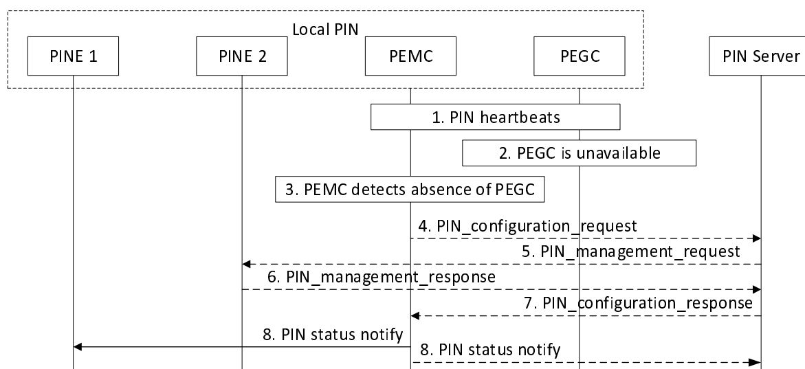
Figure 8.5.10.2.3-1: PIN Modification due to PEGC unavailability
