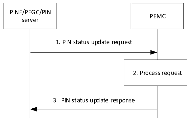
Figure 8.5.9.2.3-1: PIN status update
