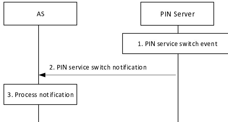
Figure 8.7.2.1.4.2.2-1: PIN service switch notify procedure
