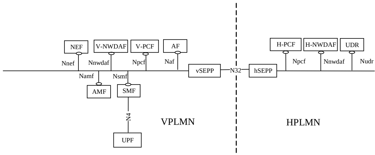
Figure 5.2.2-1: Overall roaming reference architecture of policy and charging control framework for the 5G System - local breakout scenario
