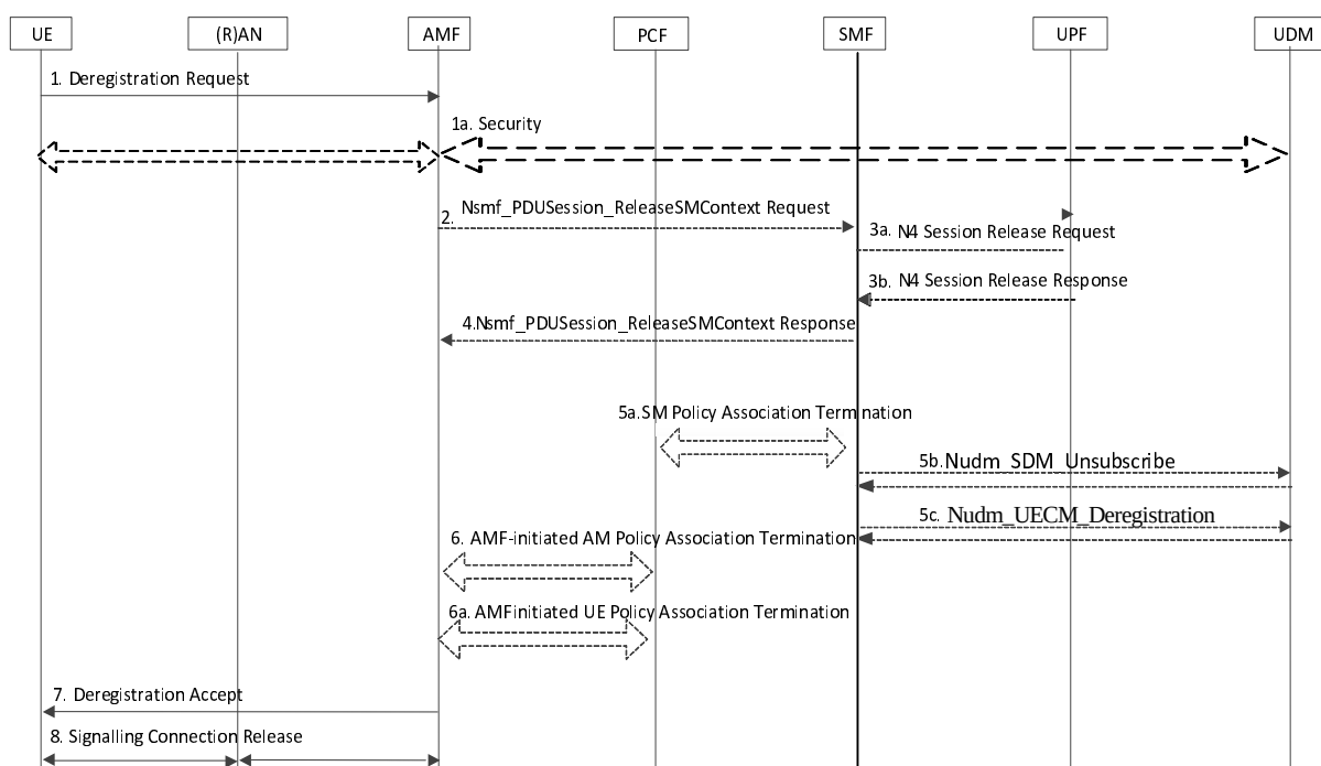
Figure 4.2.2.3.2-1: UE-initiated Deregistration
