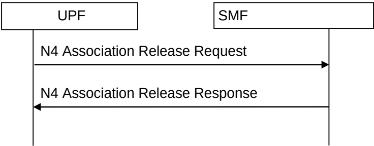
Figure 4.4.3.3-2: UPF initiated N4 association release procedure
