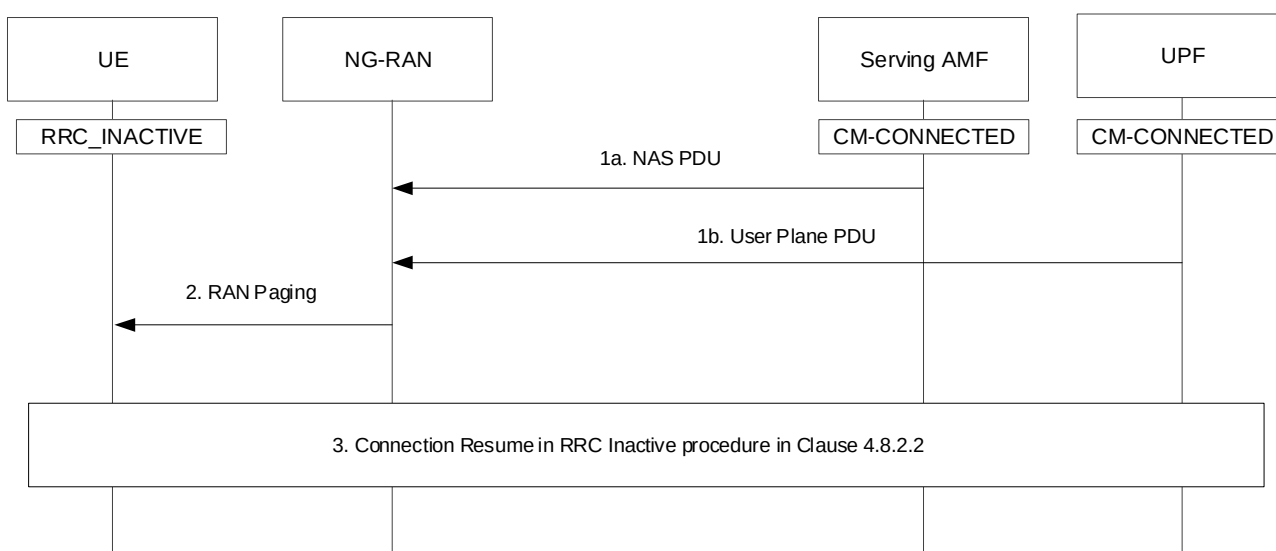
Figure 4.8.2.2a-1: Network Triggerred Connection Resume for UE in RRC_INACTIVE
