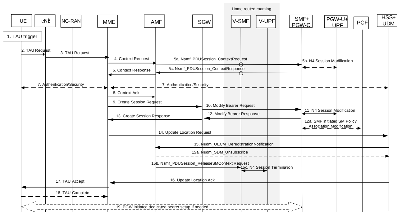
Figure 4.11.1.3.2-1: 5GS to EPS Idle mode mobility using N26 interface
