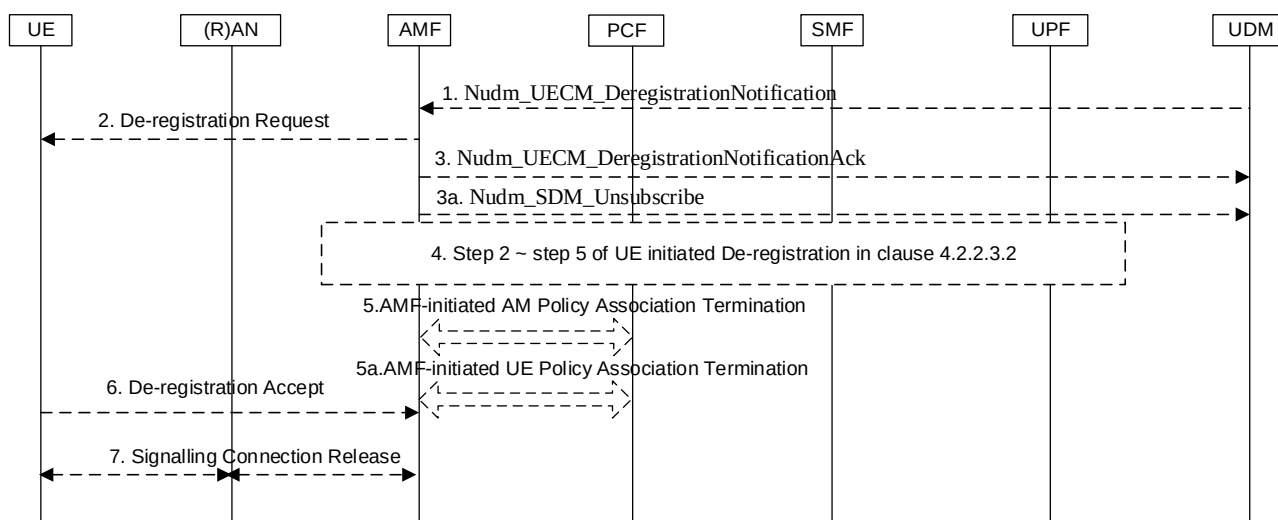
Figure 4.2.2.3.3-1: Network-initiated Deregistration
