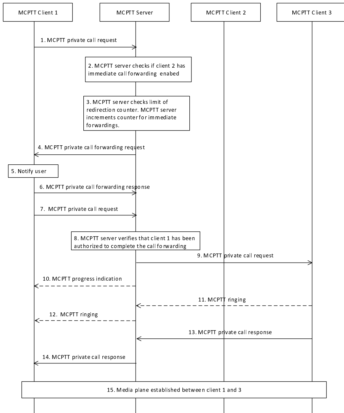
Figure 10.7.5.2.2-1: Call forwarding immediate for private calls
