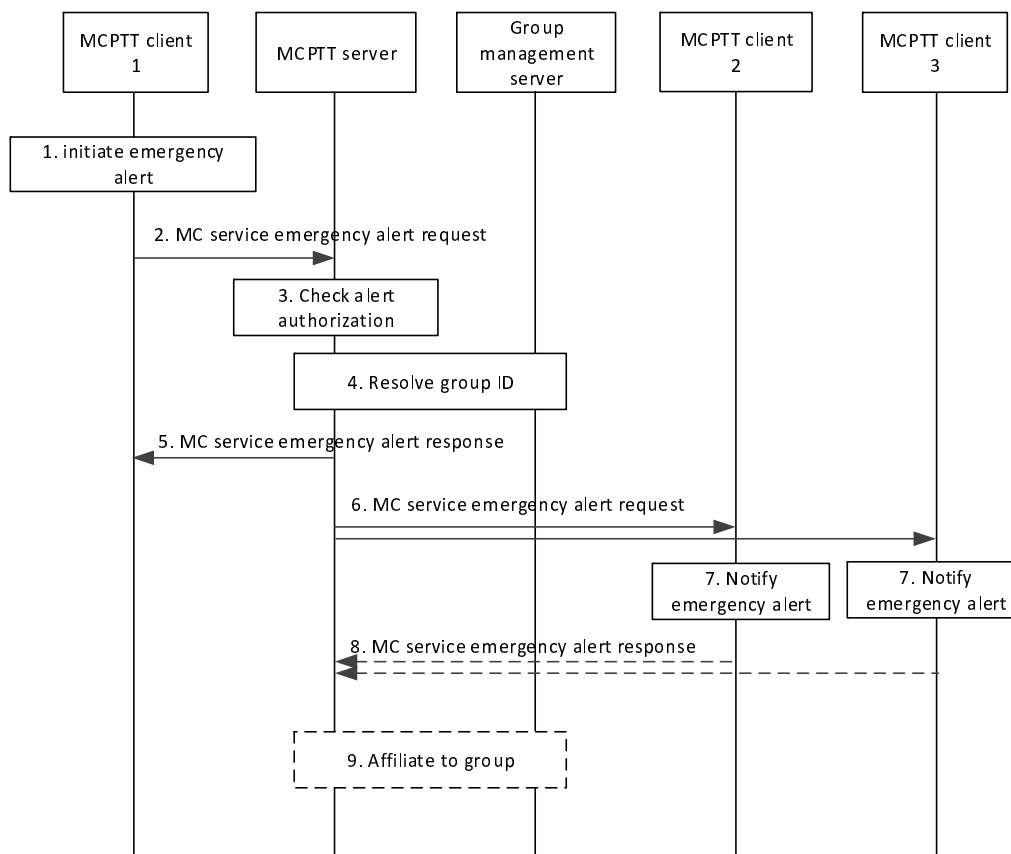
Figure 10.6.2.6.3.1-1 MCPTT emergency alert
