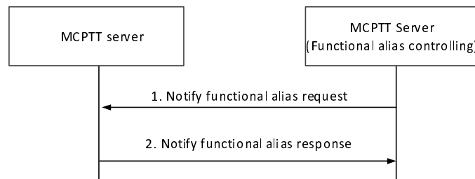
Figure 10.18.3.2-1: Notification for the functional alias
