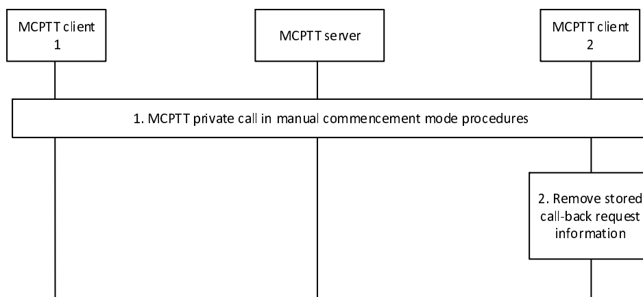
Figure 10.7.4.4-1: MCPTT private call call-back request fulfillment – MCPTT users in the same MCPTT system
