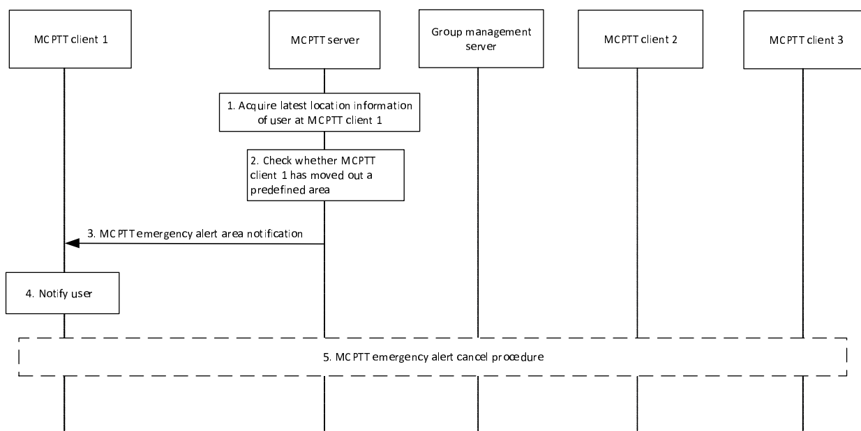
Figure 10.6.2.6.3.4-1 Leaving MCPTT emergency alert area
