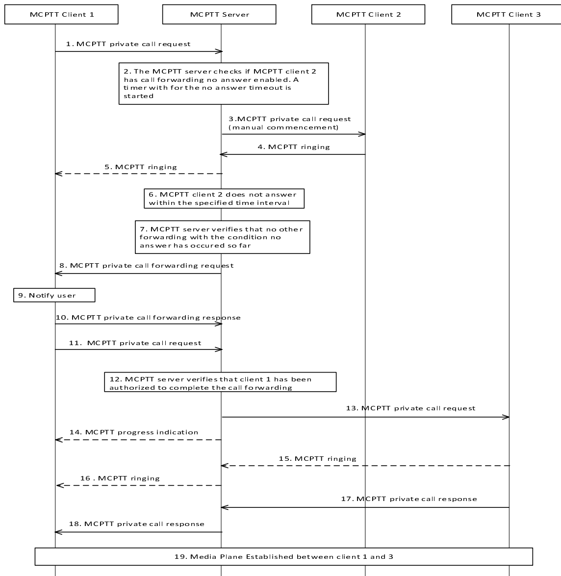
Figure 10.7.5.2.3-1: Call forwarding no answer for private call
