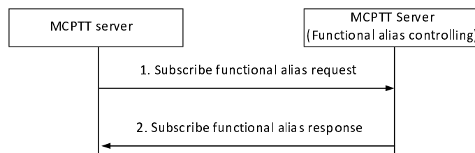
Figure 10.18.3.1-1: Subscription for functional alias
