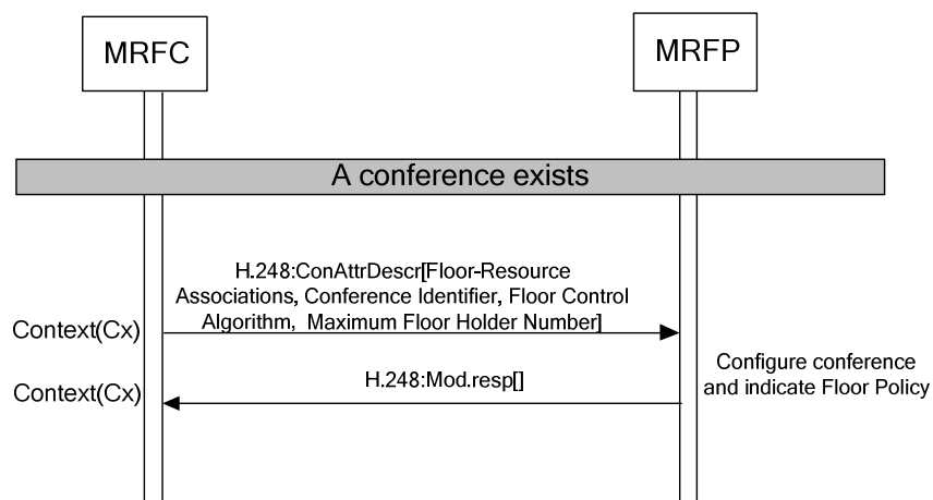
Figure 6.2.13.2.1 Procedure to Configure Conference for Floor Control
