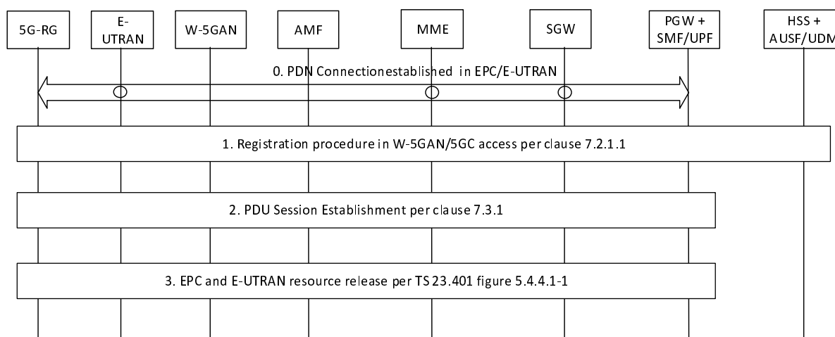
Figure 7.6.4.1-1: Handover from EPS to W-5GAN/5GC
