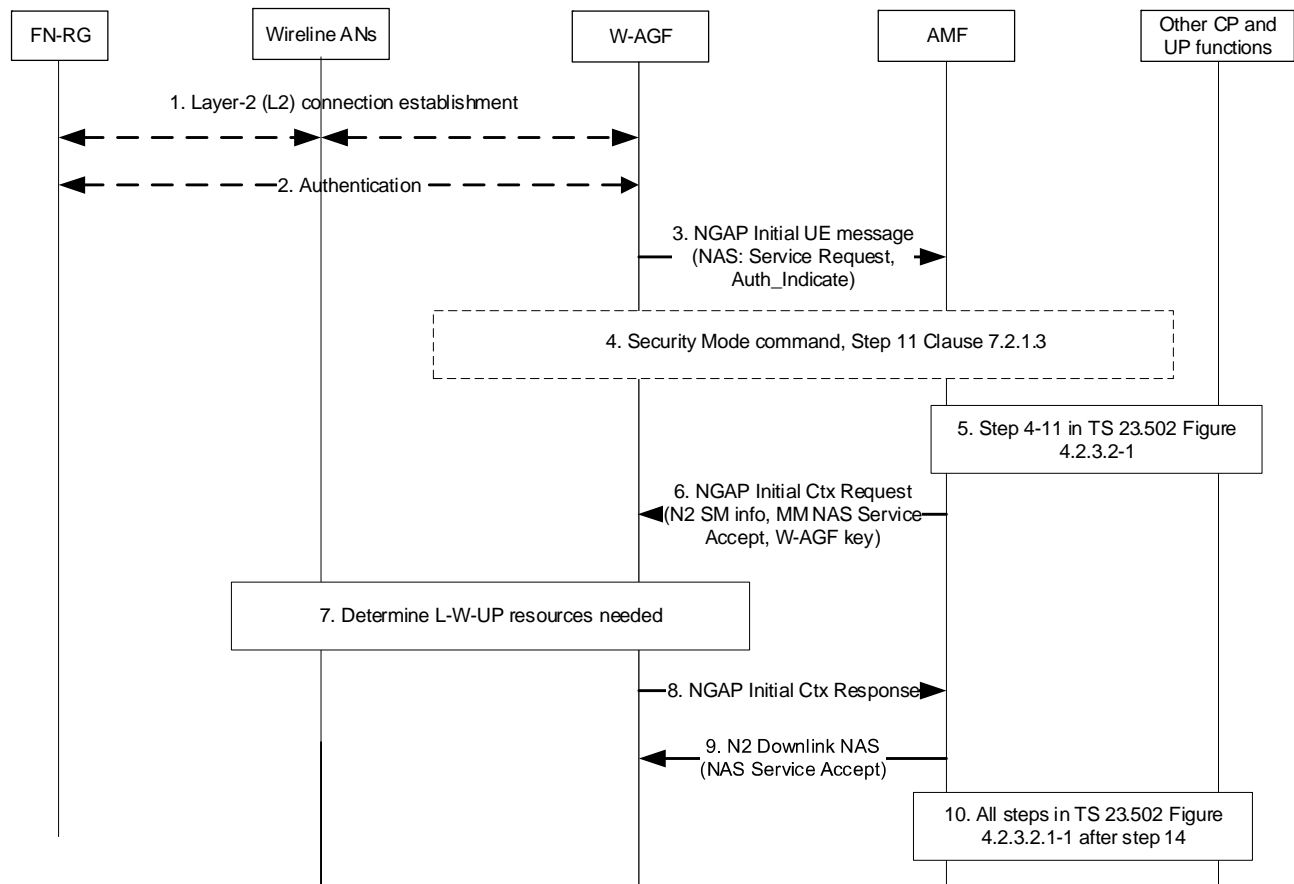
Figure 7.2.2.2-1: FN-RG Service Request procedure via W-5GAN
