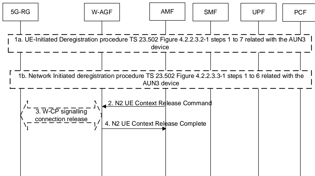
Figure 7.2.8.2-1: De-registration of an AUN3 device
