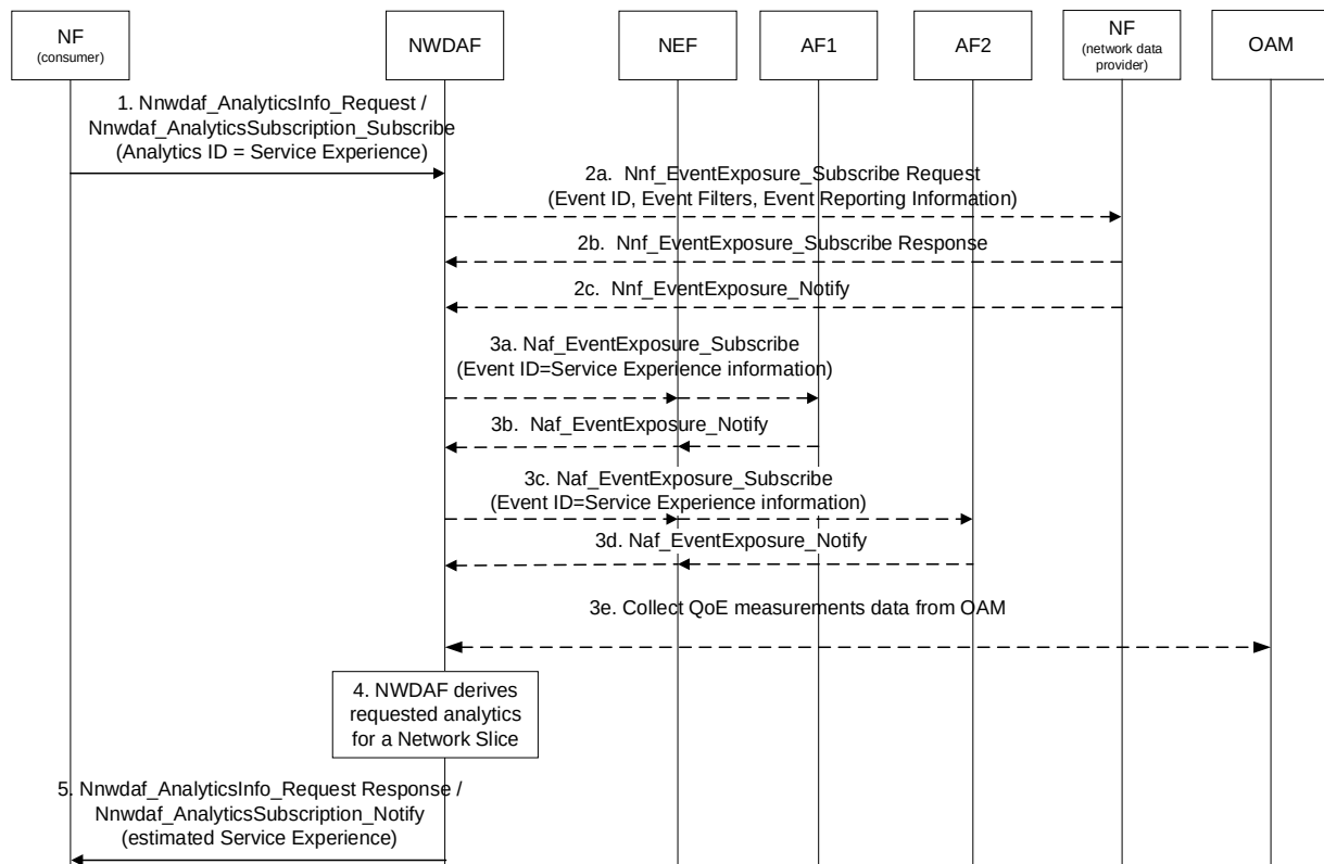
Figure 6.4.5-1: Procedure for NWDAF providing Service Experience for a UE or a group of UEs in a Network Slice
