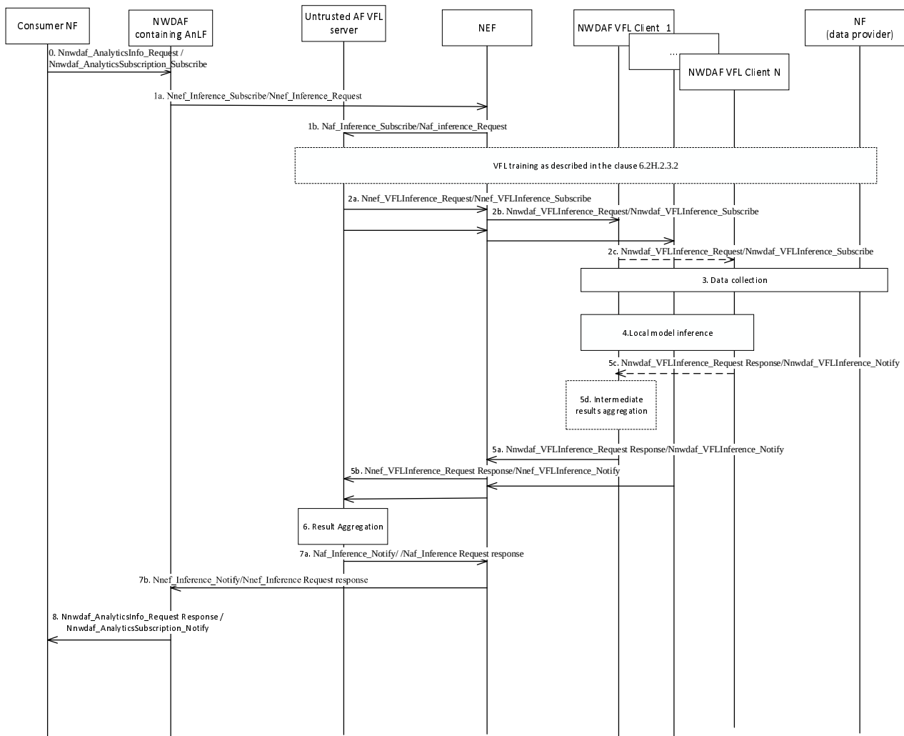
Figure 6.2H.2.4.2-1: Inference procedure for vertical federated learning when untrusted AF is acting as VFL server
