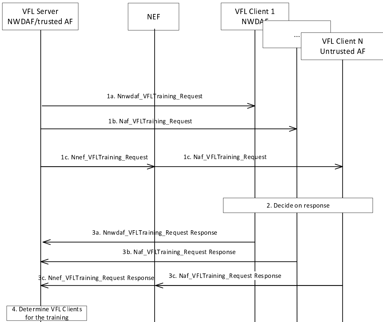
Figure 6.2H.2.2.1-1: Preparation procedure for Vertical Federated Learning when NWDAF/Trusted AF is the VFL Server
