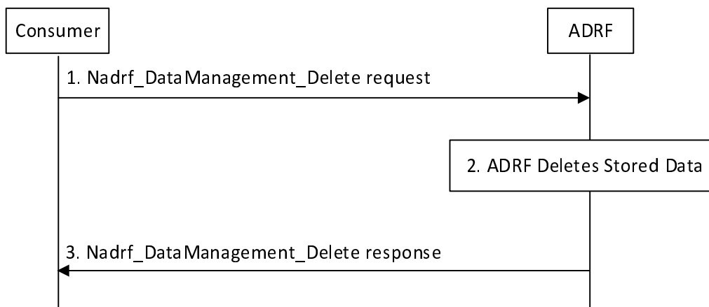
Figure 6.2B.4-1: Data Removal from an ADRF
