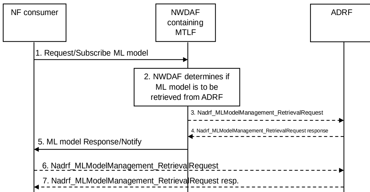
Figure 6.2B.7-1: Procedure for ML Model(s) retrieval from ADRF
