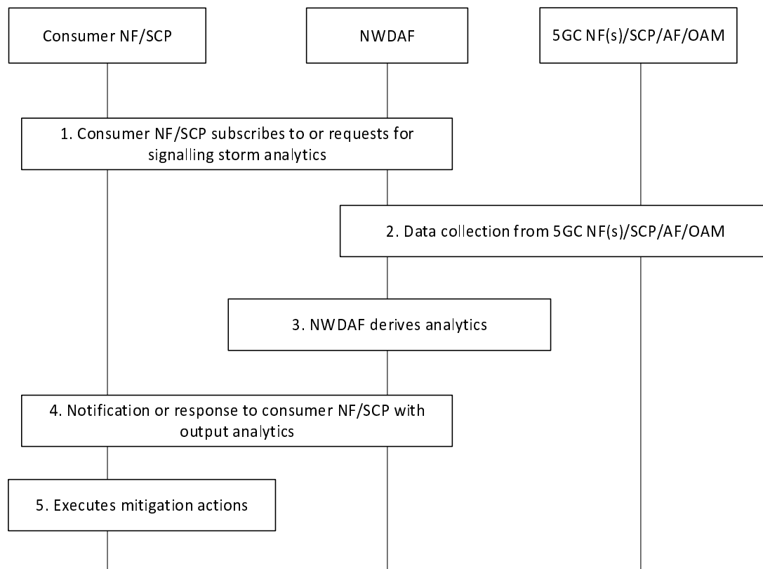
Figure 6.22.4-1: Procedure for NWDAF-assisted Network Signalling Storm Mitigation and Prevention
