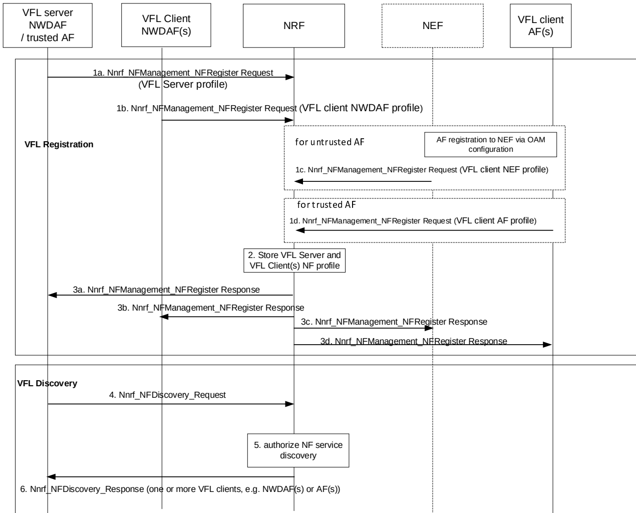
Figure 6.2H.2.1.1-1: Registration and Discovery procedure for Vertical Federated Learning when NWDAF or trusted AF is acting as VFL server
