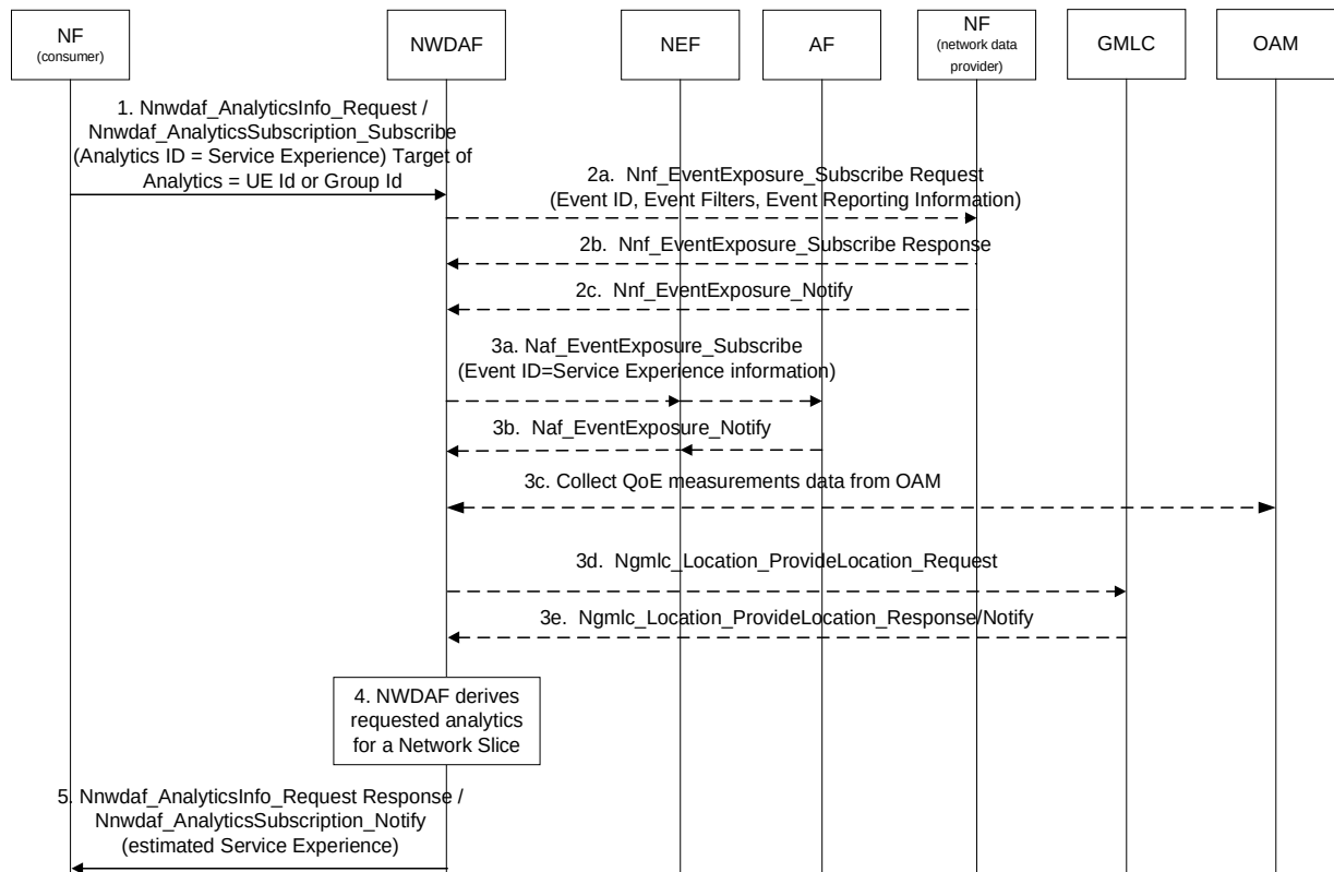
Figure 6.4.6-1: Procedure for NWDAF providing Service Experience for an application for a UE or a group of UEs
