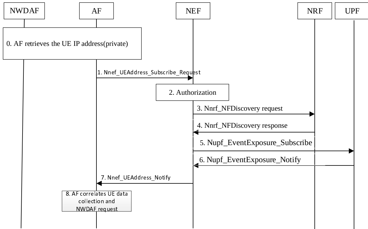
Figure 6.2.8.2.4.5-1: AF correlates UE data collection and NWDAF request when there is NAT between UE and AF
