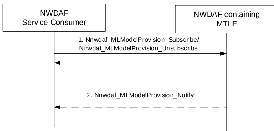
Figure 6.2A.1-1: ML Model for analytics subscribe/unsubscribe
