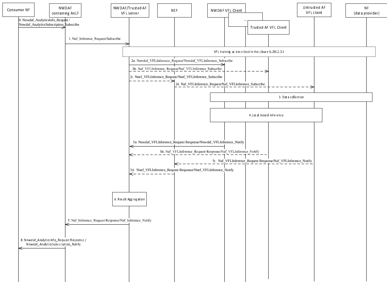
Figure 6.2H.2.4.1-1: Inference procedure for vertical federated learning when NWDAF or Trusted AF is acting as VFL server
