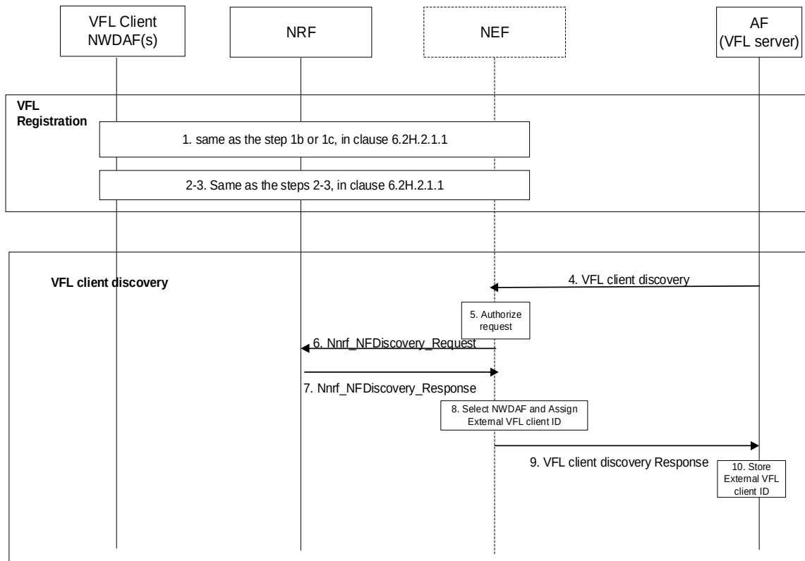
Figure 6.2H.2.1.2-1: Registration and Discovery procedure for Vertical Federated Learning when an untrusted AF is acting as VFL server and NWDAF(s) are the VFL clients
