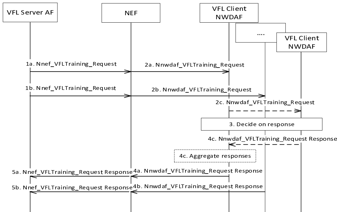
Figure 6.2H.2.2.2-1: Preparation procedure for Vertical Federated Learning when untrusted AF is the VFL Server
