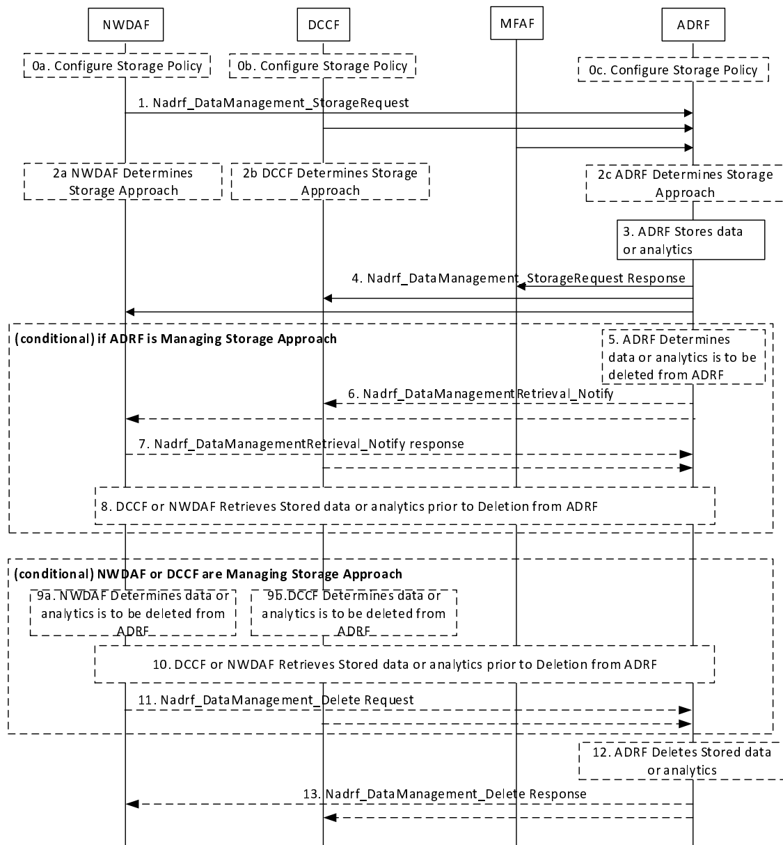
Figure 6.2B.2-1: Historical Data and Analytics storage
