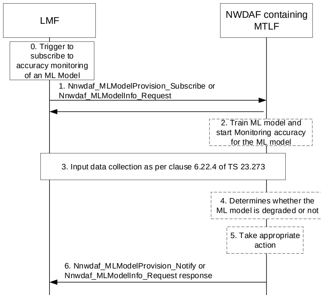
Figure 6.2E.4-1: Monitoring performance of ML Model used for LMF-based AI/ML positioning
