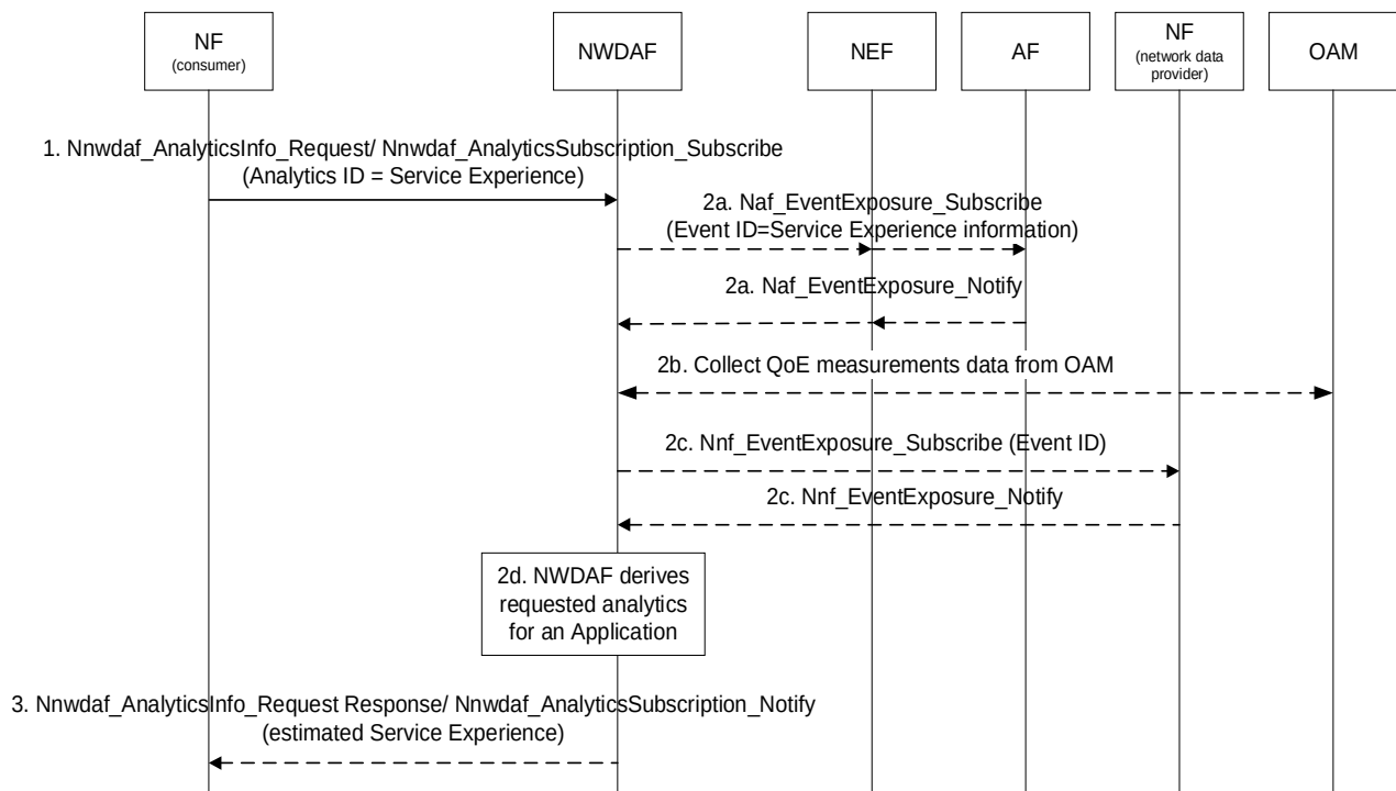
Figure 6.4.4-1: Procedure for NWDAF providing Service Experience for an Application
