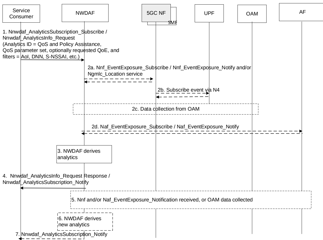
Figure 6.23.4-1: Procedure for QoS and Policy Assistance Analytics
