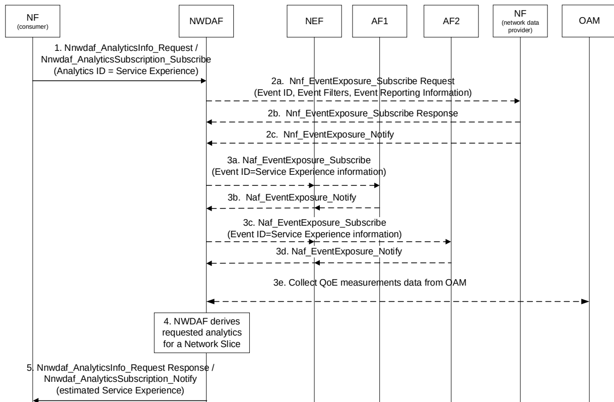
Figure 6.4.5-1: Procedure for NWDaf providing Service Experience for a UE or a group of UEs in a Network Slice
