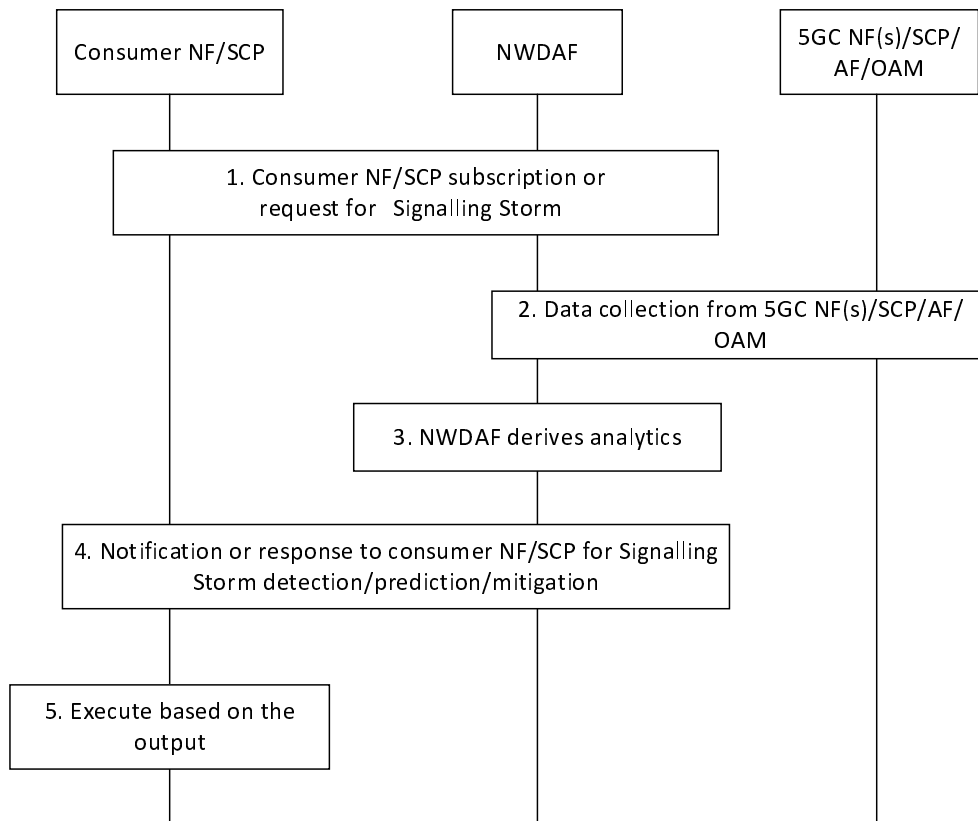
Figure 6.22.4-1: Procedure for NWDAF-assisted Network Signalling Storm Mitigation and Prevention
