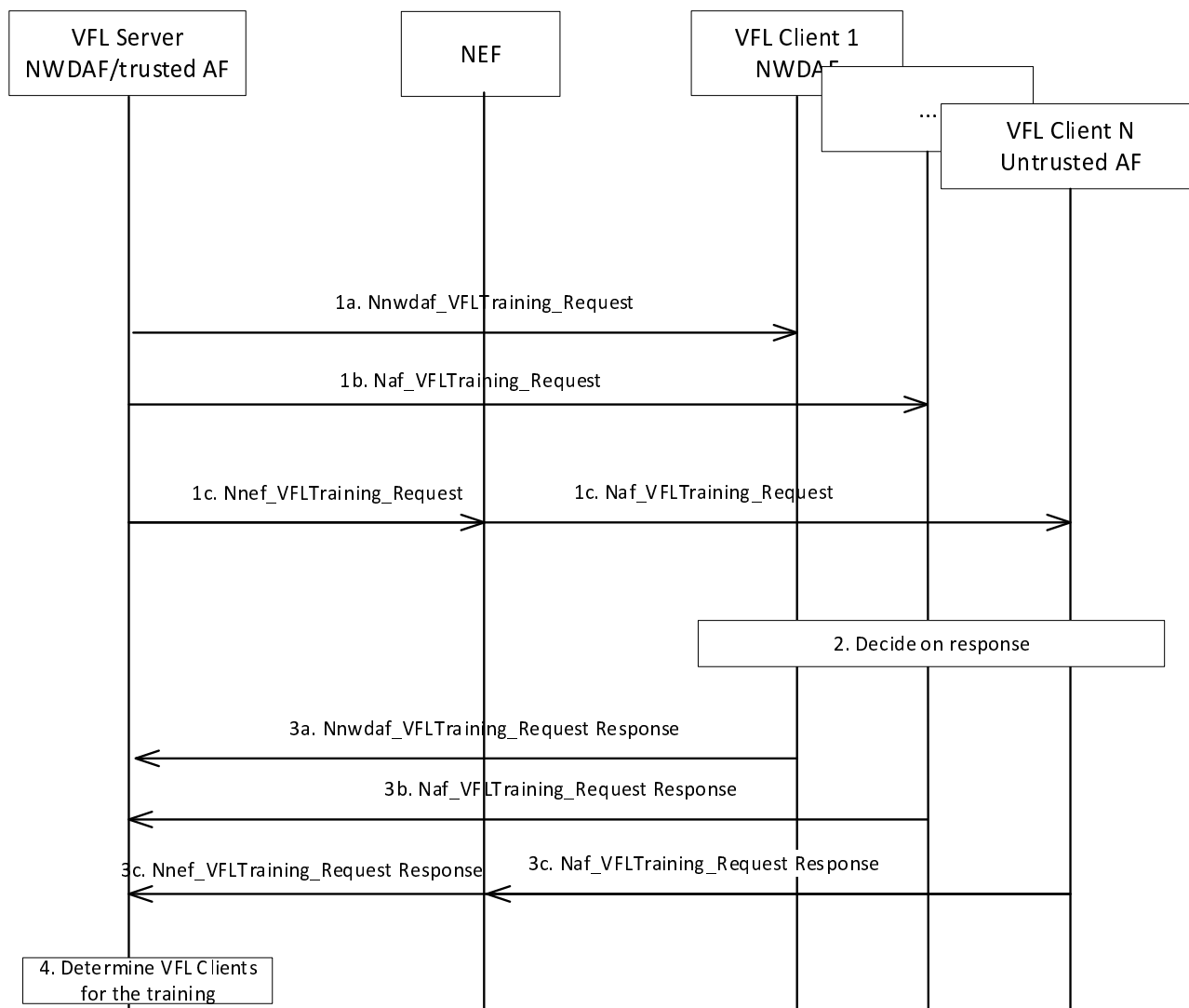
Figure 6.2H.2.2-1: Preparation procedure for Vertical Federated Learning when NWDAF/Trusted AF is the VFL Server
