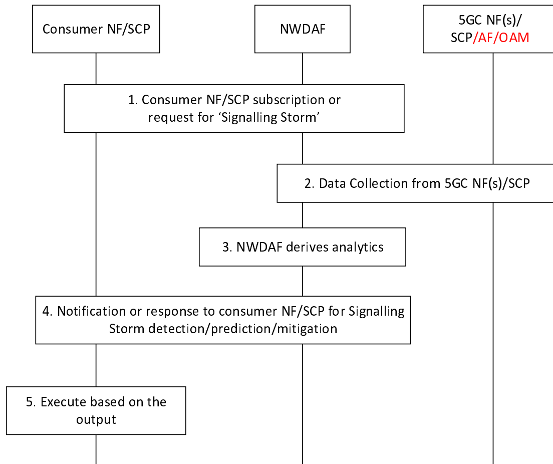
Figure 6.22.4-1: Procedure for NWDAF-assisted Network Signalling Storm Mitigation and Prevention
