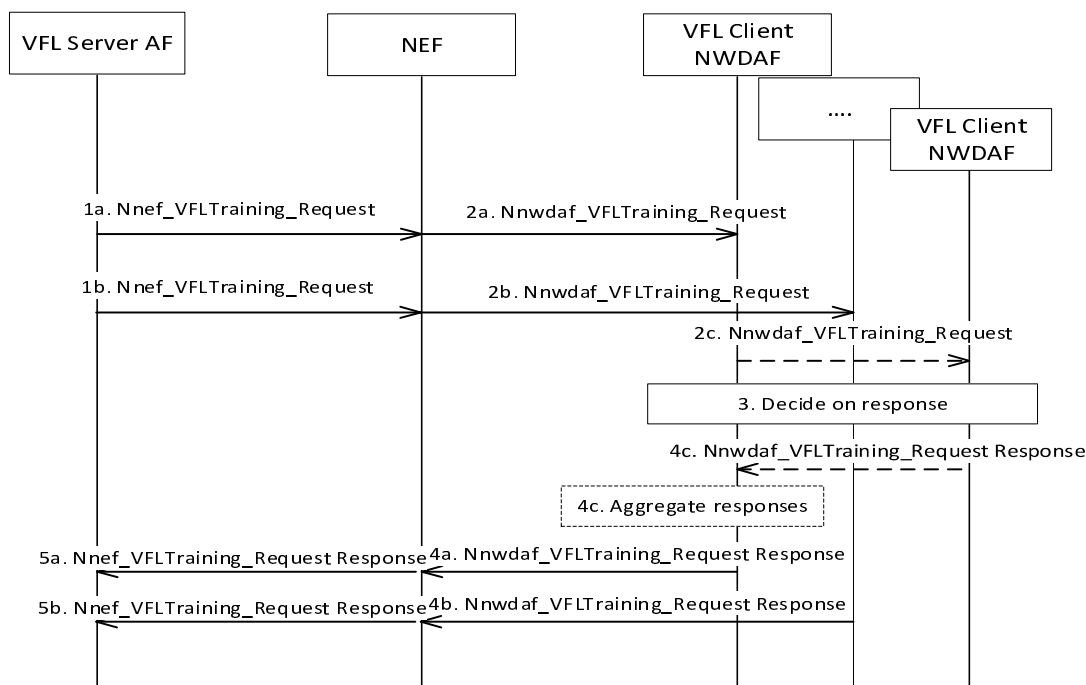
Figure 6.2H.2.2-1: Preparation procedure for Vertical Federated Learning when untrusted AF is the VFL Server
