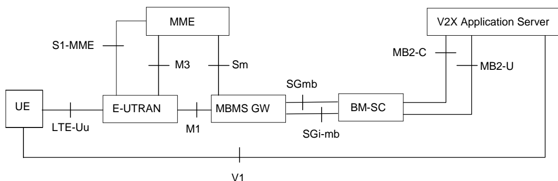
Figure 4.2.2-1a: Reference architecture for MBMS for LTE-Uu based V2X communication via MB2
