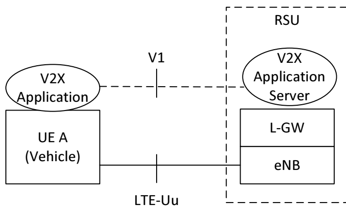
Figure A-2: RSU includes an eNB, L-GW and a V2X Application Server
