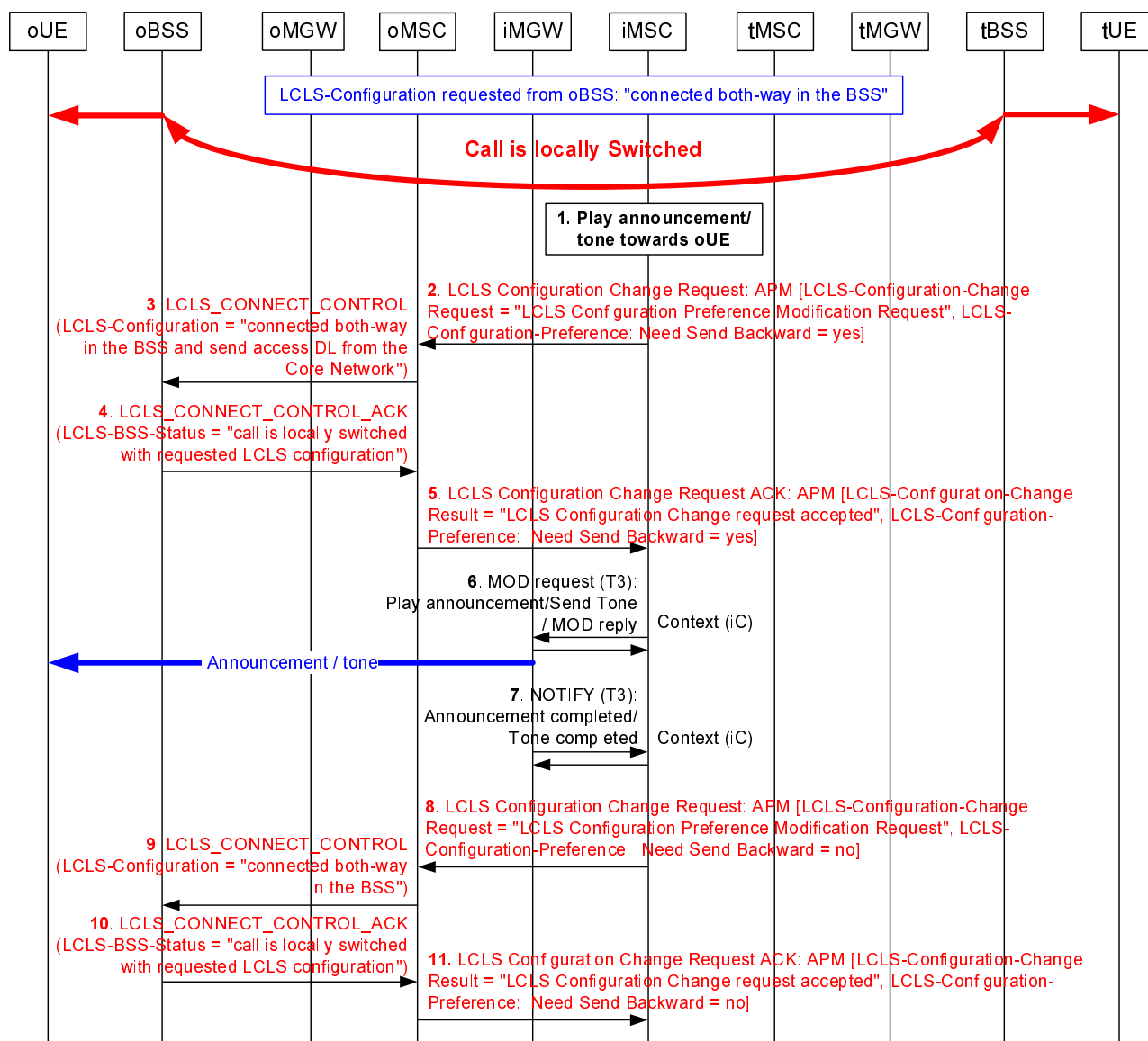
Figure 14.6.2.5.2.1: Mid-Call Announcement/Tone Flow
