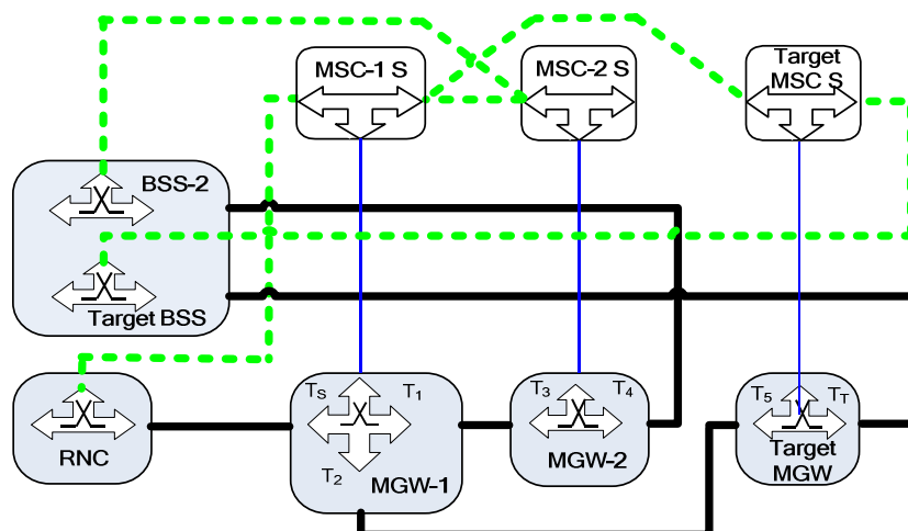
Connection Model 2: During Handover, T_2 is isolated from T_S , T_1 is one-way connected to T_2
