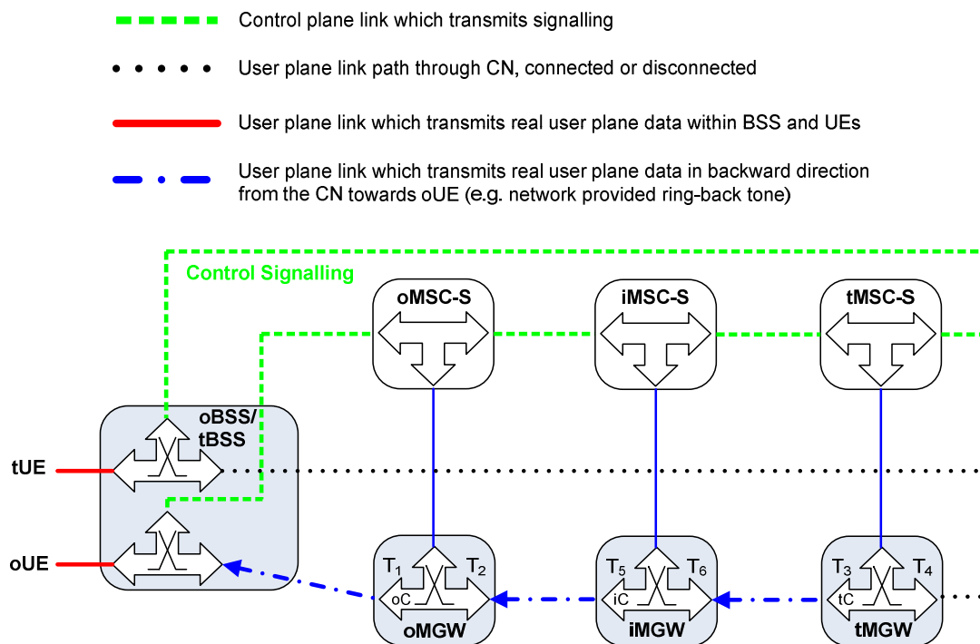
Connection Model 1: After Alerting, Backward Through Connection
