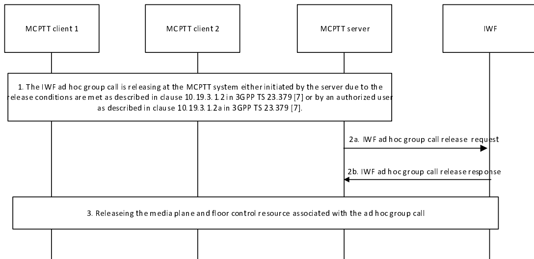
Figure 10.17.3.3-1: Release IWF ad hoc group call by the MC system
