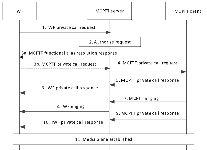
Figure 10.4.3.2-1: Private call setup in manual commencement mode, initiated by an LMR user
