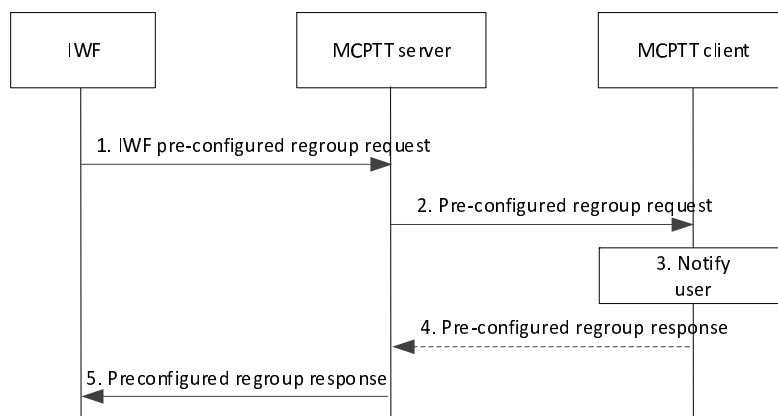
Figure 10.3.8.2.2-1: User regroup procedure using pre-configured group by the IWF
