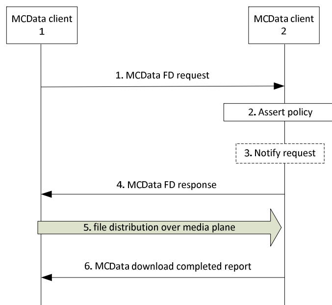
Figure 7.5.3.2-1: One-to-one standalone file distribution using media plane
