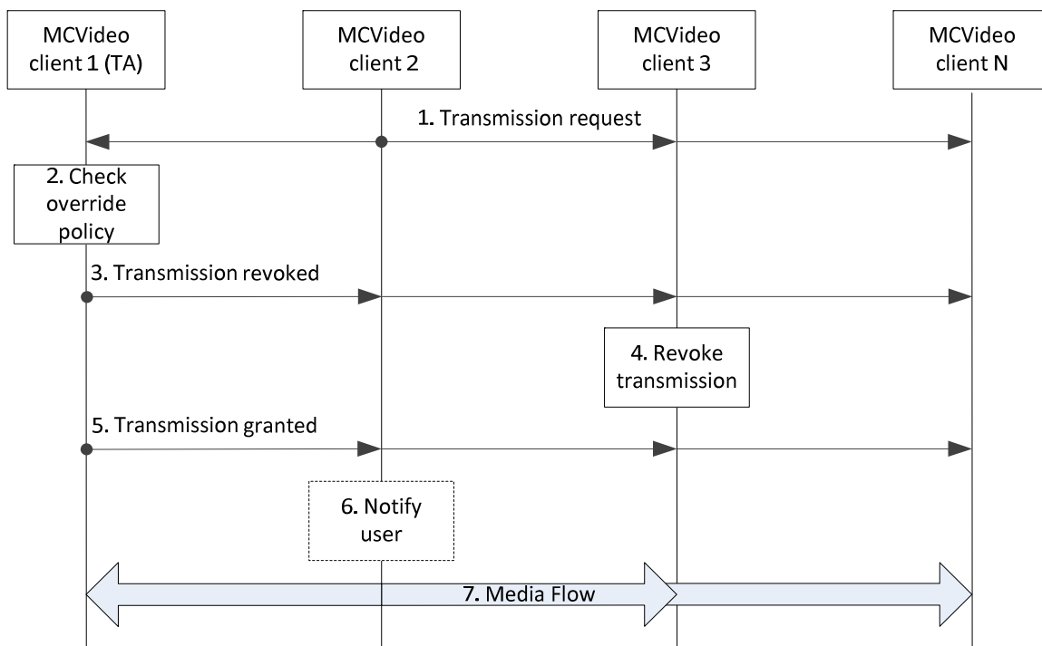
Figure 7.7.2.7-1: Transmission override
