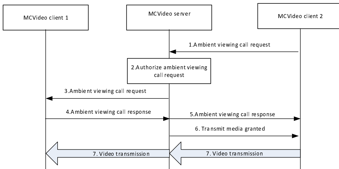
Figure 7.6.3.2-1: Locally initiated ambient viewing call setup
