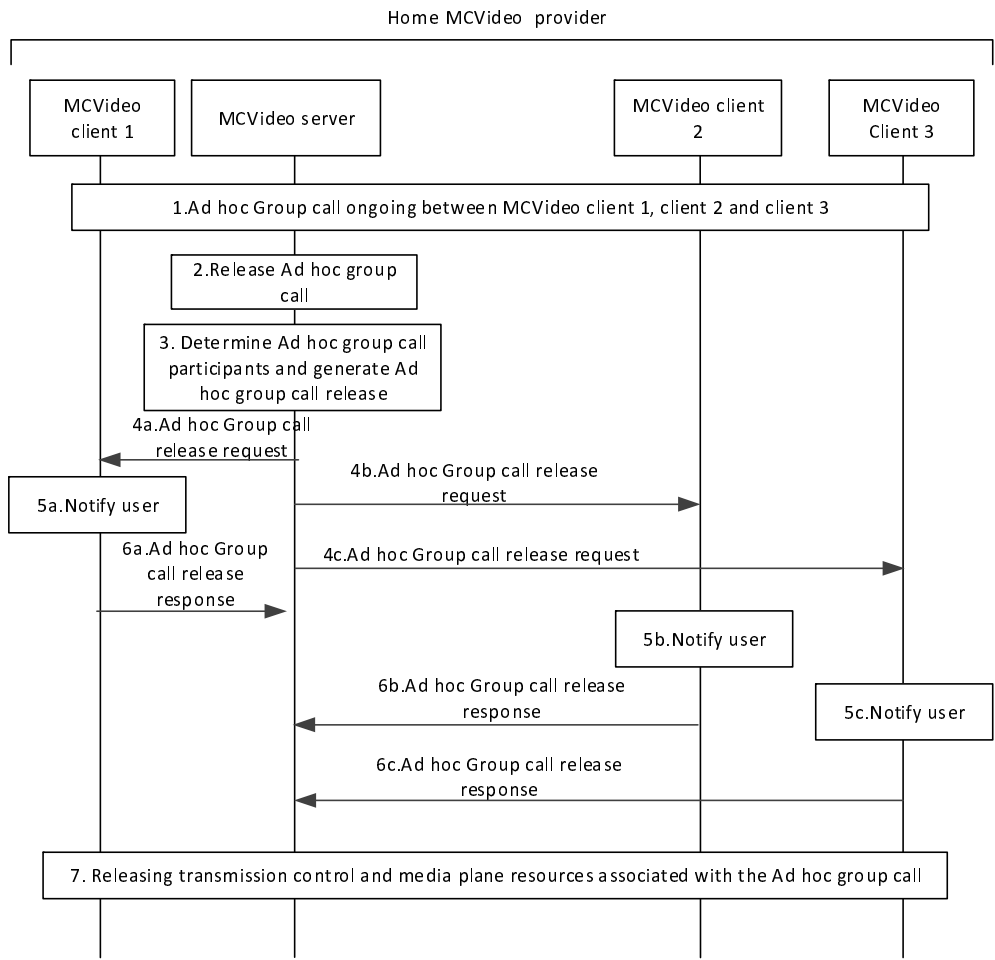
Figure 7.19.3.1.2-1: Release ad hoc group call by the MCVideo server
