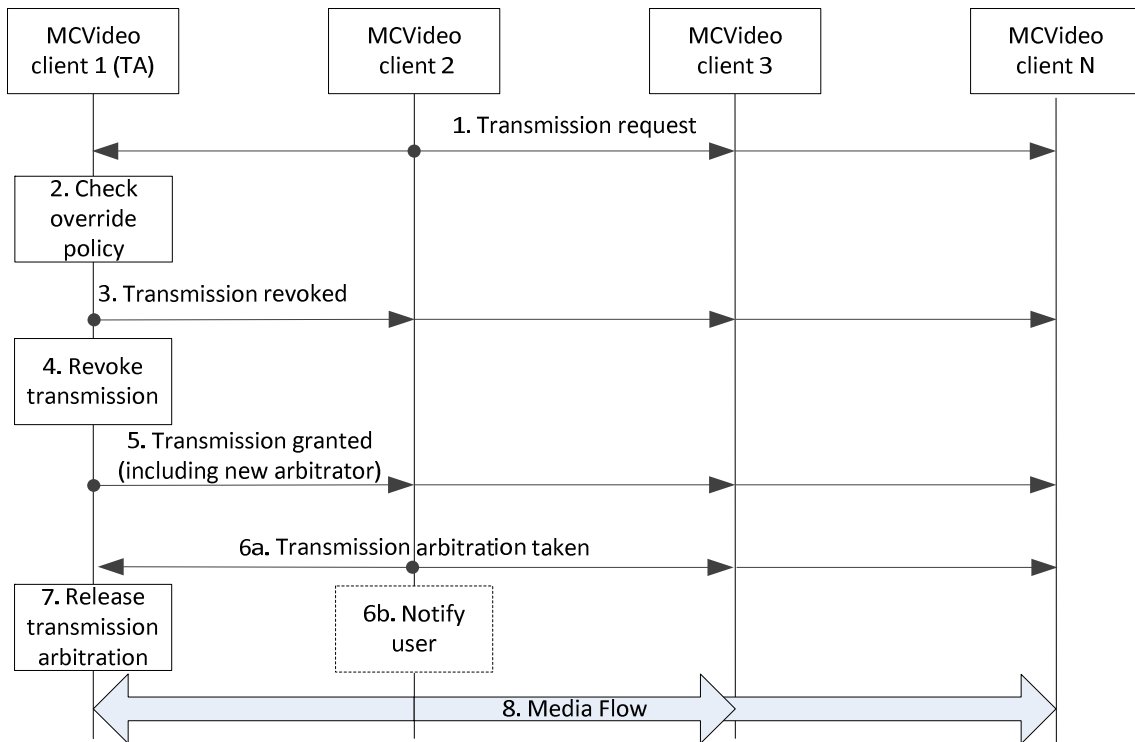
Figure 7.7.2.8-1: Transmission override
