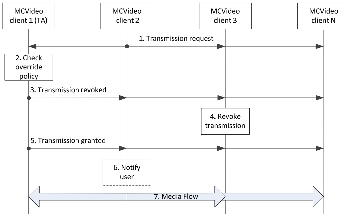
Figure 7.7.2.7-1: Transmission override
