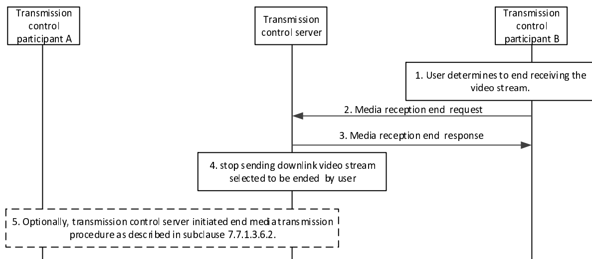
Figure 7.7.1.3.2A-1: End media reception – receiving user initiated
