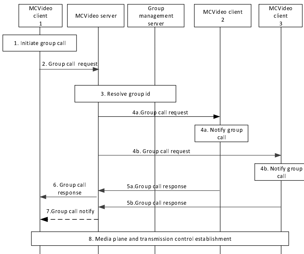
Figure 7.1.2.3.1.1.2-1: Pre-arranged group call setup
