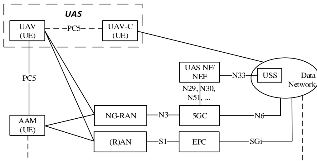
Figure 5.7.1-1: Logical architecture for ground based DAA
