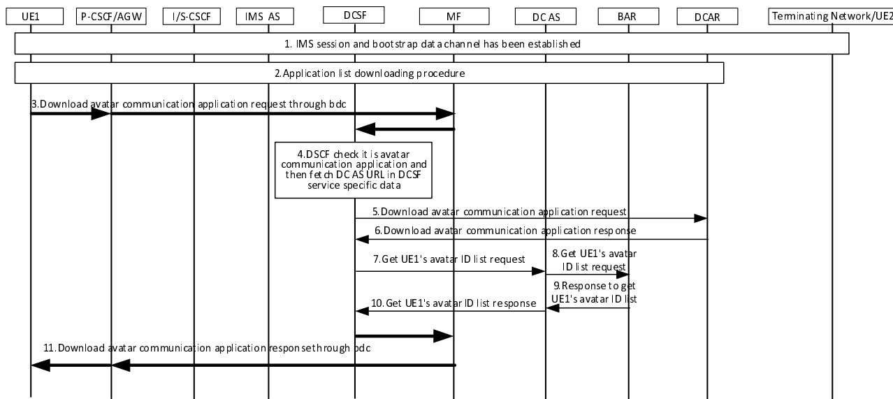
Figure AC.11.3.1-1: Procedures of Avatar ID List Download through Bootstrap Data Channel
