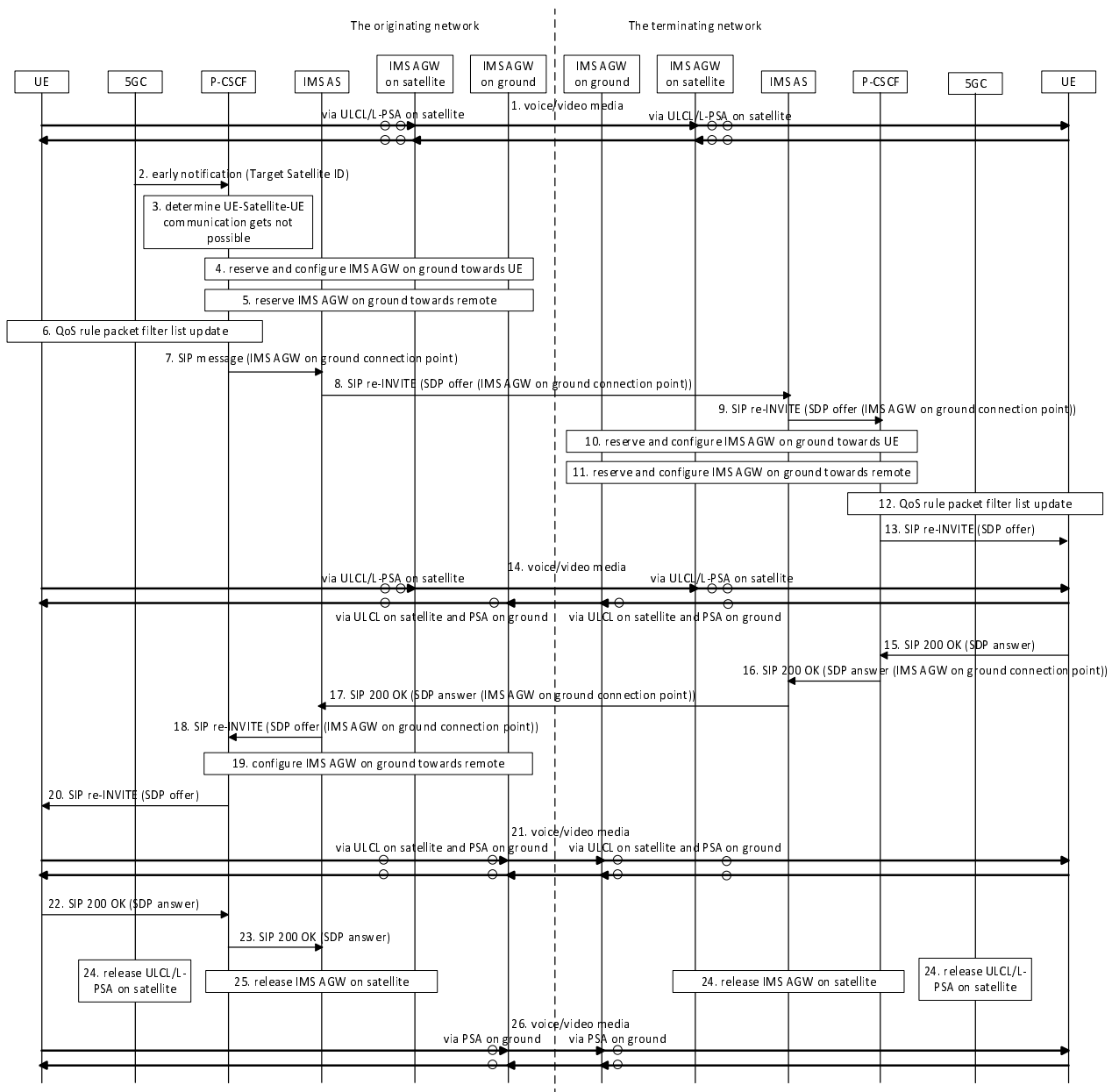
Figure AE.5.2.2-1: Ground fallback procedure
