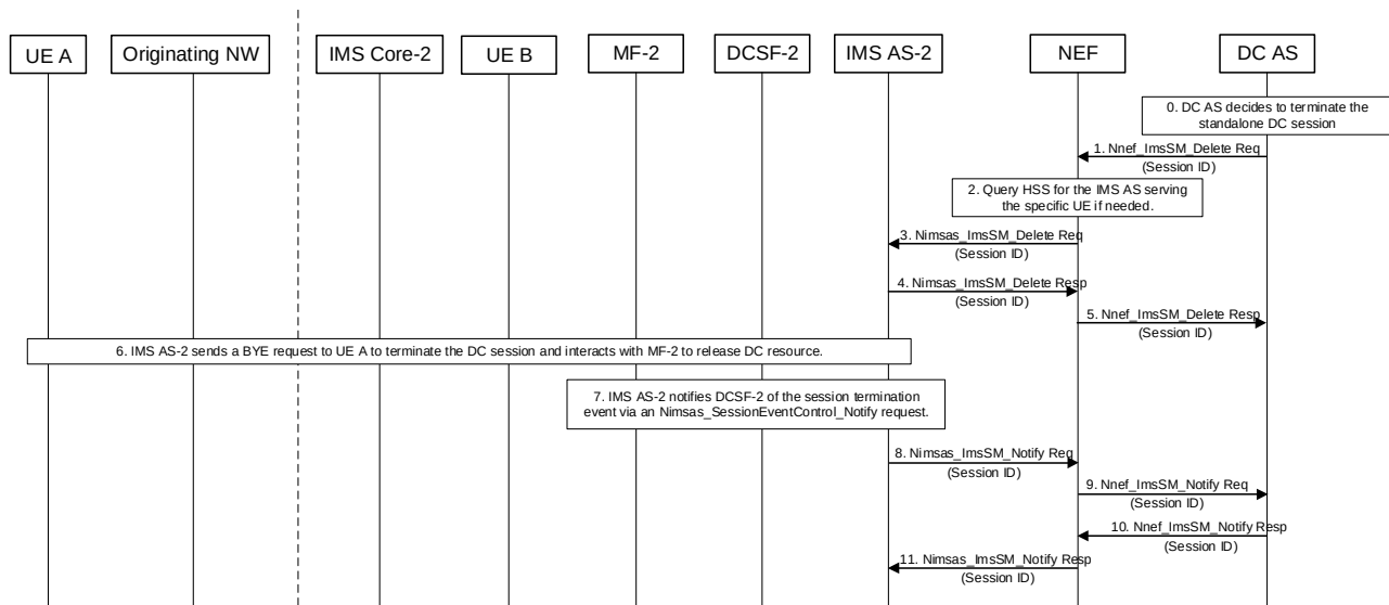
Figure AG.2.3-1: Terminating of a standalone data channel Session
