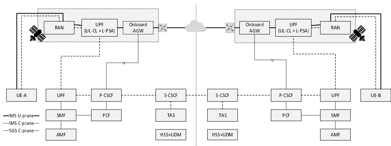
Figure AE.2.1.1-1: Reference architecture of IMS satellite media plane optimization
