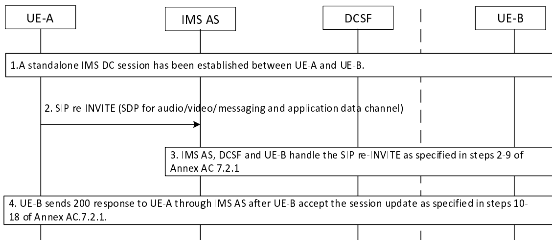
Figure AC.10.2.4-1: Adding MMTel Media to standalone IMS data channel session
