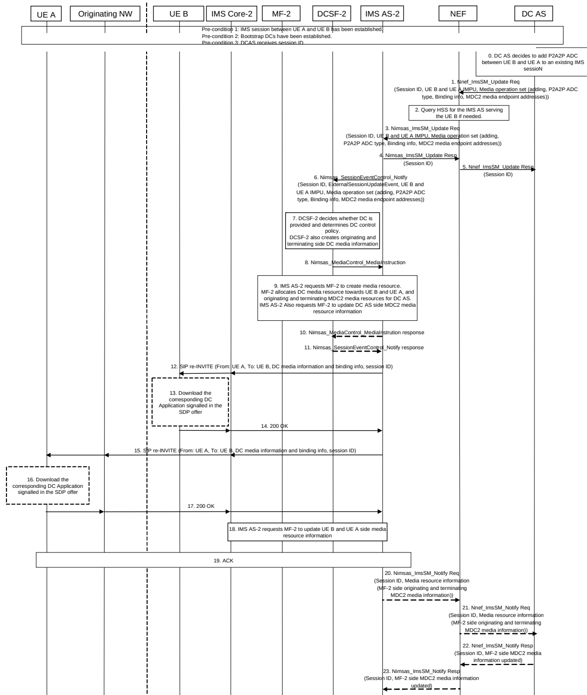
Figure AG.2.1.3-1: Procedure of adding P2A2P data channel(s) to an existing IMS session
