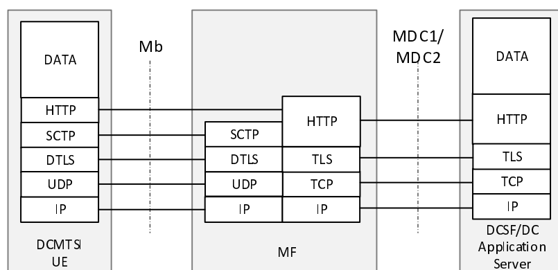
Figure AC.6-1: MF acting as "HTTP Proxy"
