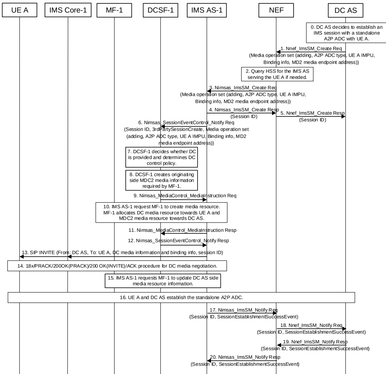
Figure AG.2.2.2-1: Establishment procedure of an IMS session with a standalone A2P application data channel
