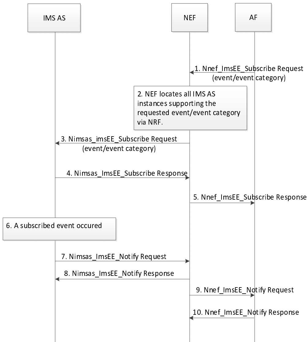
Figure AD.3.3-1: SUBSCRIBE/NOTIFY Procedure for non-subscriber specific IMS events
