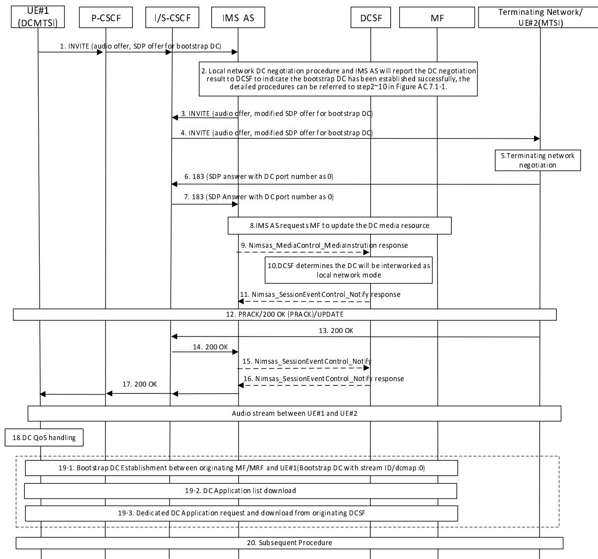
Figure AC.7.9.1-1: Bootstrap Data Channel set up Signalling Procedure for IMS data channel interworking with MTSI UE
