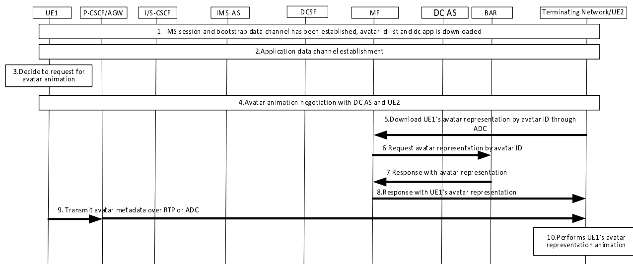
Figure AC.11.3.2.2-1: Procedures of Receiving UE centric IMS Avatar communication
