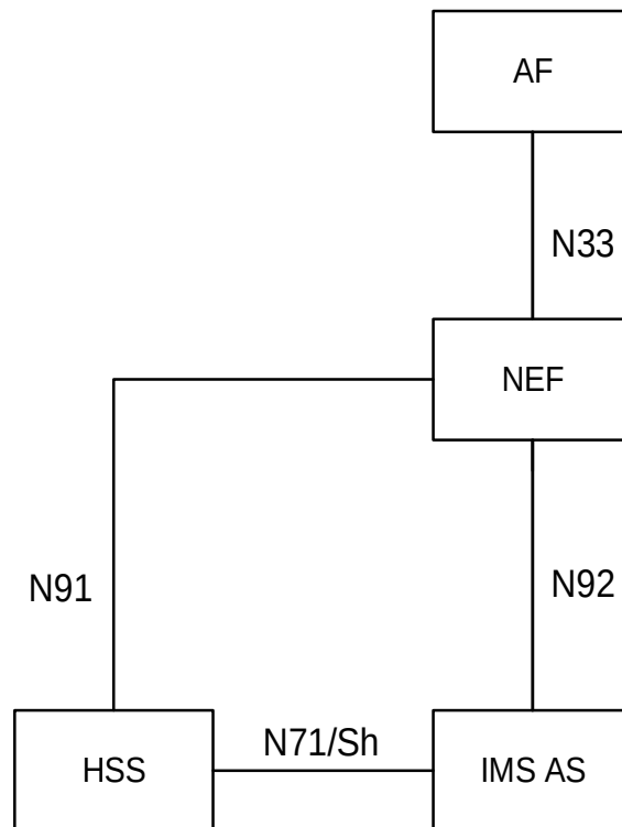
Figure AD.2.1-1: Subscribe/Notify Framework for event monitoring in IMS
