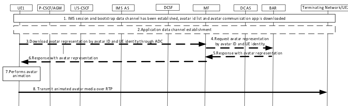
Figure AC.11.3.2.1-1: Procedures of Sending UE centric IMS Avatar communication
