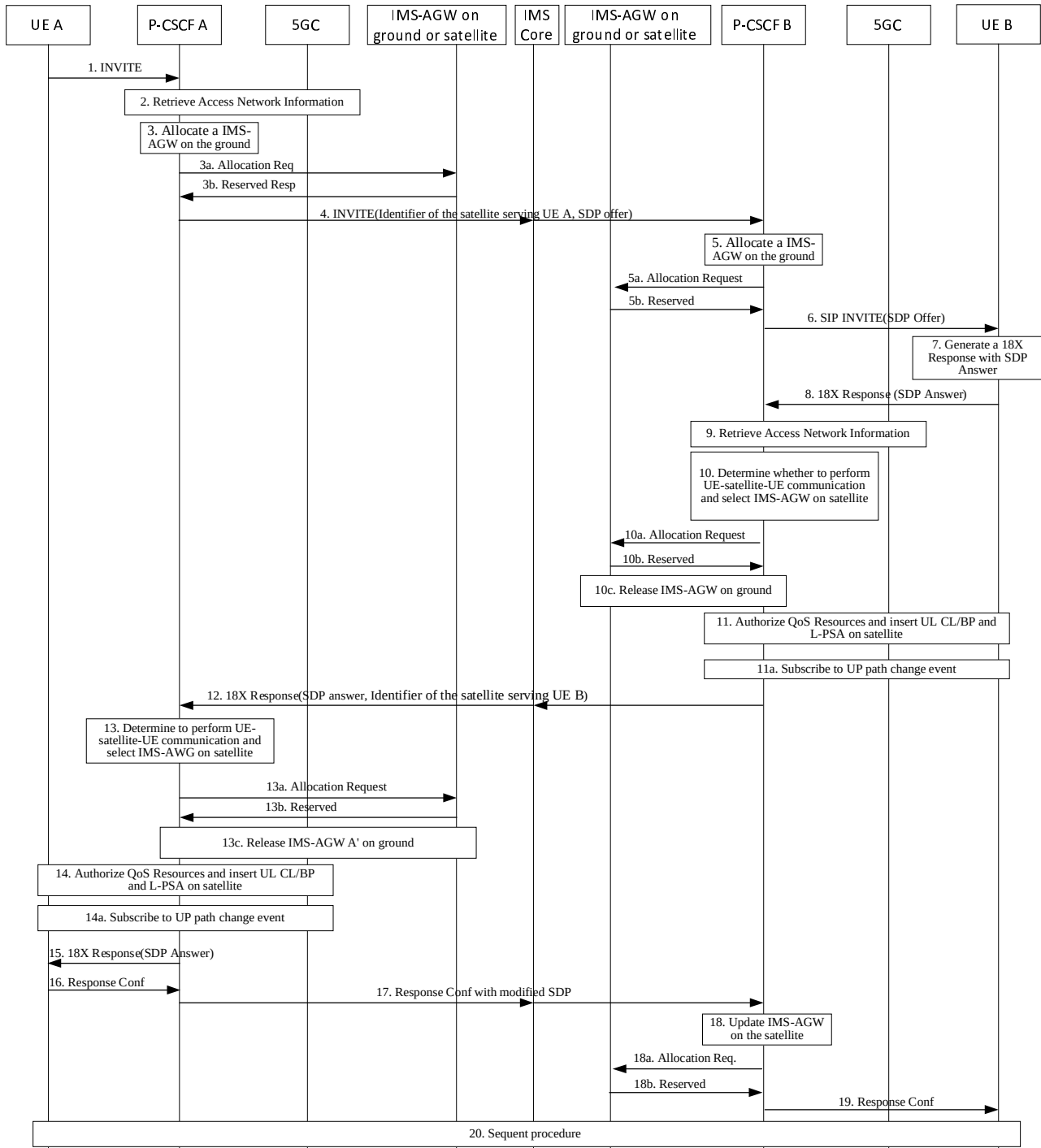
Figure AE.5.1-1: Session establishment procedure with activation of optimizing media routing
