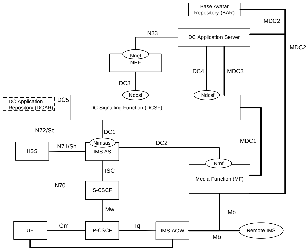
Figure AC.11.2-1: Architecture to support Avatar communication
