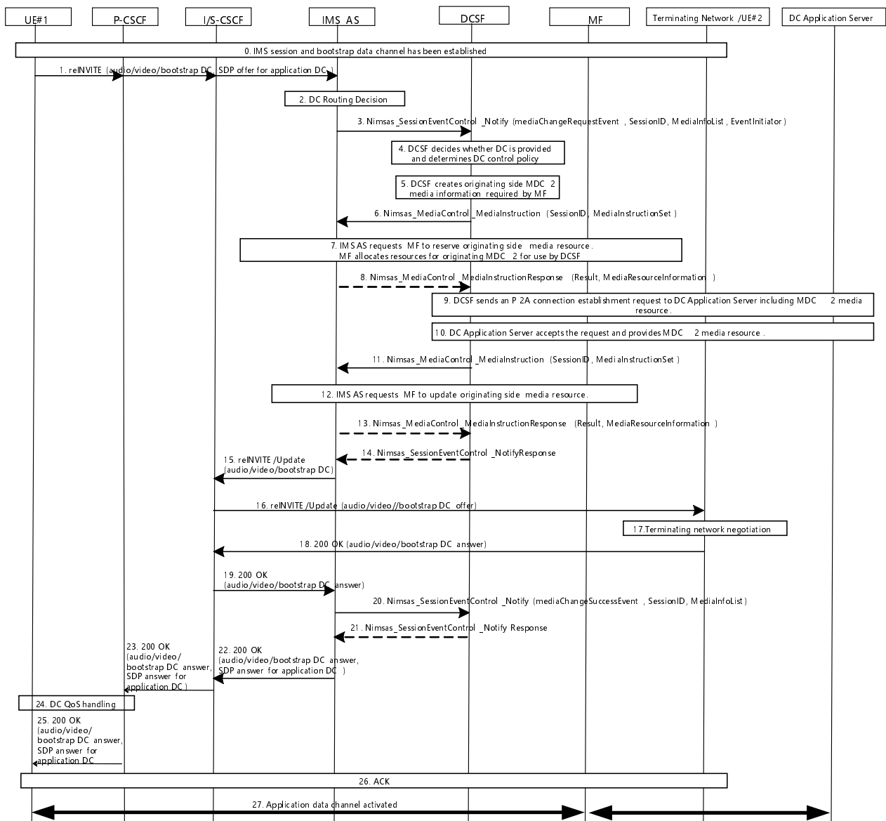
Figure AC.7.2.2-1: Person-to-Application (P2A) Application Data Channel set up Signalling Procedure
