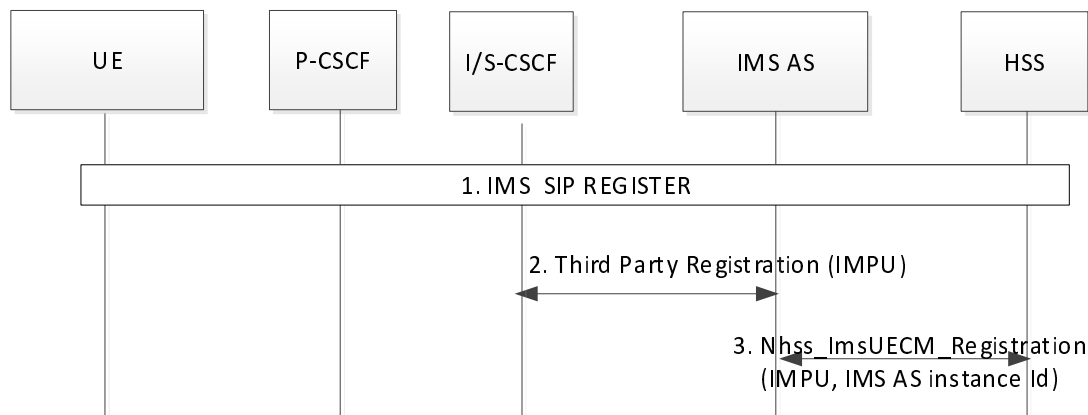
Figure AD.3.1-1: IMS AS Instance Registration in HSS
