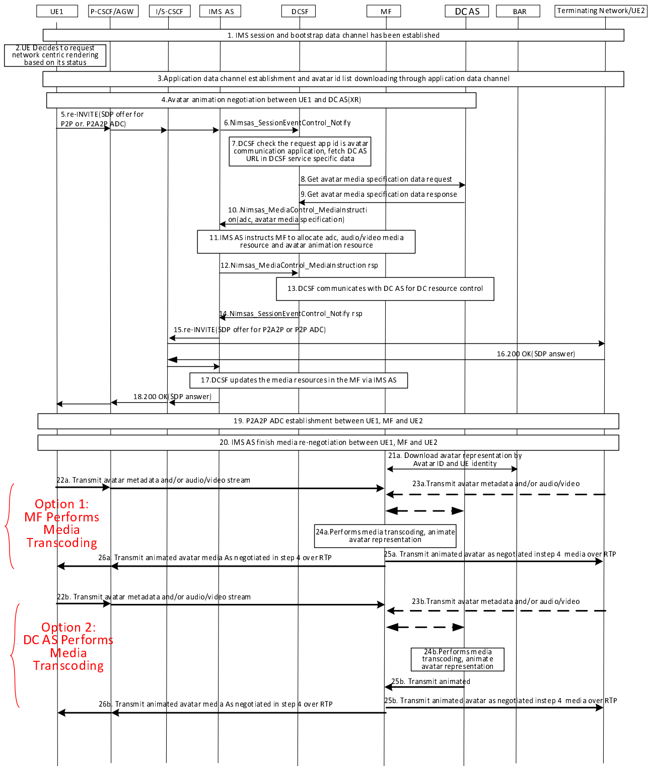
Figure AC.11.3.3-1: Procedures of network centric IMS Avatar communication
