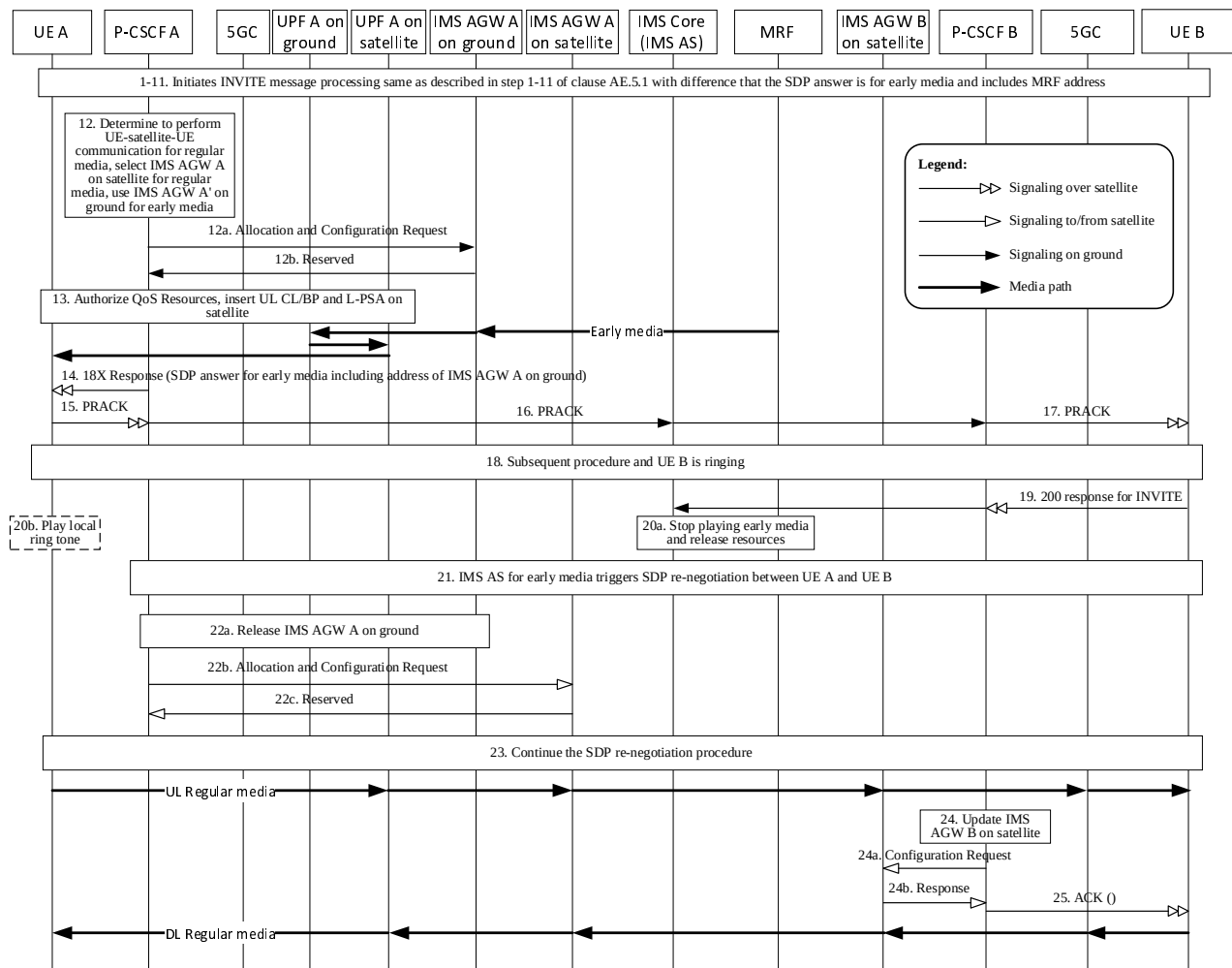
Figure AE.5.3-1: IMS session establishment procedure with early media
