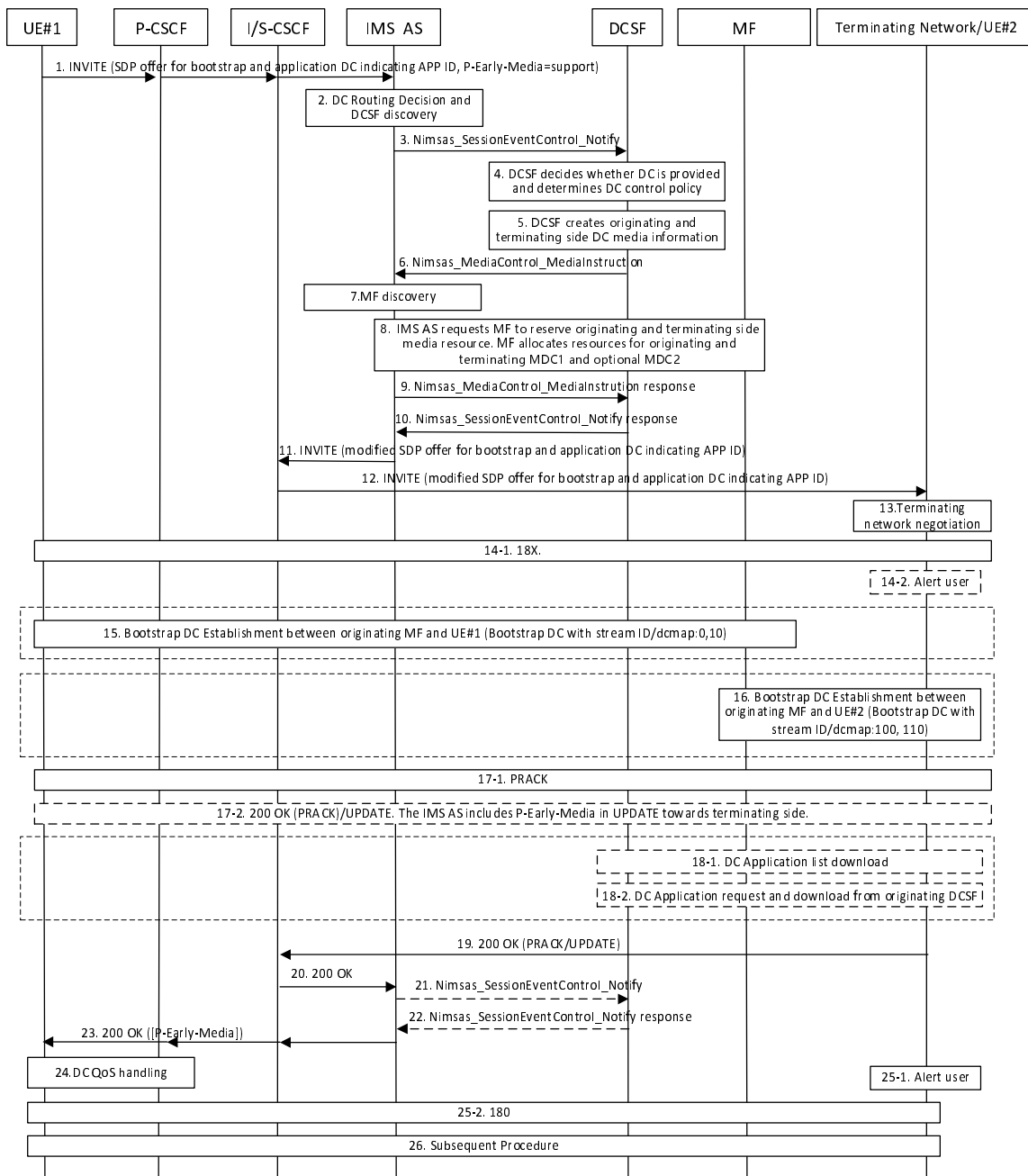
Figure AC.10.2.3-1: Originating Standalone IMS DC Session if Application Available in Originating UE
