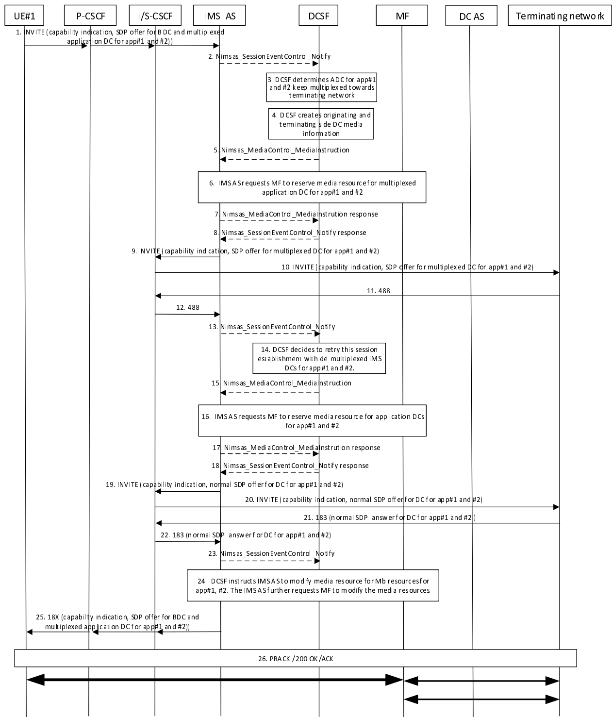
Figure AC.7.10.4.2.3-1: Application data channel multiplexing when terminating network rejects standalone IMS DC session
