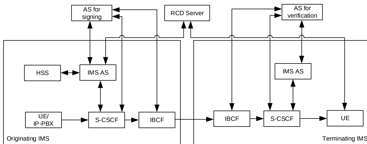
Figure AF.2.1-1: System architecture to support authorization, signing and verification of third party user identity information in IMS
