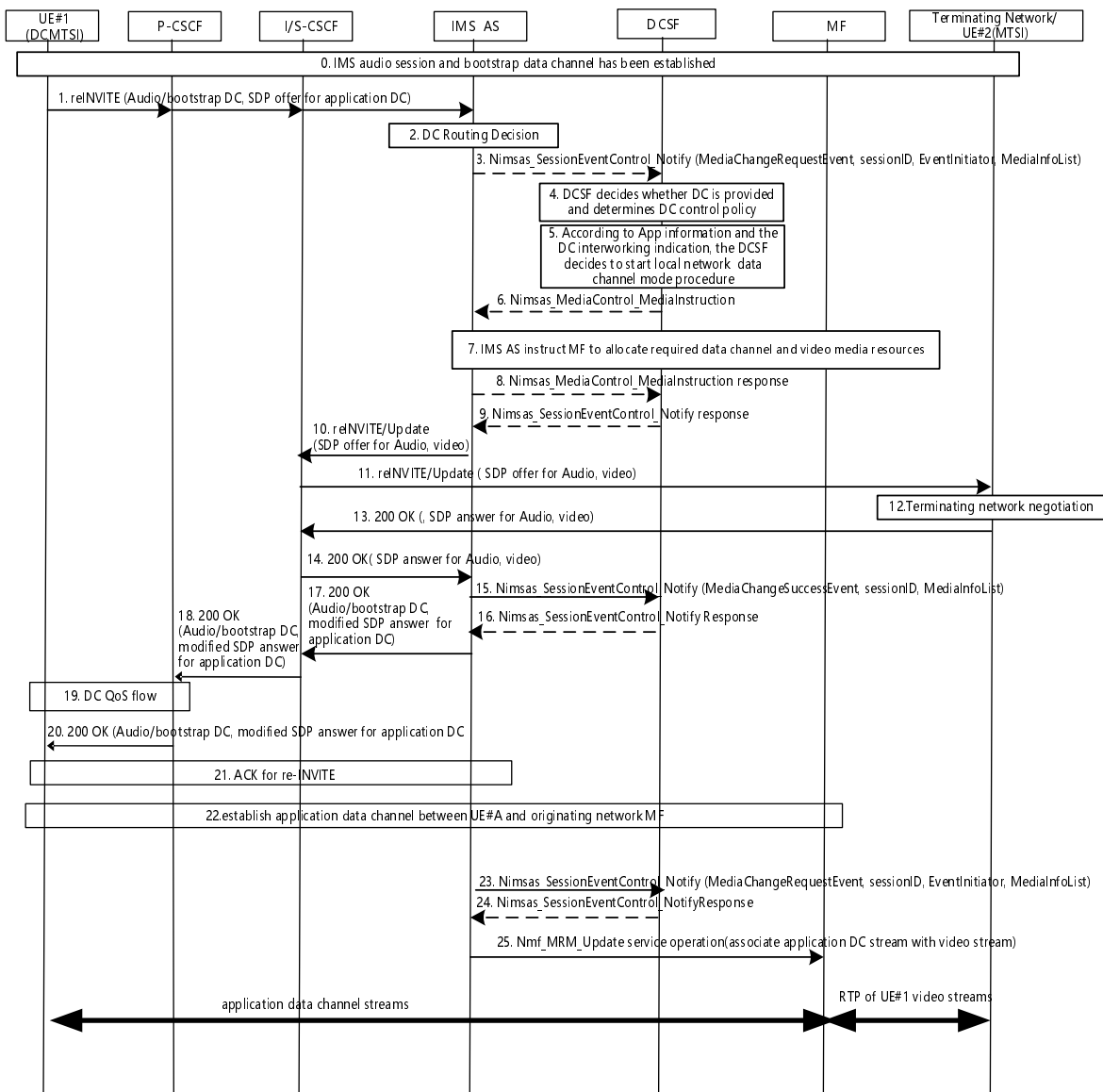
Figure AC.7.9.2-1: Application Data Channel set up signalling procedure for IMS data channel interworking with MTSI UE via MF
