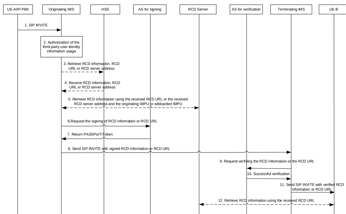
Figure AF.3-1: Procedure for signing and verification of third party user identity information in IMS
