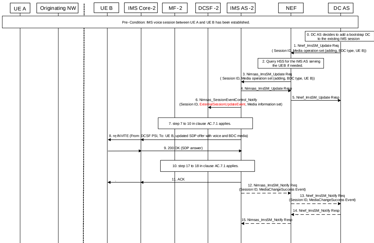
Figure AG.2.1.4-1: Procedure of adding bootstrap data channel to an existing IMS session
