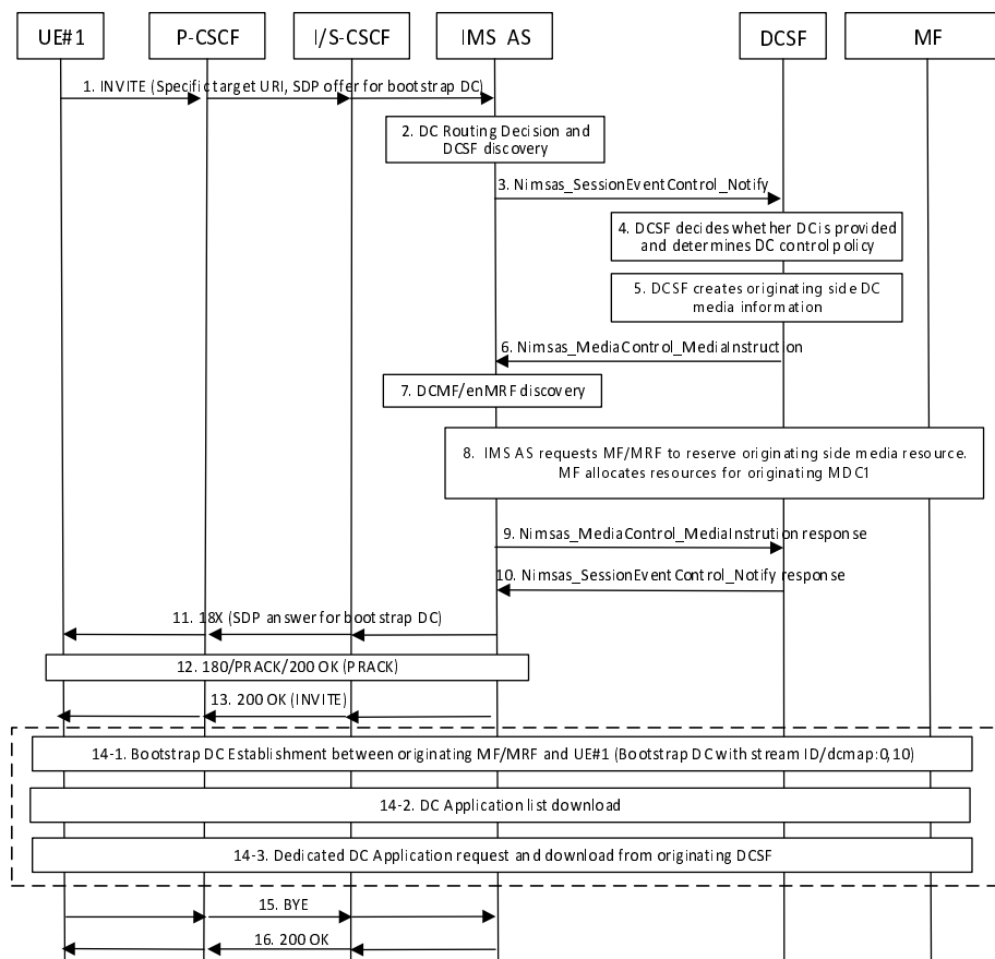
AC.10.2.1-1: Originating Standalone Bootstrap DC Setup using PSI
