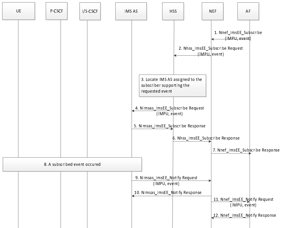
Figure AD.3.2-1: SUBSCRIBE/NOTIFY Procedure for Subscriber specific IMS events
