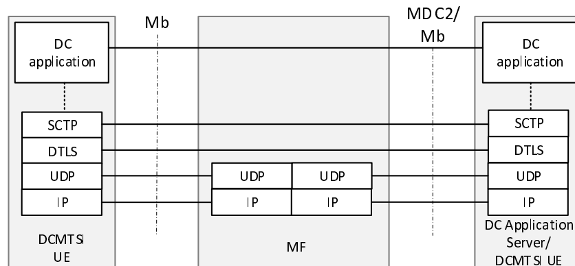
Figure AC.6-2: MF acting as "UDP Proxy"
