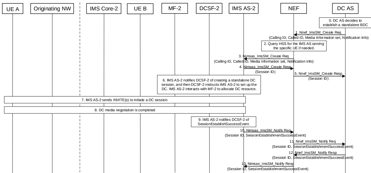
Figure AG.2.2.1-1: Establishment procedure of a standalone BDC session
