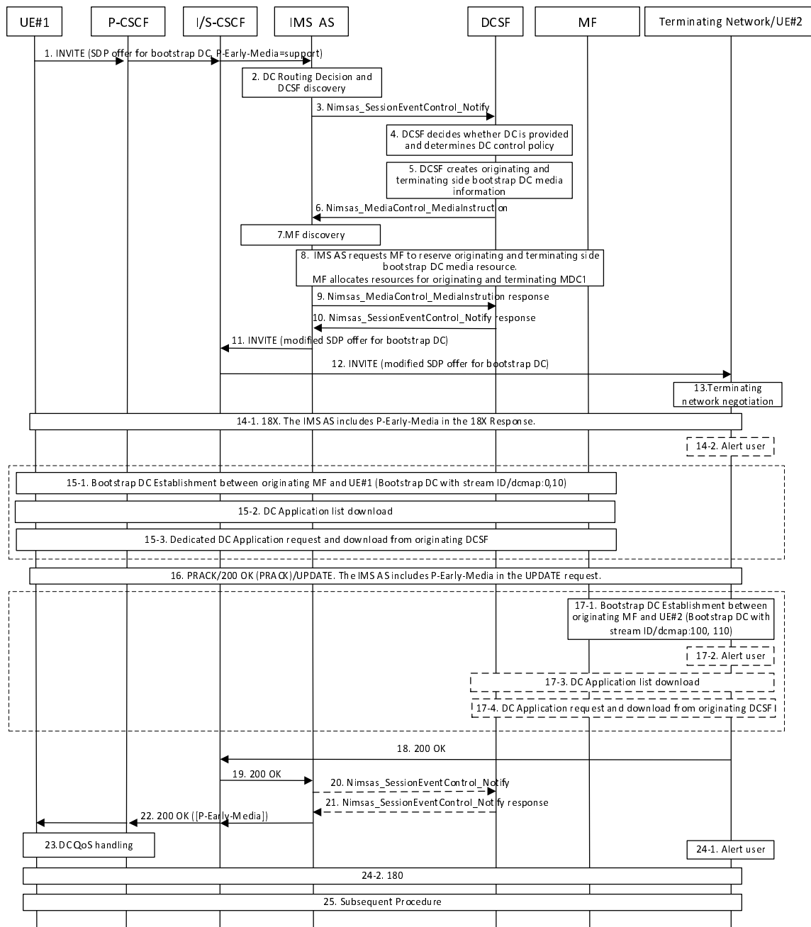
Figure AC.10.2.2-1: Originating Standalone IMS DC Session if Application not Available in Originating UE
