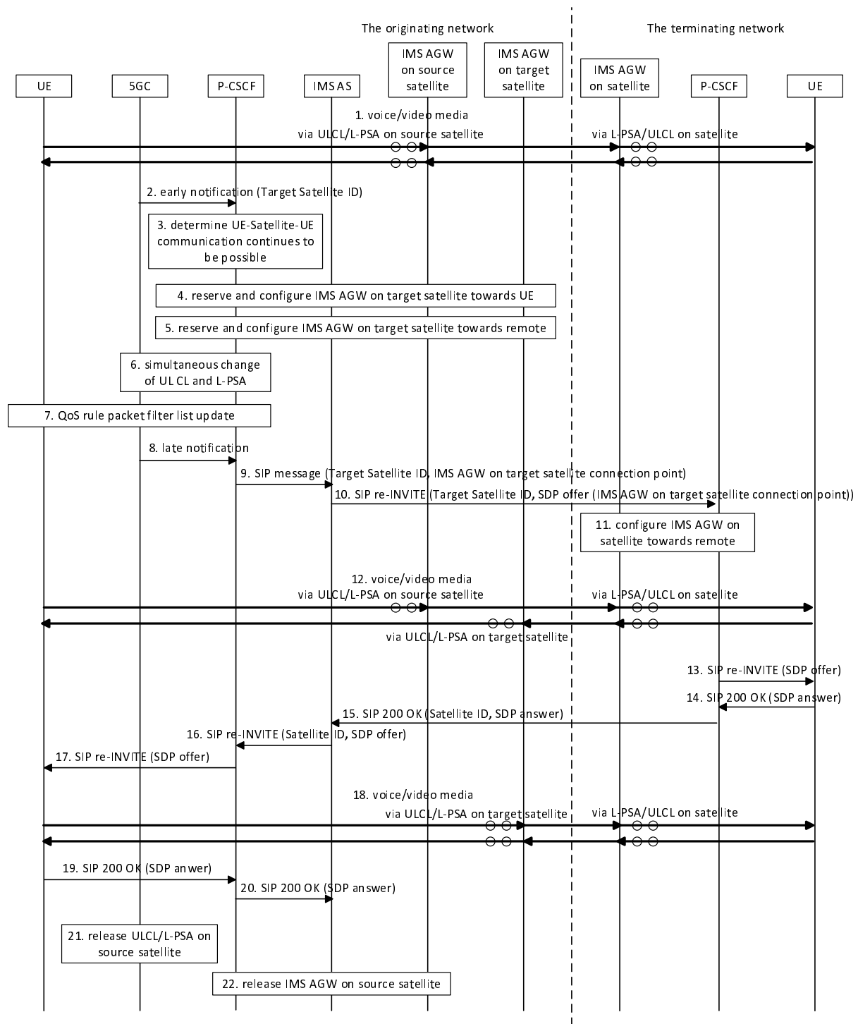
Figure AE.5.2.1-1: Continued optimized media routing procedure
