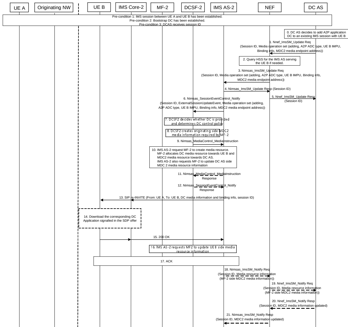
Figure AG.2.1.1-1: Procedure of adding A2P application data channel(s) to an existing IMS session
