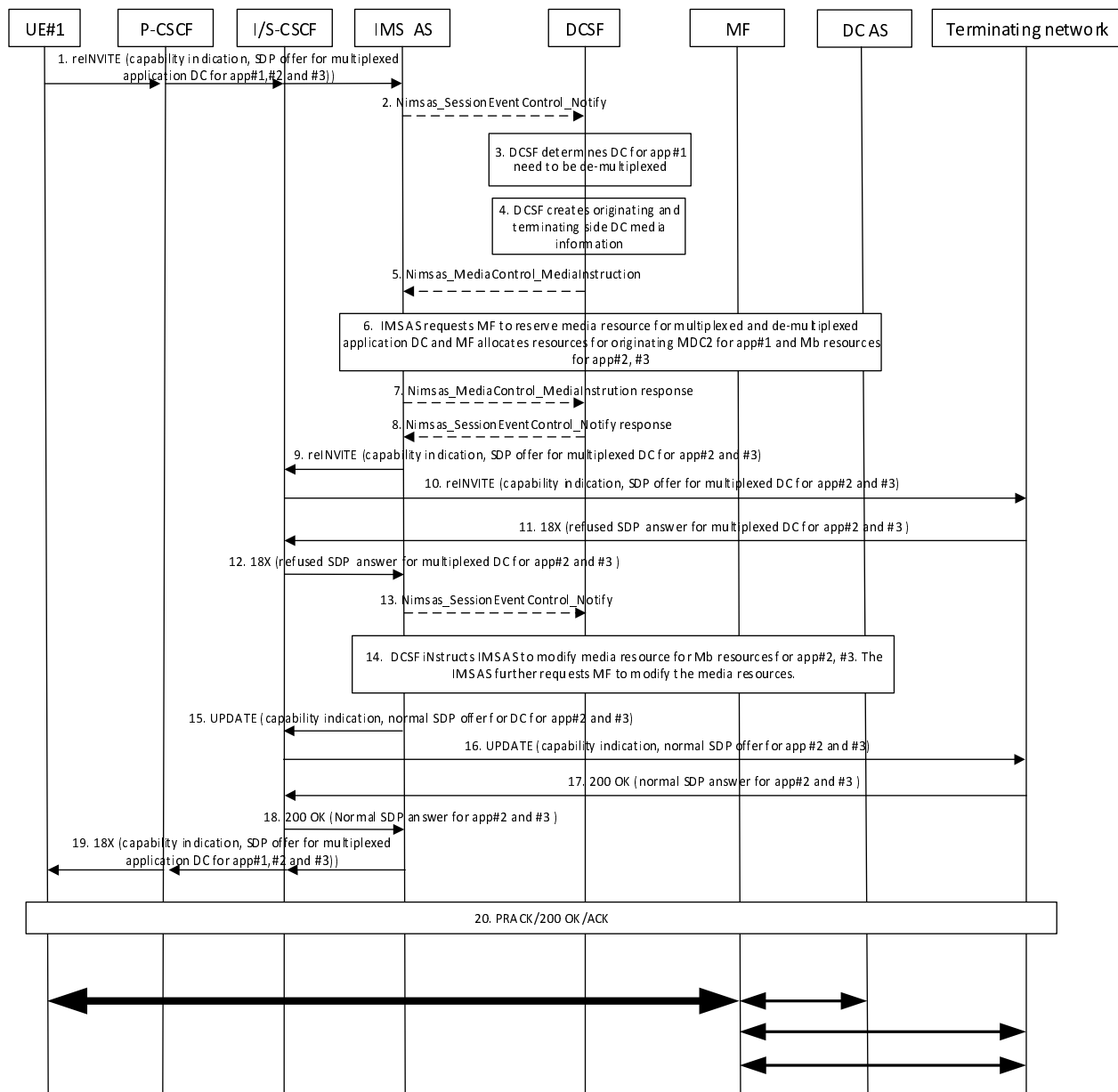
Figure AC.7.10.4.2.2a-1: Application data channel multiplexing when terminating network does not support data channel multiplexing
