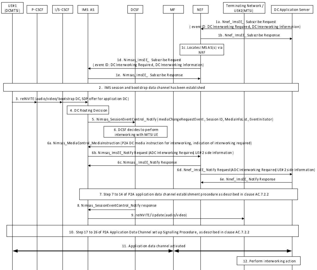
Figure AC.7.9.3-1: Application Data Channel set up signalling procedure for IMS data channel interworking with MTSI UE via DC application server
