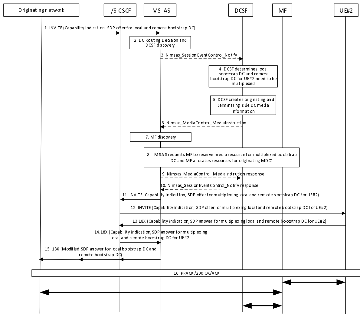
Figure AC.7.10.4.1.2-1: Multiplexing bootstrap data channels in terminating network
