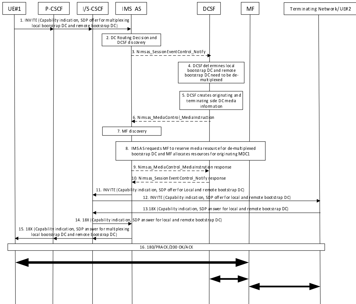
Figure AC.7.10.4.1.1-1: Multiplexing bootstrap data channels in originating network
