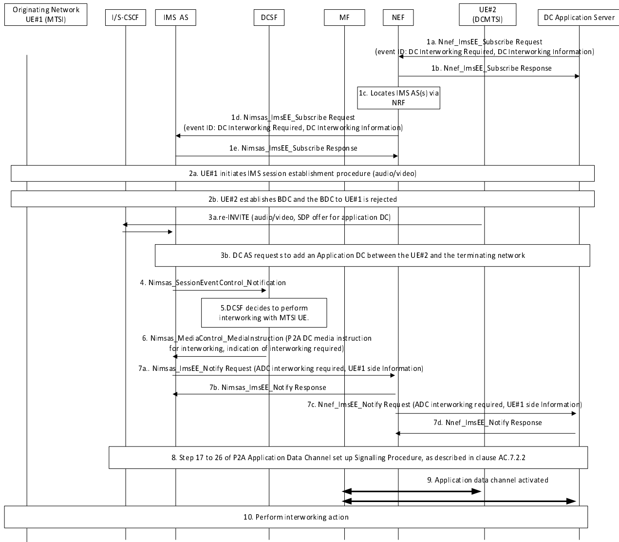
Figure AC.7.9.4-1: Application Data Channel set up signalling procedure for IMS data channel interworking with originating MTSI UE via DC application server
