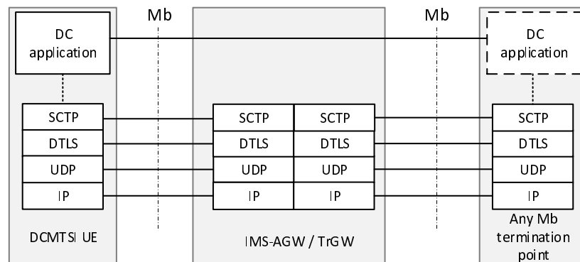
Figure AC.6-4: IMS-AGW / TrGW acting as "DC Application Proxy"
