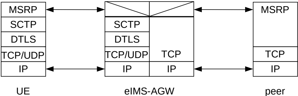
Figure U.1.5.1-2: Protocol architecture for MSRP acting as transport relay function
