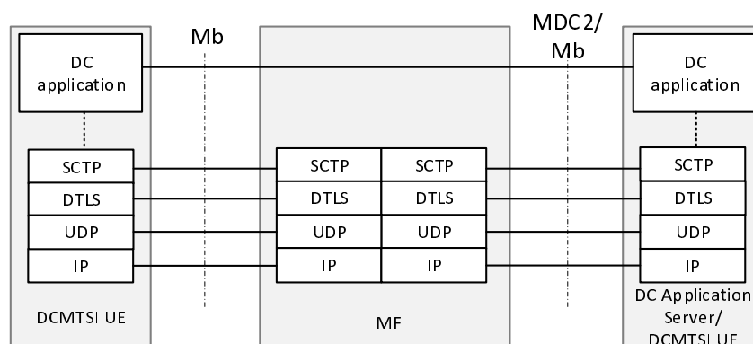
Figure AC.6-3: MF acting as "DC Application Proxy"
