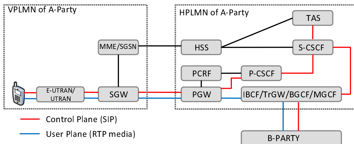
Figure W.2-1: architecture IMS architecture
