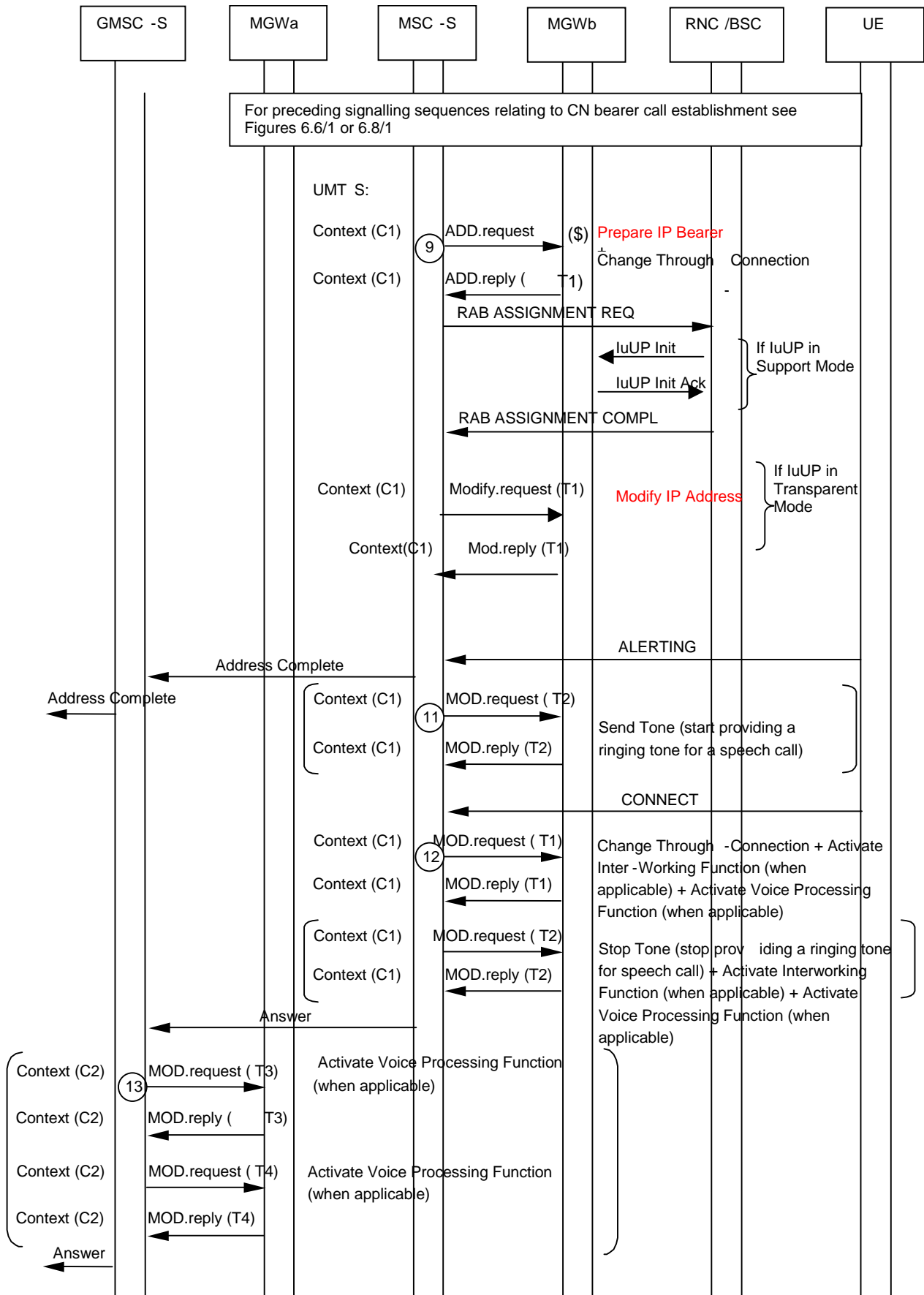
Figure 6.2.3/1 Terminating Call Establishment For lu Interface on IP
