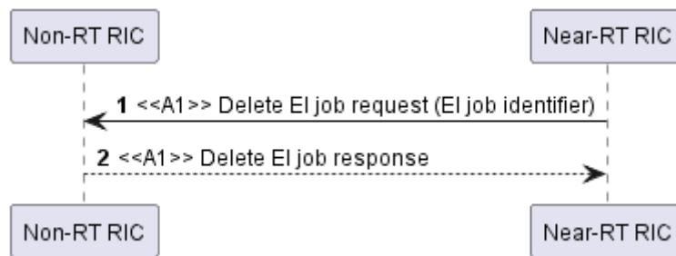
Figure 7.6.3.3-1: Delete EI job
