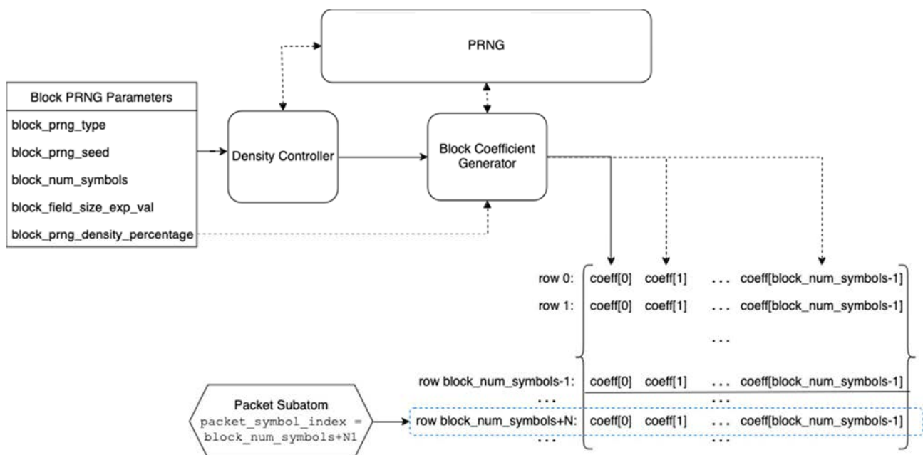
Figure 14: Block PRNG
