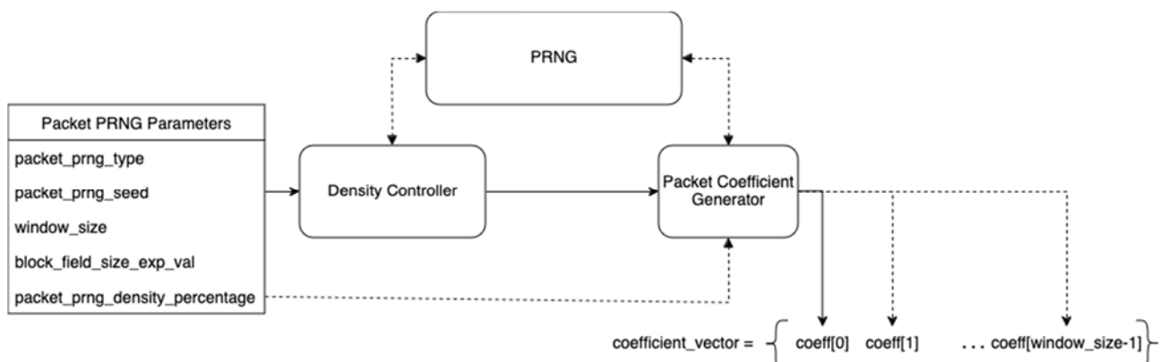
Figure 15: Packet PRNG
