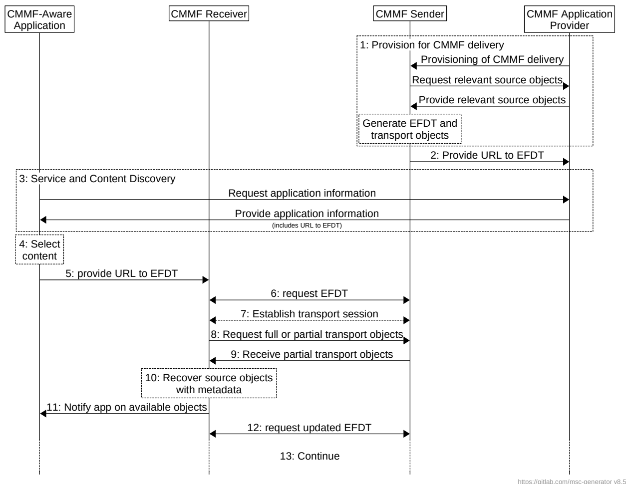
Figure D.1: High-level procedure for CMMF delivery using FDT-based CDP
