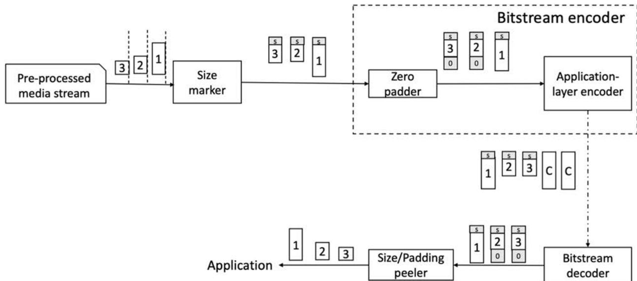
Figure 16: Handling variable size data
