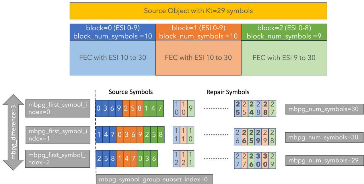
Figure 12: Example symbol arrangement for mbpg_symbol_arrangement=0010b (Source-Symbol Interleaved Arrangement)
